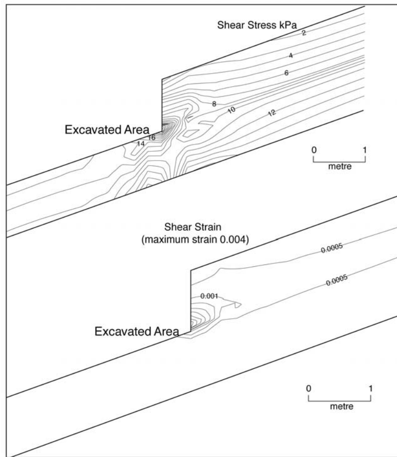
Figure 8 Distribution of shear stress and strain for a 1 m-high headcut in loess-derived materials. From Collison and Simon (2001).
