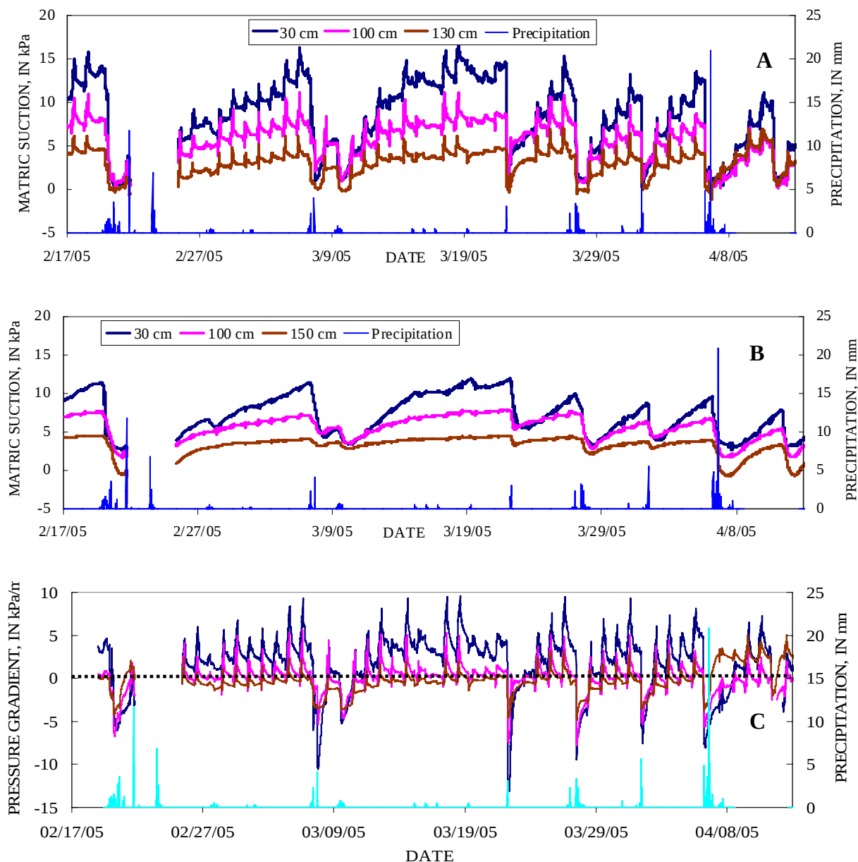
Figure 5 Data for the edge-center (A) and front-center (B) tensiometers nests, and pressure gradient between the front and edge nests (C) at three depths, all with associated rainfall.
