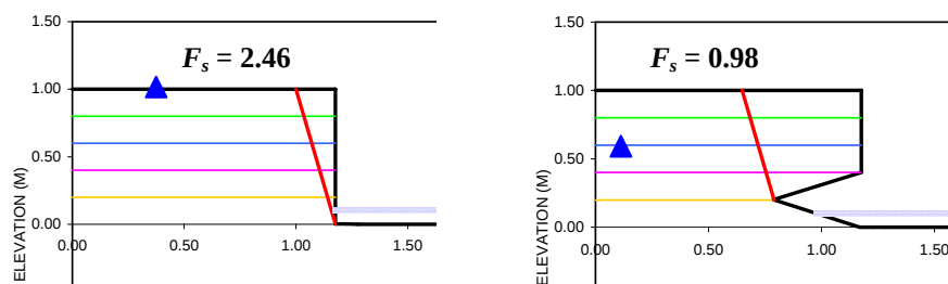
Figure 4 Bank-stability analysis of gully headwall showing destabilization by undercutting and partial saturation. F_s = factor of safety; blue triangles represent height of the phreatic surface.
