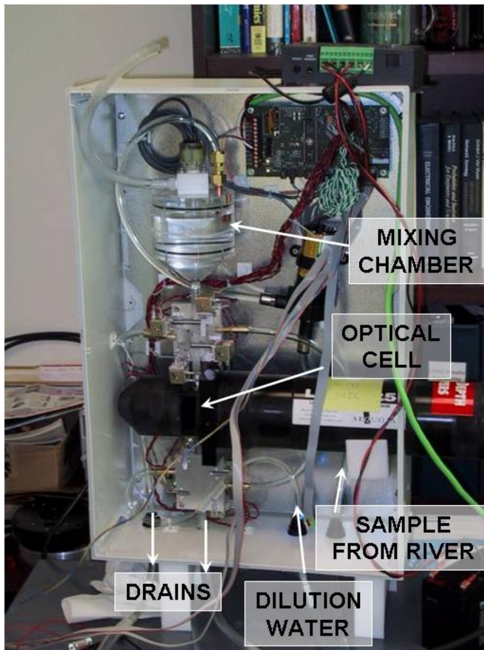
Figure 2 LISST-Infinite. Photo credit: Chuck Pottsmith.
