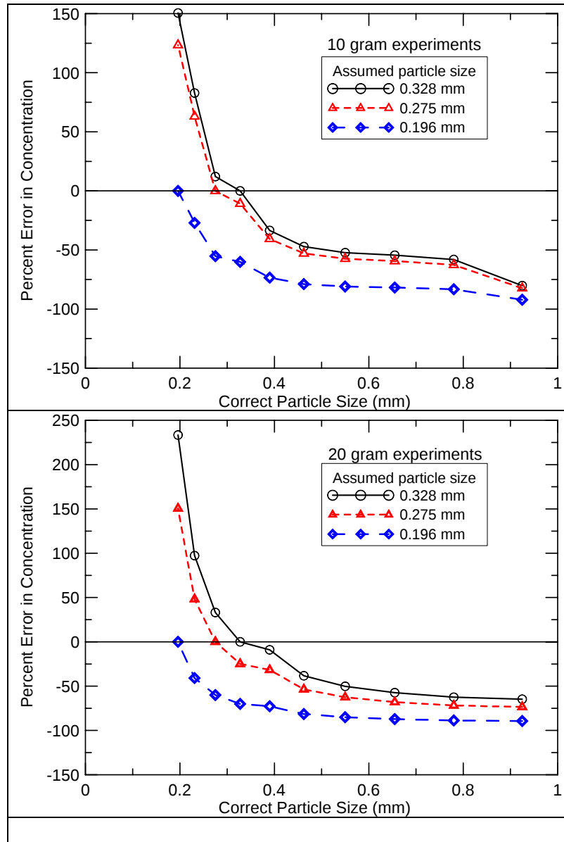
Figure 1 Errors in concentration due to incorrect grain size calculated using acoustic backscattering data from jet tank.
