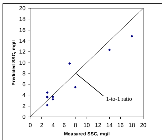
Figure 3 Measured versus predicted suspended sediment concentrations for the St. Joe River near Chatcolet, Idaho (12415140).
