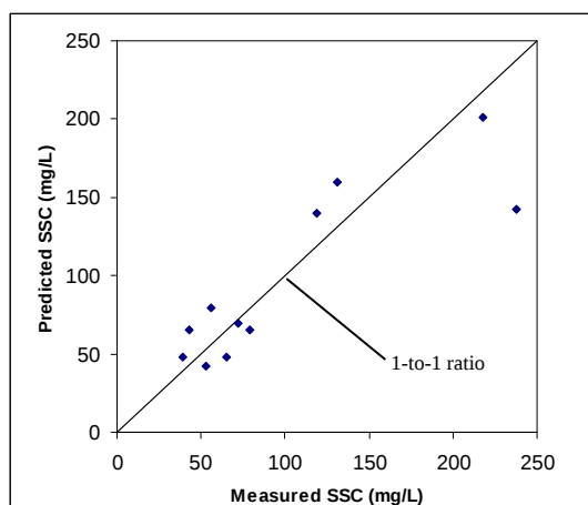
Figure 4 Measured versus predicted suspended sediment concentrations for the Boise River near Parma, Idaho (13213000).
