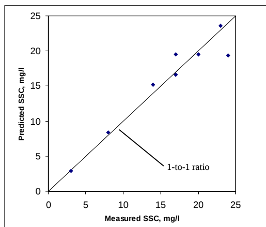
Figure 1 Measured versus predicted suspended sediment concentrations for the Kootenai River at Tribal Hatchery near Bonners Ferry, Idaho (12310100).
