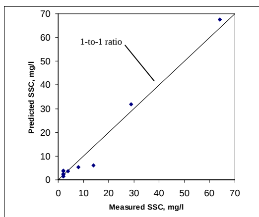
Figure 2 Measured versus predicted suspended sediment concentrations for the Coeur d'Alene River near Harrison, Idaho (12413860).
