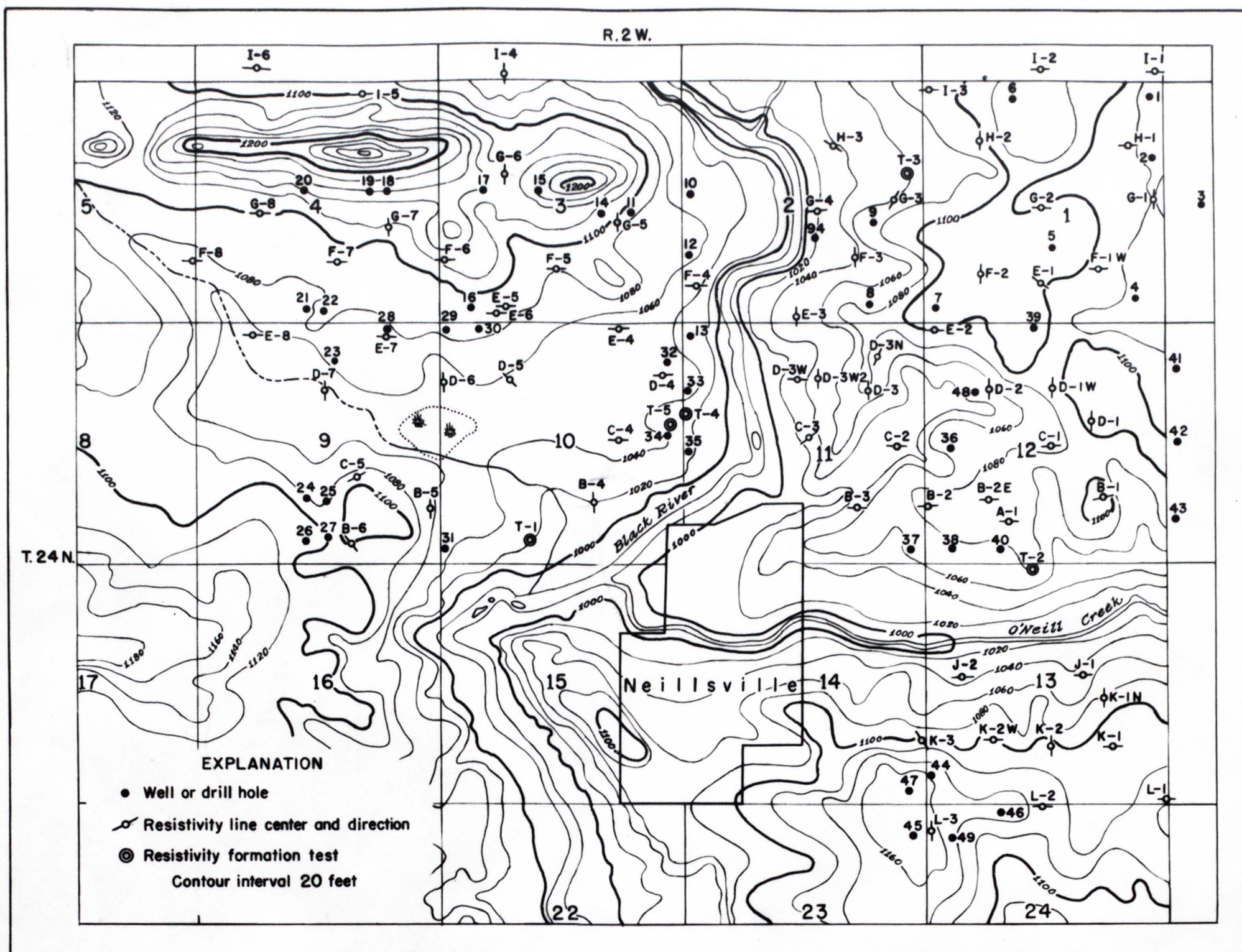
Figure 1. — Map of the Neillsville, Wisconsin area showing surface contours, resistivity line centers and directions, and locations of drilling information.
