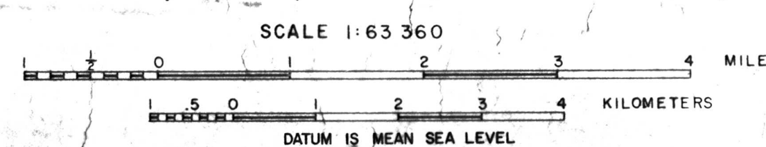
STRUCTURAL CONTOUR MAP ON HEART RIVER (E) COAL BED DICKINSON AREA, BILLINGS, DUNN, AND STARK COUNTIES, NORTH DAKOTA
