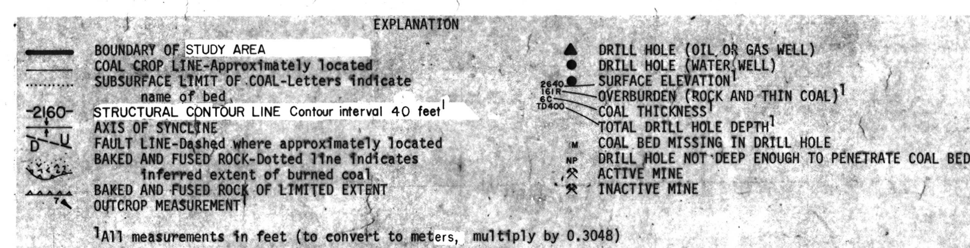
STRUCTURAL CONTOUR MAP ON HEART RIVER (E) COAL BED DICKINSON AREA, BILLINGS, DUNN, AND STARK COUNTIES, NORTH DAKOTA
