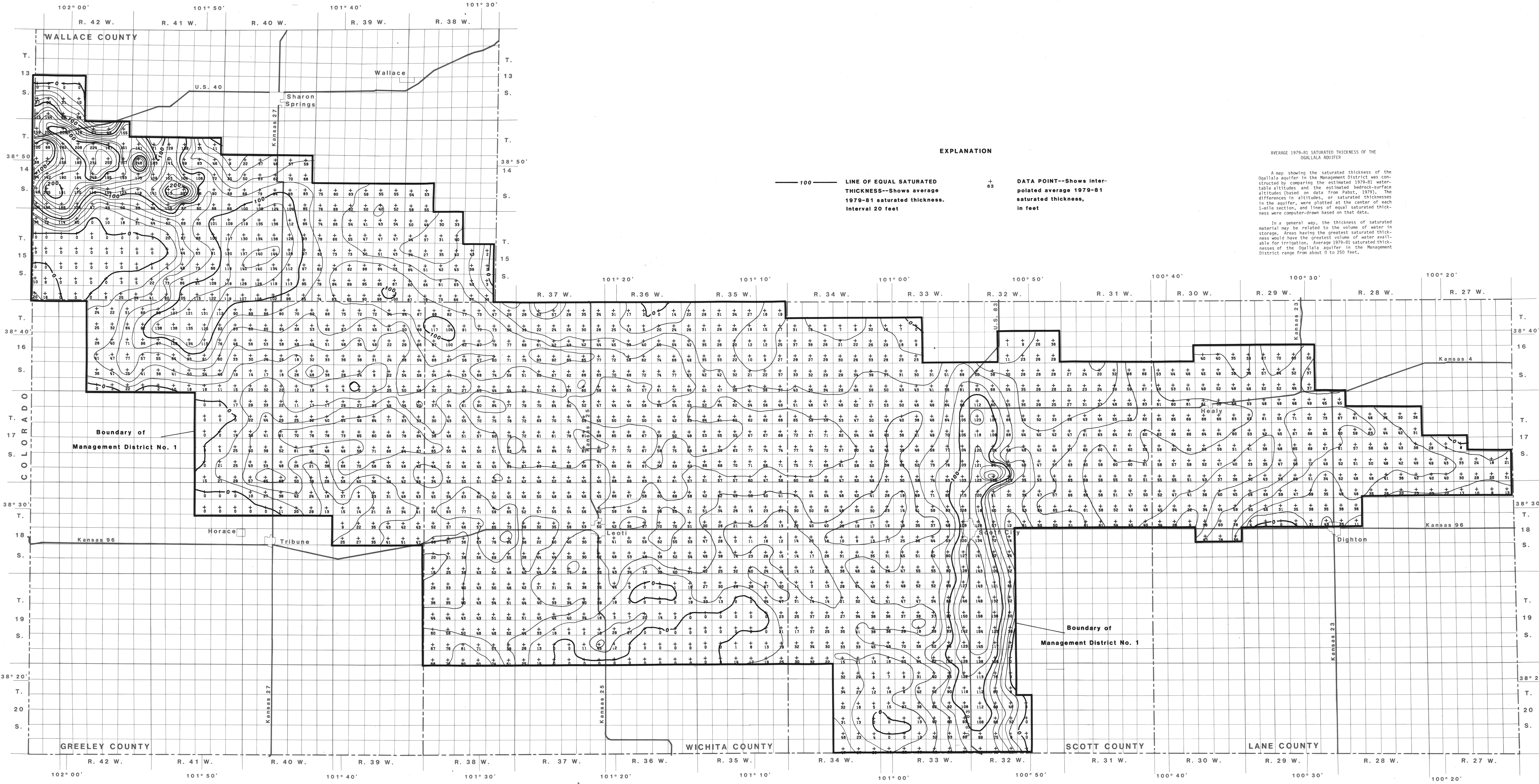
AVERAGE 1979-81 SATURATED THICKNESS OF THE OGALLALA AQUIFER HYDROLOGIC MAPS OF OGALLALA AQUIFER, WEST-CENTRAL KANSAS, 1979-81
