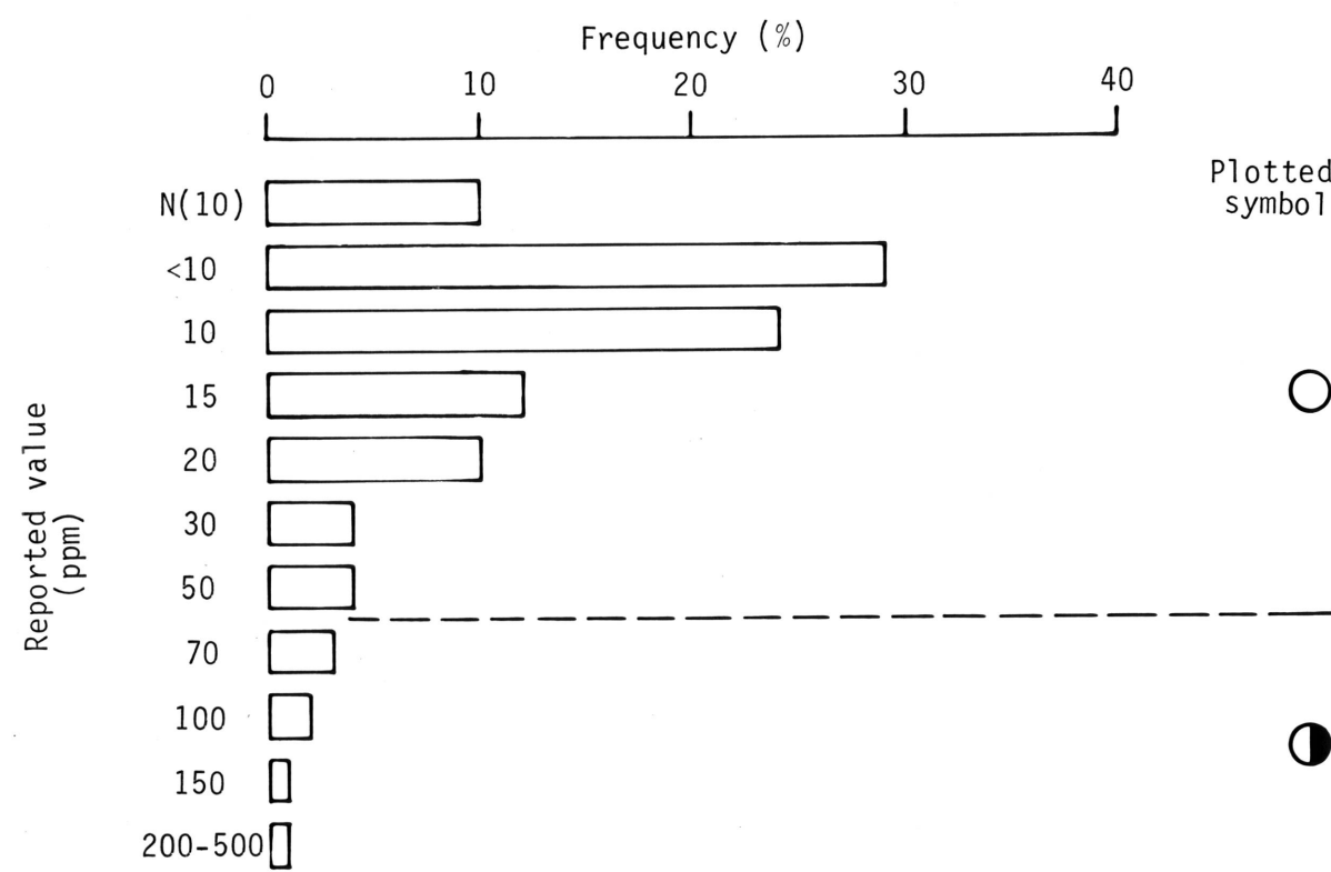
Figure 2.--Frequency diagram for copper in samples of nonmagnetic heavy-mineral concentrate. [N = Not detected at the lower limit of determination shown in parentheses]
