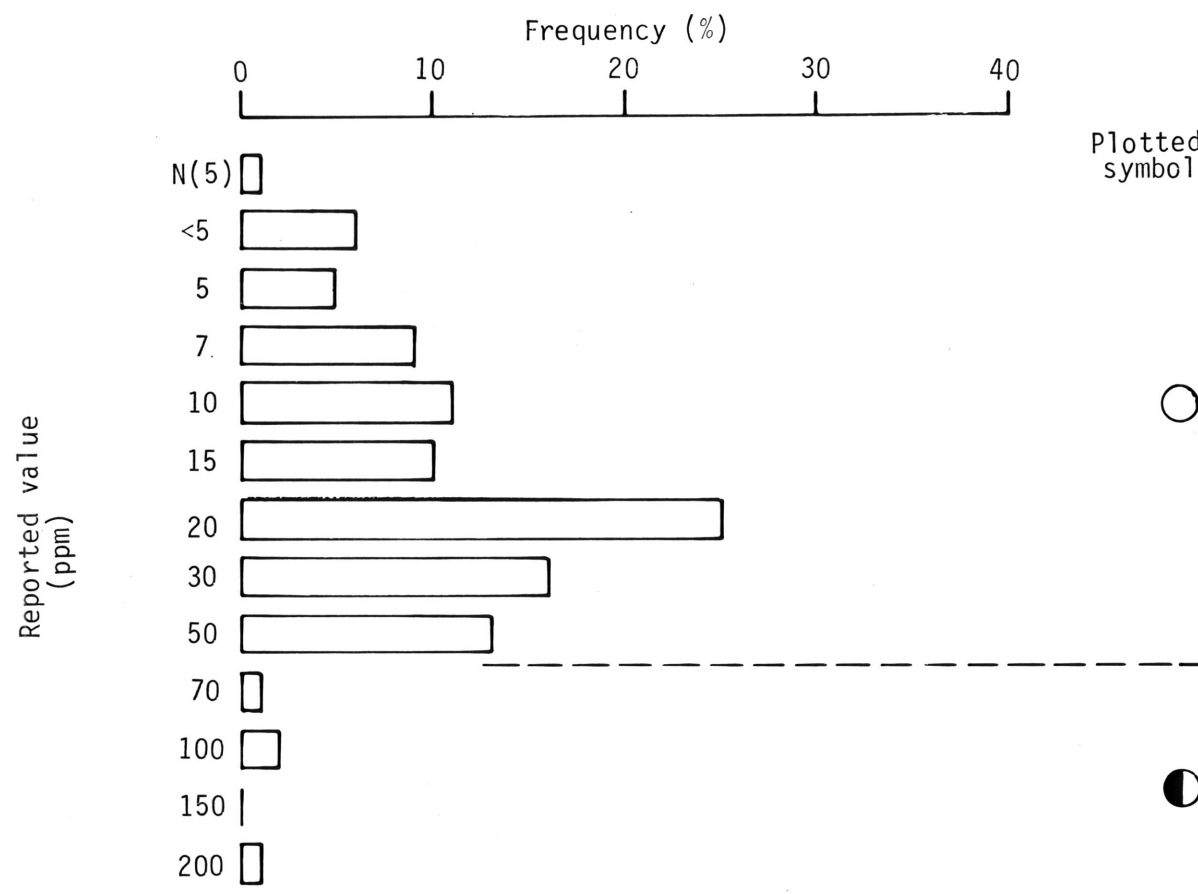
Figure 1.--Frequency diagram for copper in samples of minus-60-mesh (0.25-mm) stream sediment. [N = Not detected at the lower limit of determination shown in parentheses]
