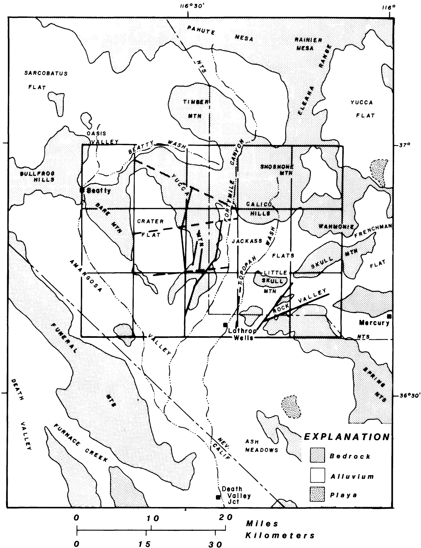
Figure 2.--Structures indicated by aeromagnetic data. Solid line where anomaly shape implies offset in magnetized rock units; dashed line where structural alignment, probably faulting, is indicated by discontinuities, gradient, and (or) contrast in regional magnetic expression.
