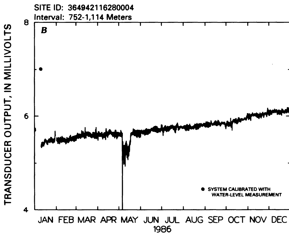
Figure 29.--Transducer output for well USW H-3.
