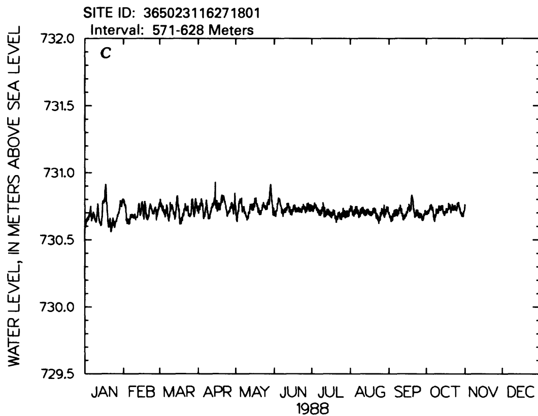
Figure 10.--Water-level altitude for well USW WT-2.--Continued
