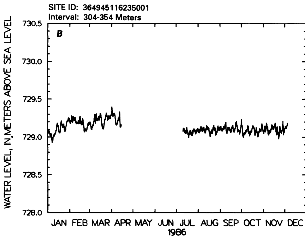
Figure 18.--Water-level altitude for well UE-25 WT #13.
