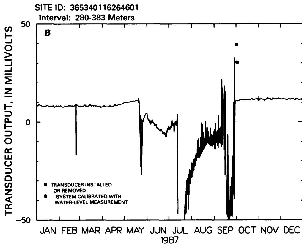
Figure 13.--Transducer output for well UE-25 WT #6.
