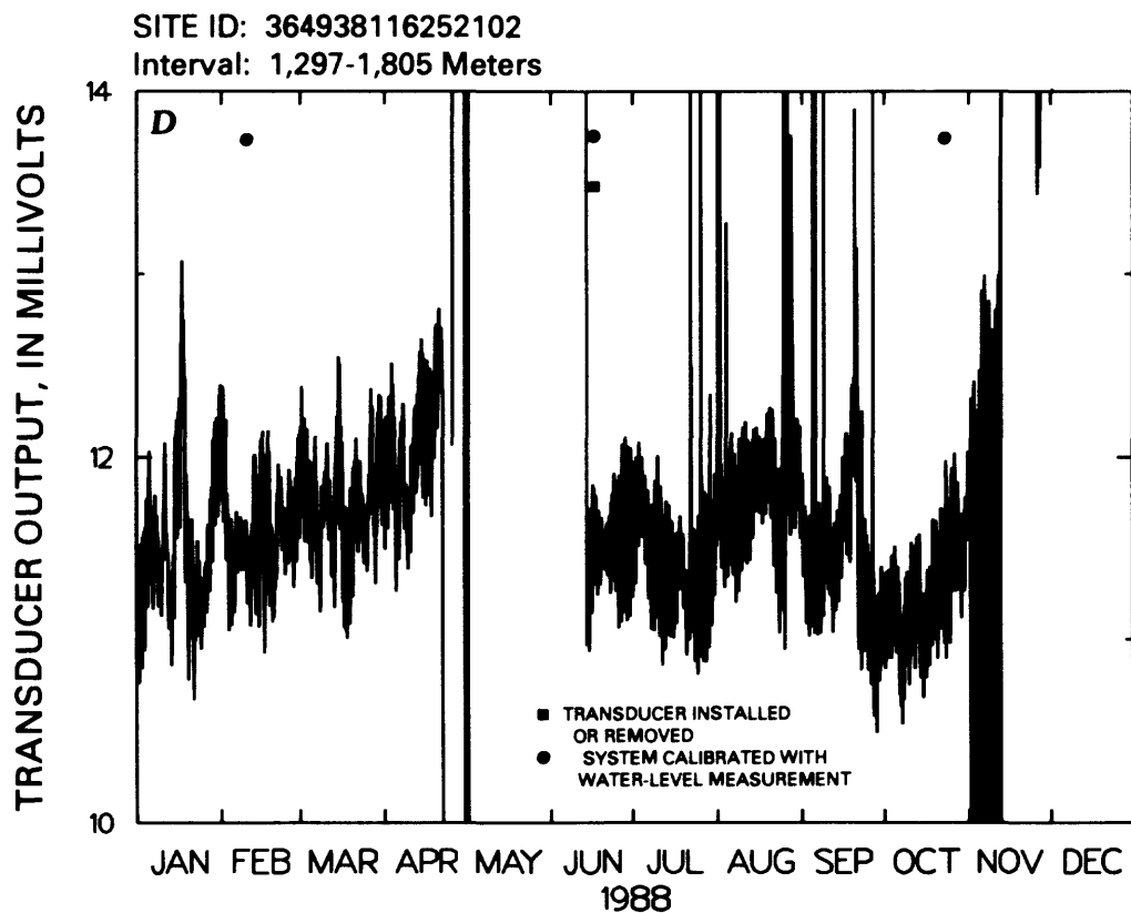
Figure 23.--Transducer output for well UE-25p #1.--Continued
