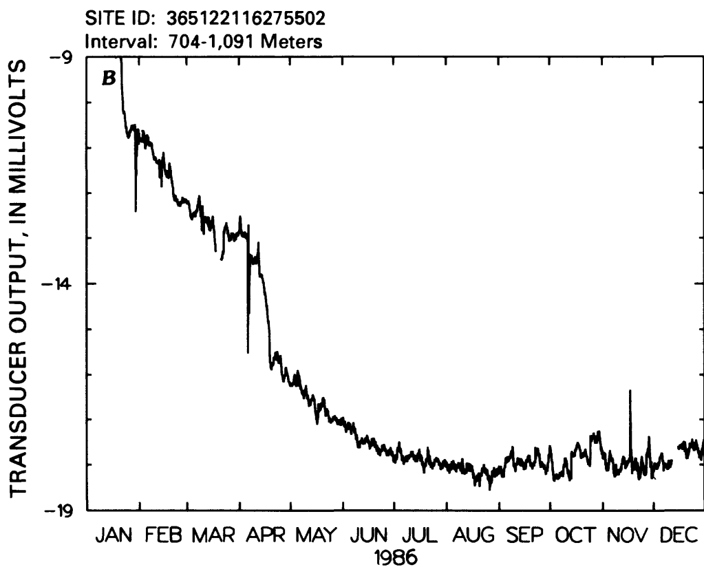
Figure 33.--Transducer output for well USW H-5.
