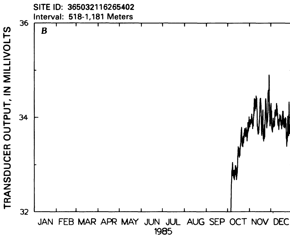
Figure 31.--Transducer output for well USW H-4.
