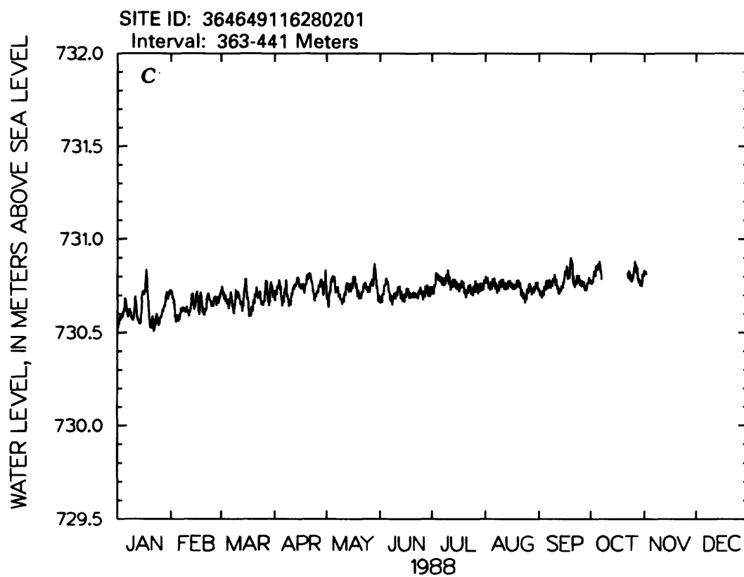
Figure 16.--Water-level altitude for well USW WT-11.--Continued
