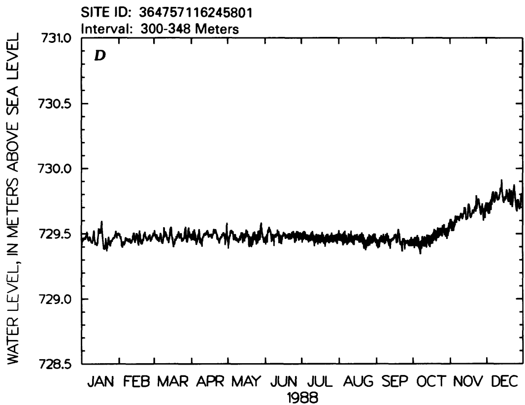
Figure 12.--Water-level altitude for well UE-25 WT #3.--Continued
