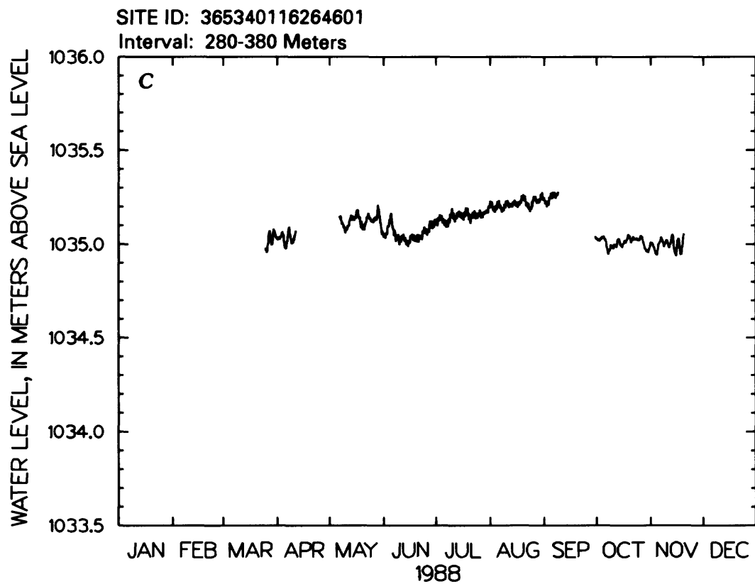
Figure 14.--Water-level altitude for well UE-25 WT #6.--Continued
