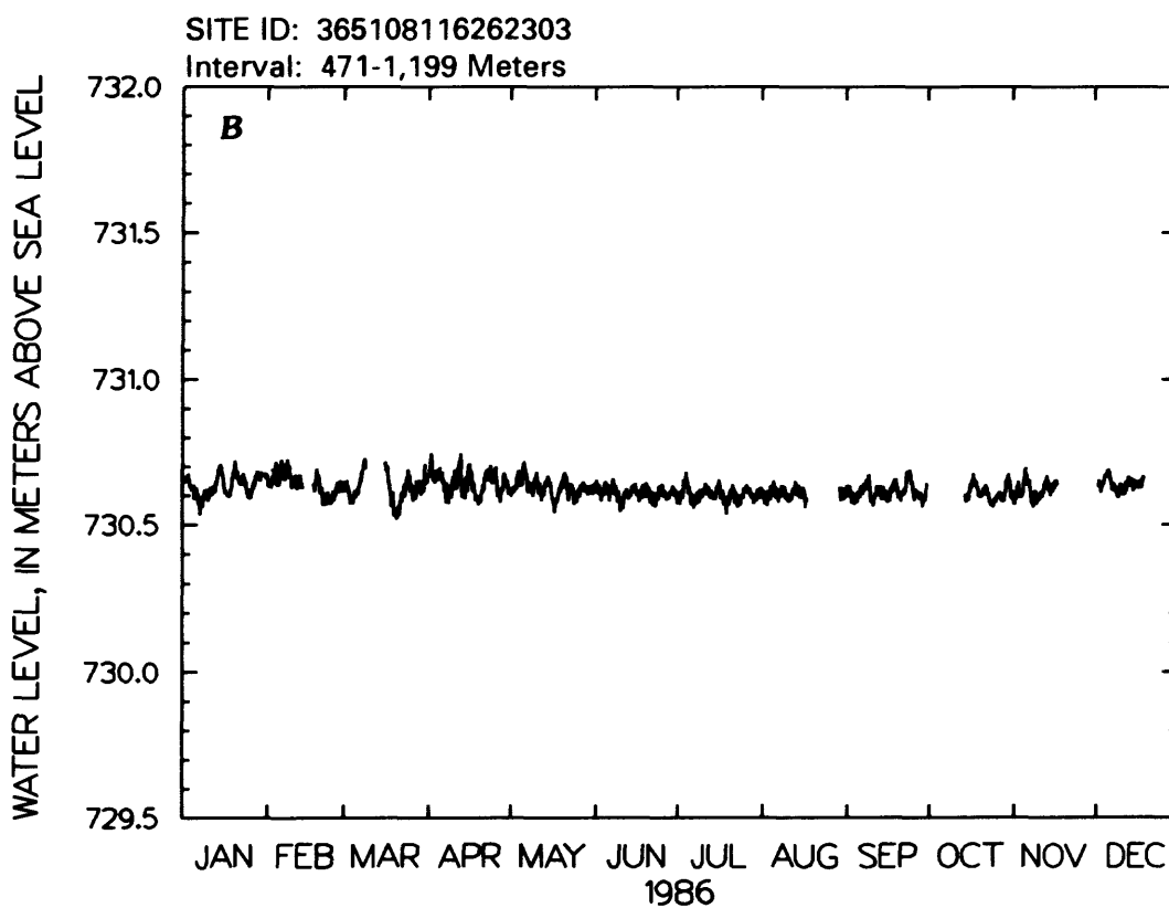
Figure 22.--Water-level altitude for well UE-25b #1.
