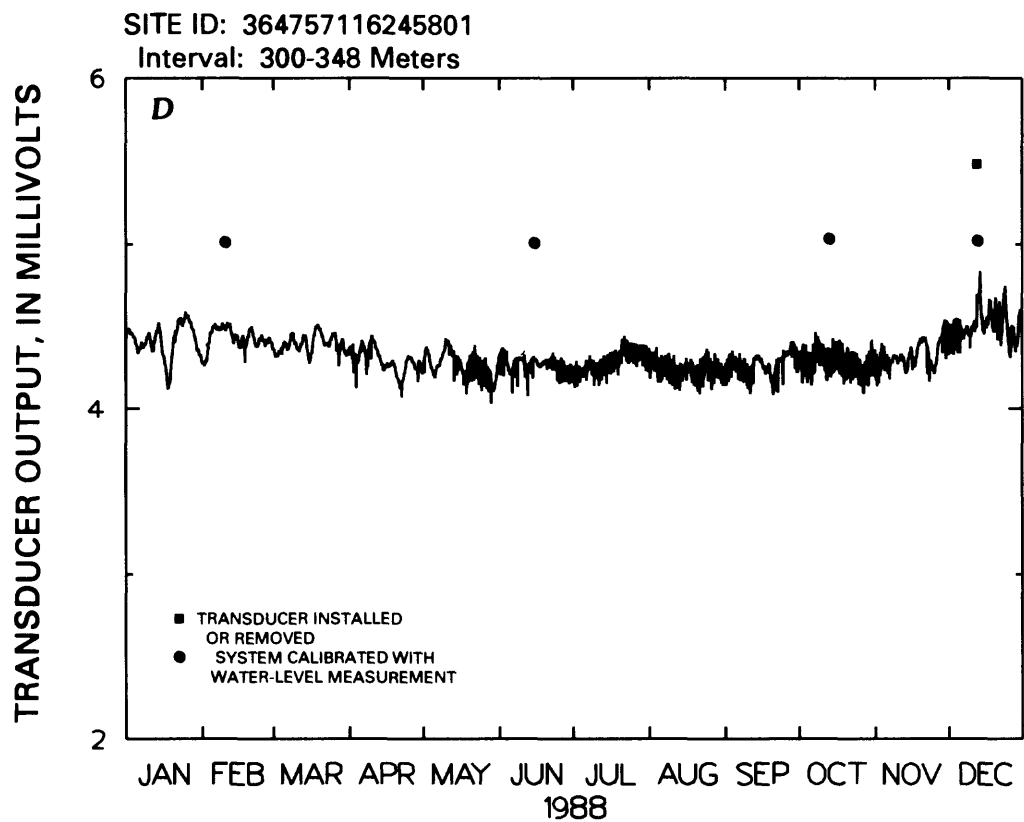
Figure 11.--Transducer output for well UE-25 WT #3.--Continued
