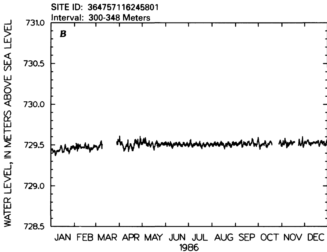
Figure 12.--Water-level altitude for well UE-25 WT #3.
