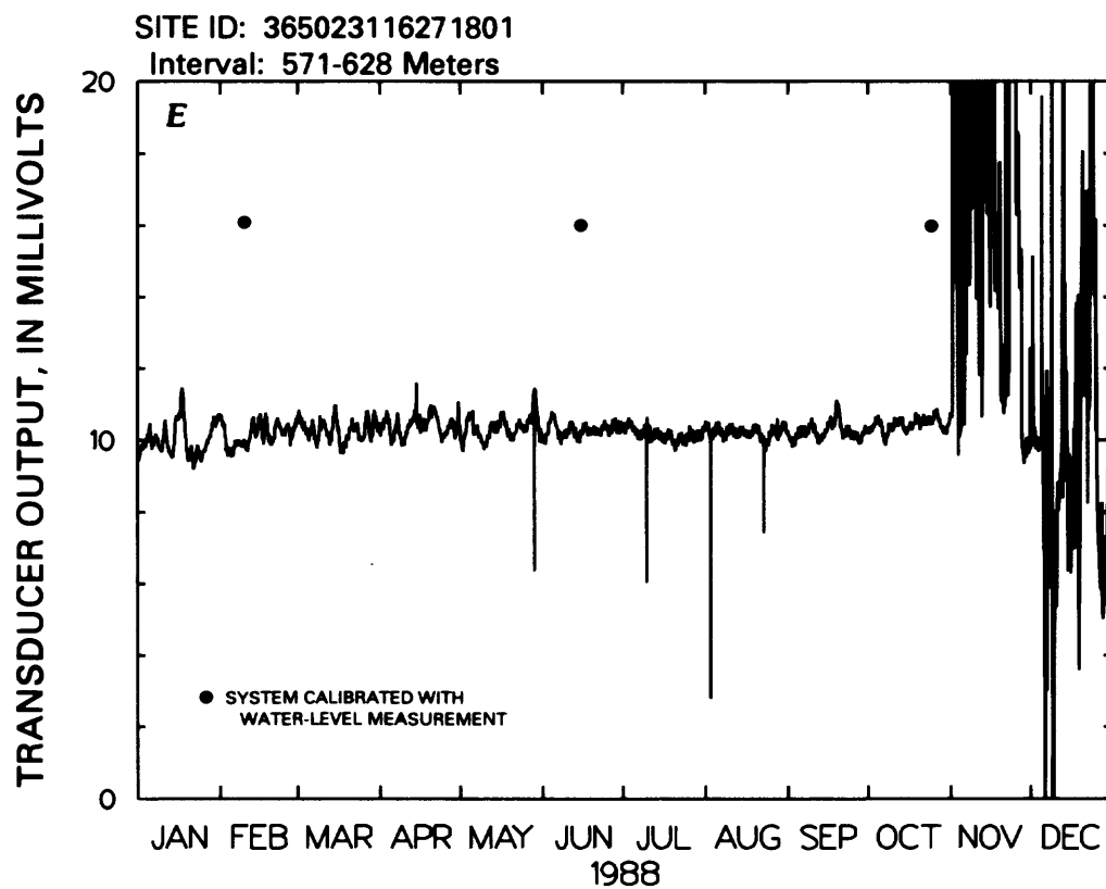
Figure 9.--Transducer output for well USW WT-2.--Continued
