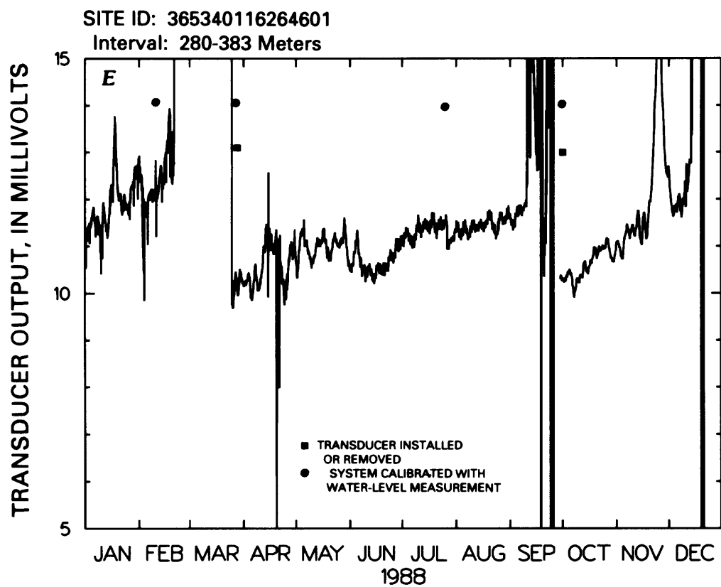
Figure 13.--Transducer output for well UE-25 WT #6.--Continued
