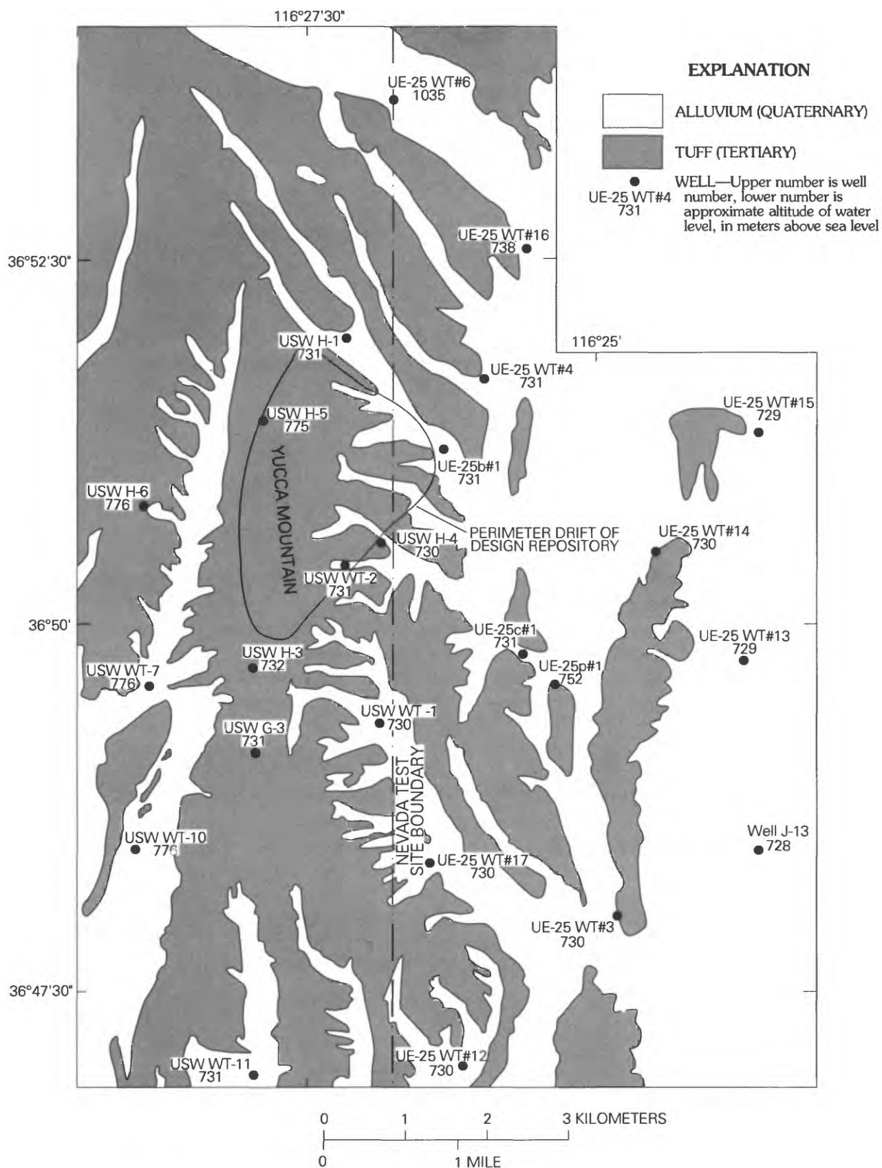
Figure 2.—Location of wells and 1988 water-level altitudes in the vicinity of Yucca Mountain (modified from Robison and others, 1988 and Gemmell, 1990).
