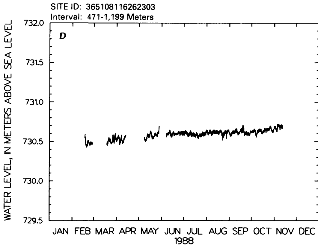
Figure 22.--Water-level altitude for well UE-25b #1.--Continued
