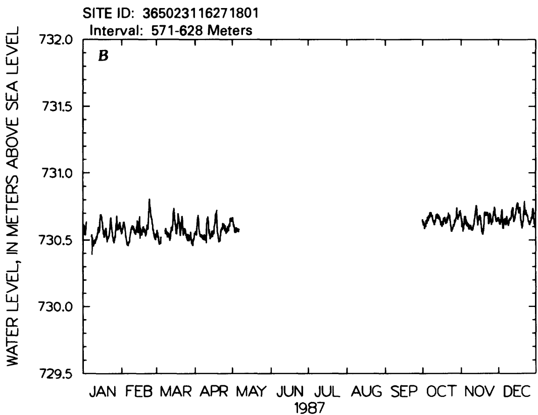
Figure 10.--Water-level altitude for well USW WT-2.
