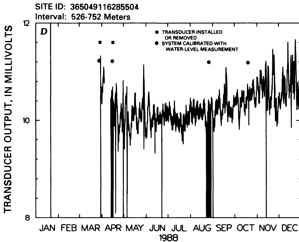
Figure 35.--Transducer output for well USW H-6.--Continued
