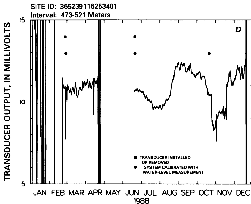
Figure 19.--Transducer output for well UE-25 WT #16.--Continued
