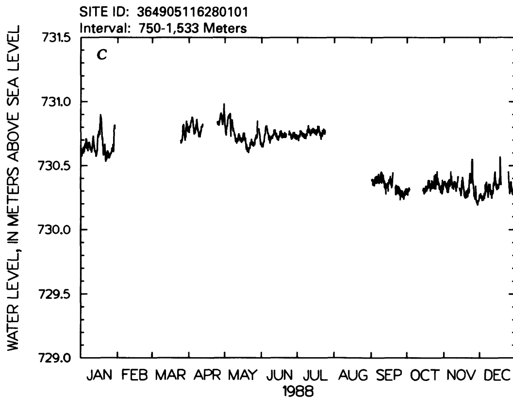
Figure 26.--Water-level altitude for well USW G-3.--Continued
