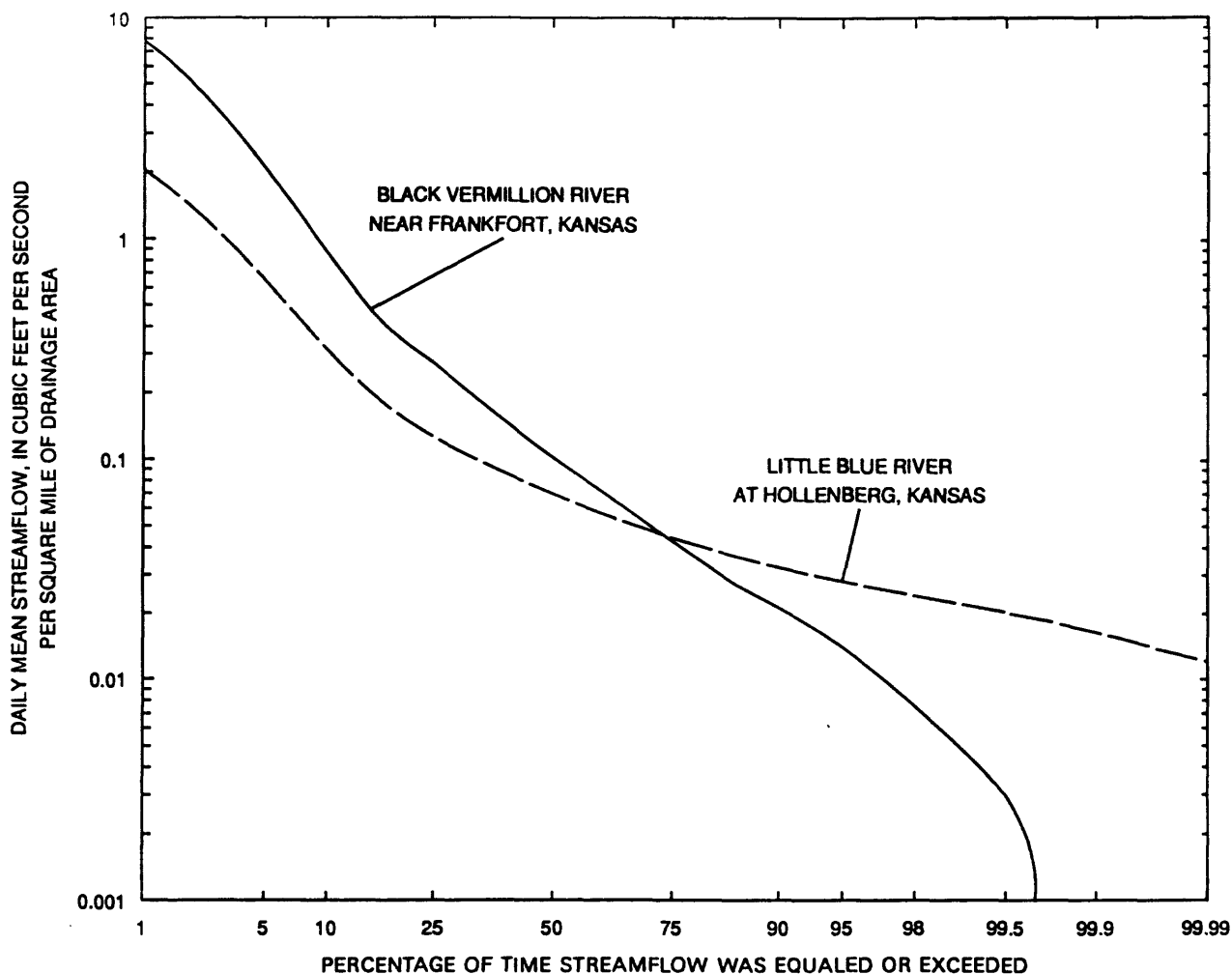
Figure 3. Streamflow-duration curves for Little Blue River at Hollenberg and Black Vermillion River near Frankfort, Kansas, 1974-87.
