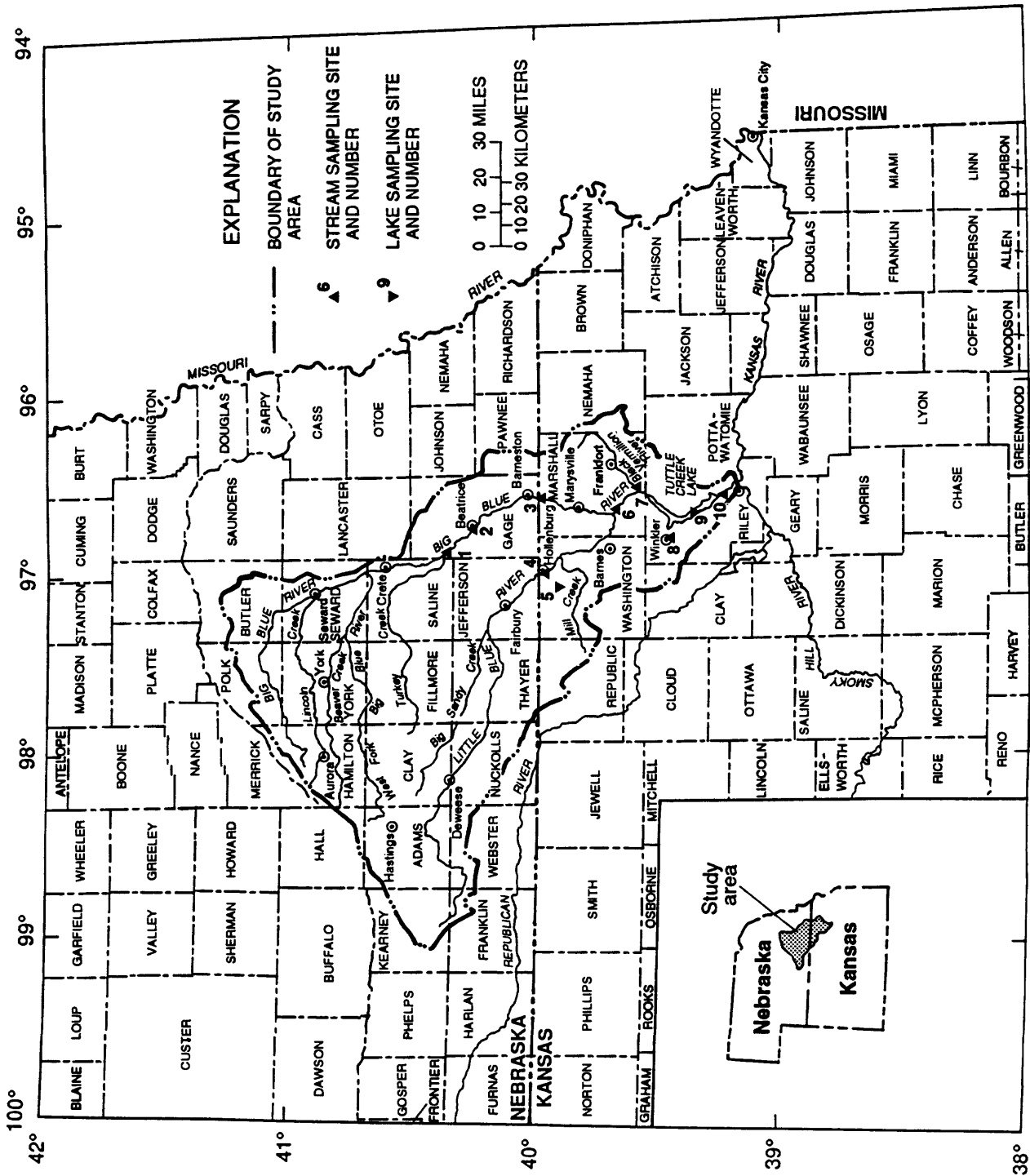
Figure 1. Location and extent of study area and location of previously sampled surface-water sites, 1969-86.
