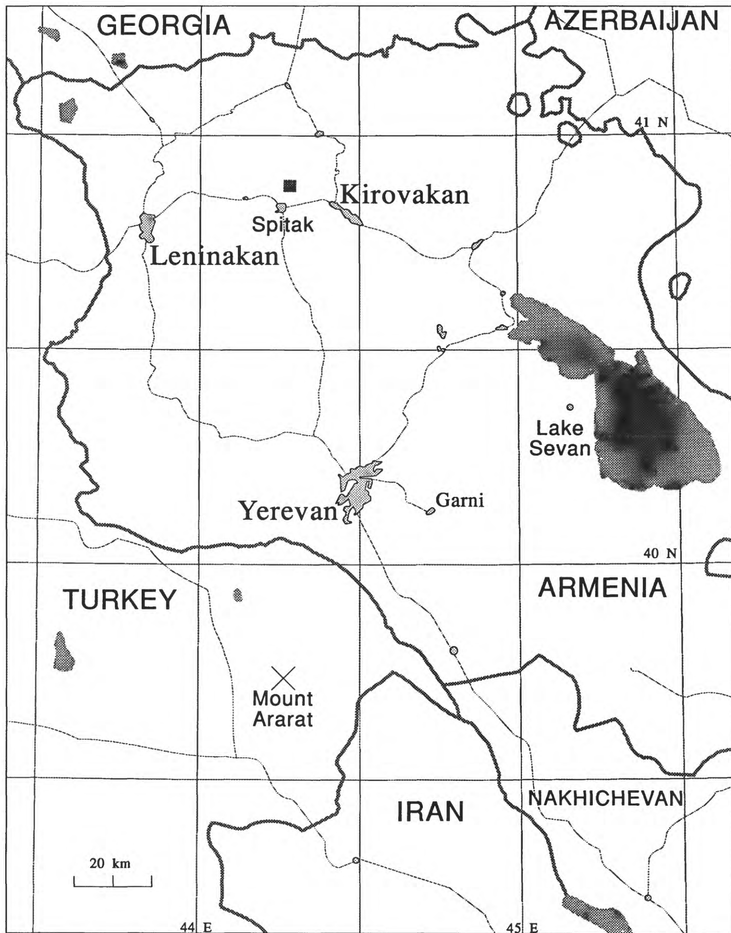
Figure 2-3. Northern Armenia with bodies of water, political boundaries, major highways, selected cities, Mt. Ararat, and the epicenter of the 1988 Spitak Earthquake.
