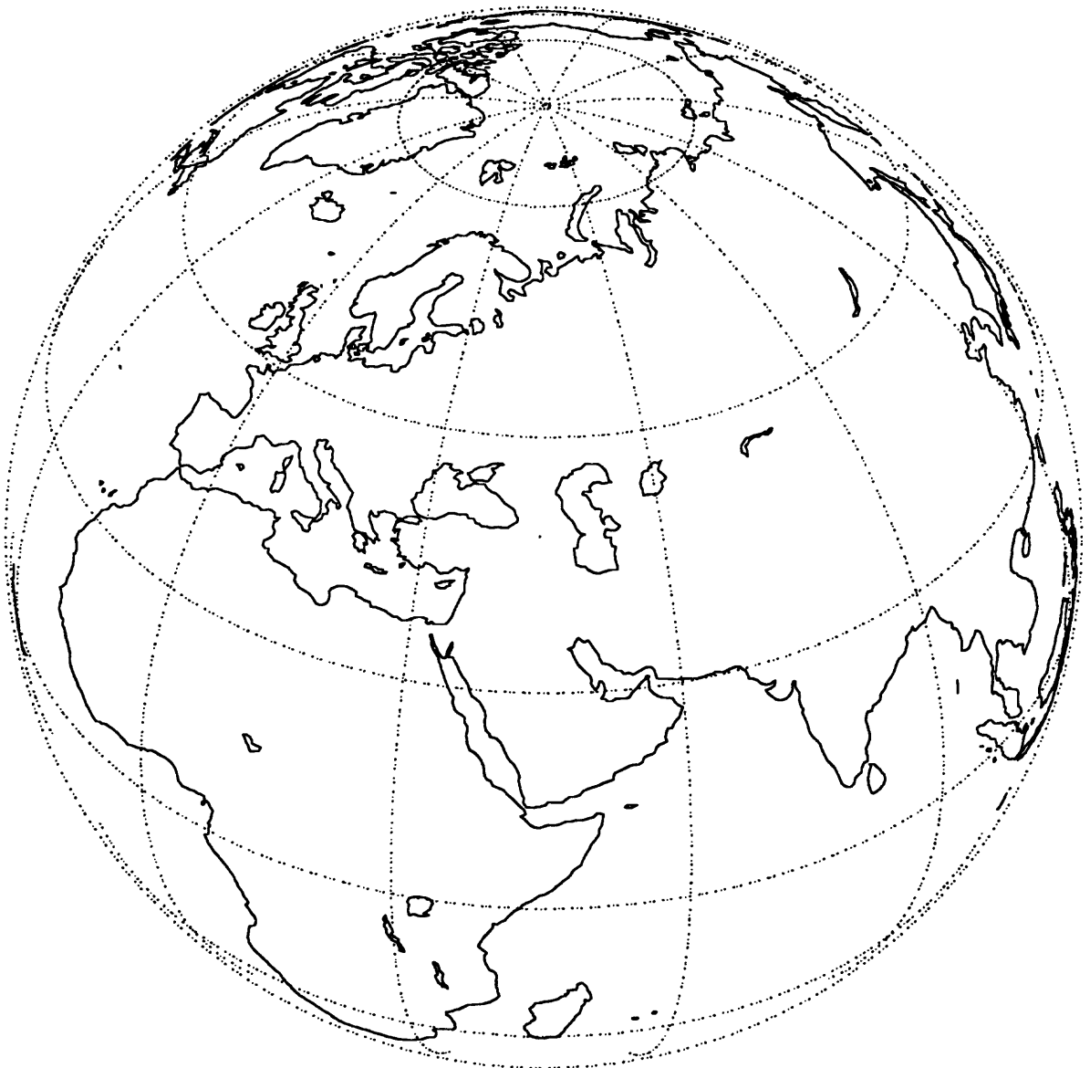
Figure 2-1. World view centered on Garni, Armenia.
