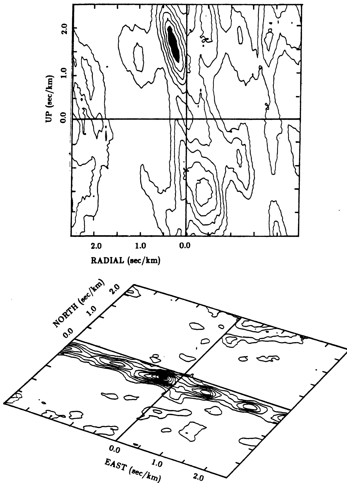
Figure 5-4. Contoured plots of combined correlation values from the S-wave window of the event at 1500 on 11/16/90.
