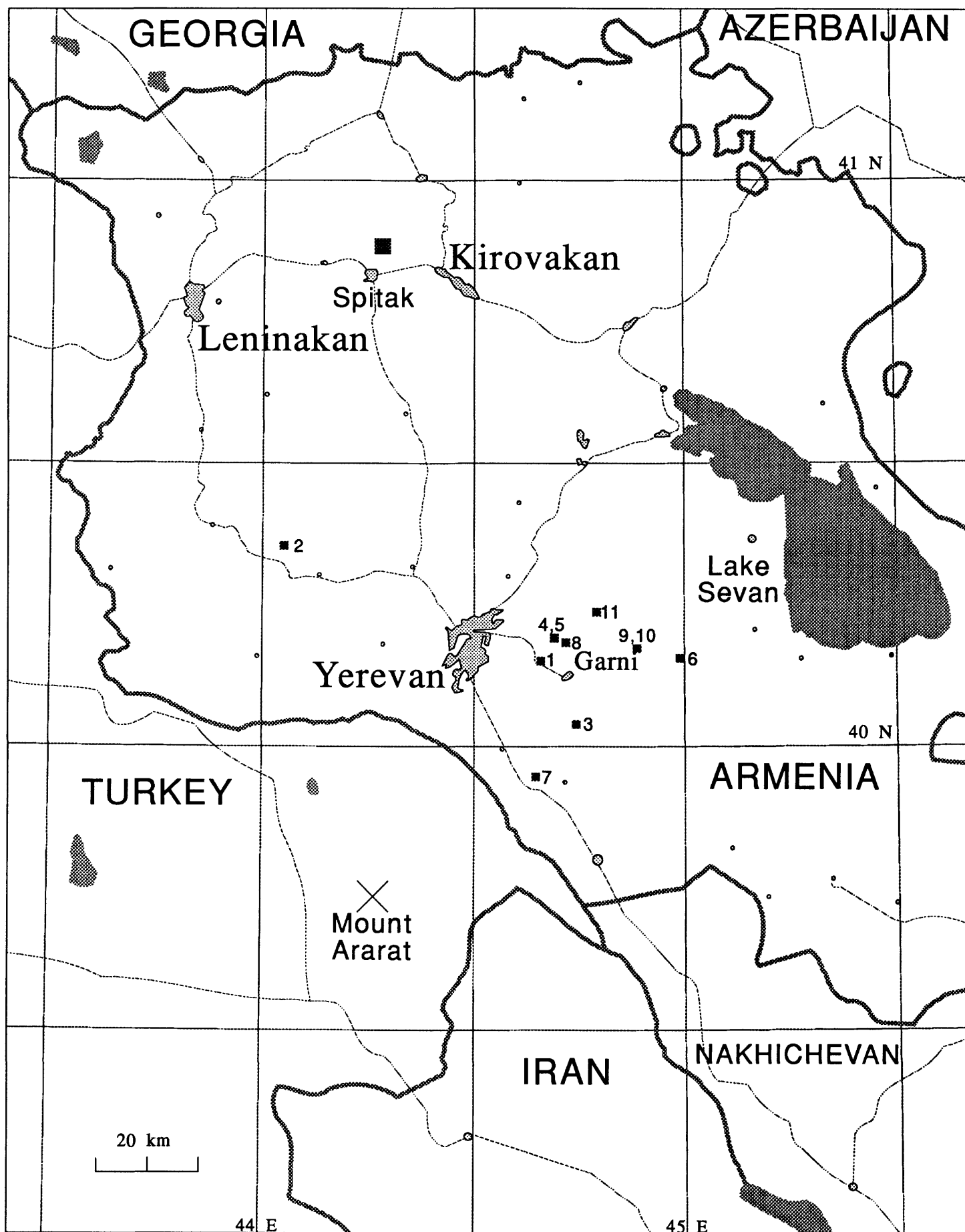
Figure 5-8. Rough locations of the numbered events from Table 5-1 shown on a map of northern Armenia.
