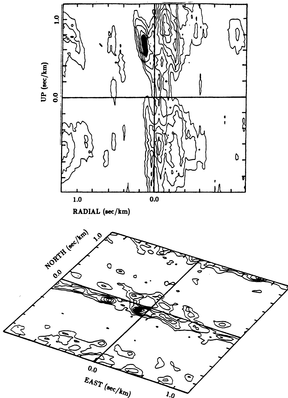
Figure 5-3. Contoured plots of combined cross correlation values for tested values of slowness from the P-wave window of the event at 1500 on 11/16/90. Vertical (top) and horizontal (bottom) slices of the three-dimensional slowness space are shown. High correlation values (shaded areas) correspond to values of slowness which are consistent with a plane-wave propagating across the array.
