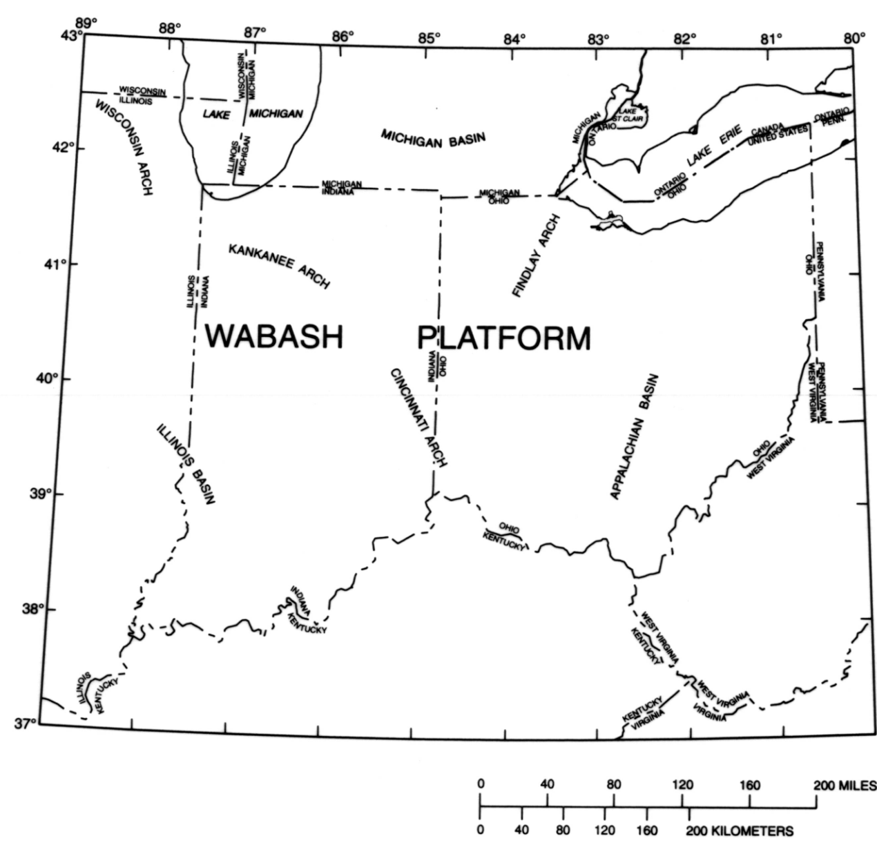
Figure 2. Structural elements of Midwestern Basins and Arches region of Indiana, Ohio, Michigan, and Illinois
