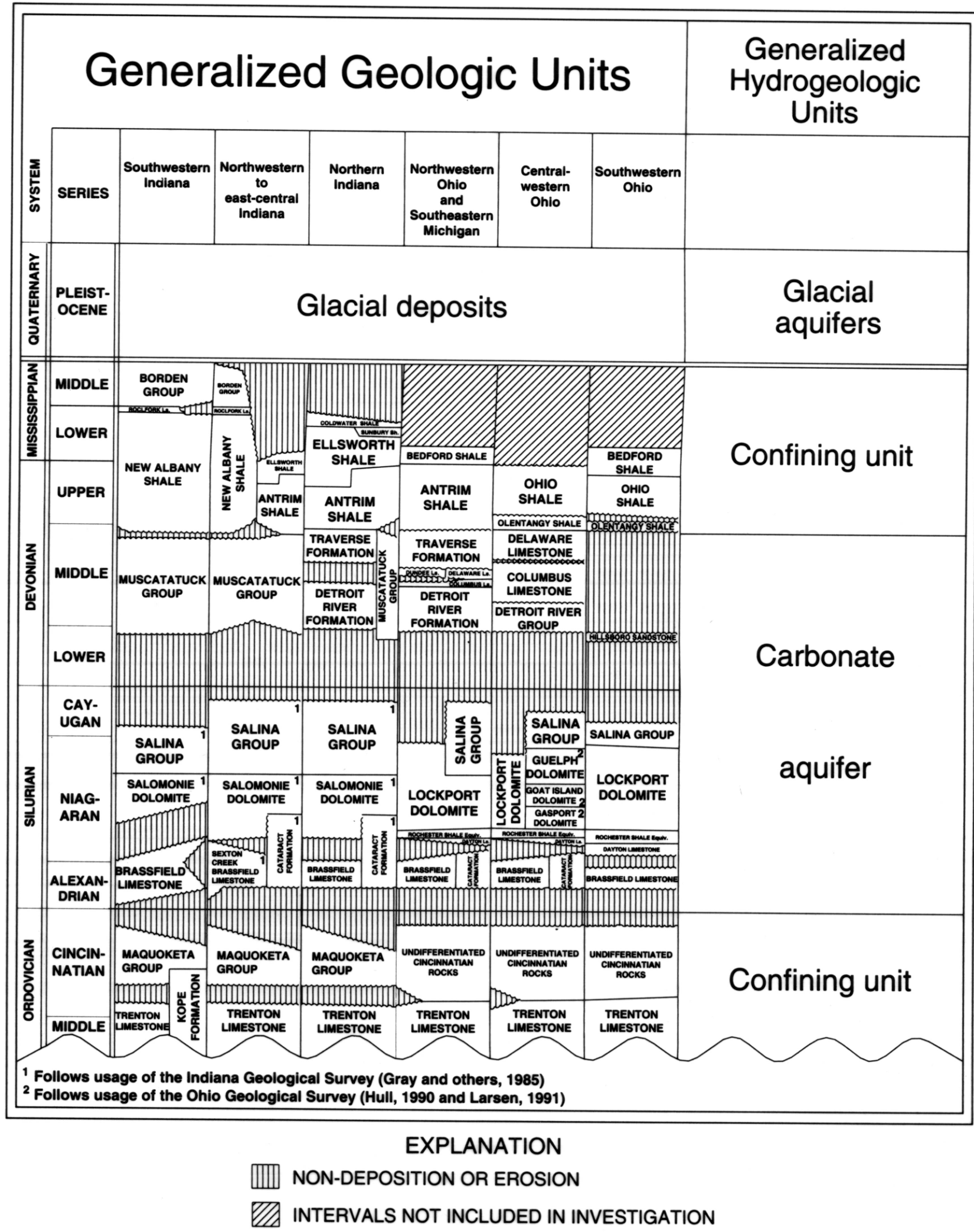
Figure 3. Time- and rock-stratigraphic framework and nomenclature (Modified from Bugliosi, 1990)
