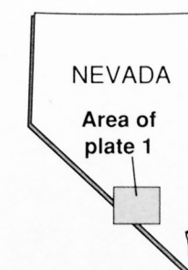
MAP SHOWING LOCATION OF DATA-COLLECTION SITES THROUGH 1992, YUCCA MOUNTAIN REGION OF SOUTHERN NEVADA AND EASTERN CALIFORNIA
