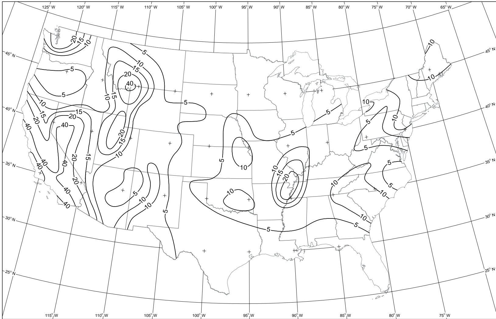
Figure A3. Contour map for effective peak velocity-related acceleration (EPV) coefficient, A_v , for the continental United States. The units of EPV are expressed as a percent of gravity. After BSSC, 1995 (This map was redrawn from the original source, if differences occur, the original source should be used).
