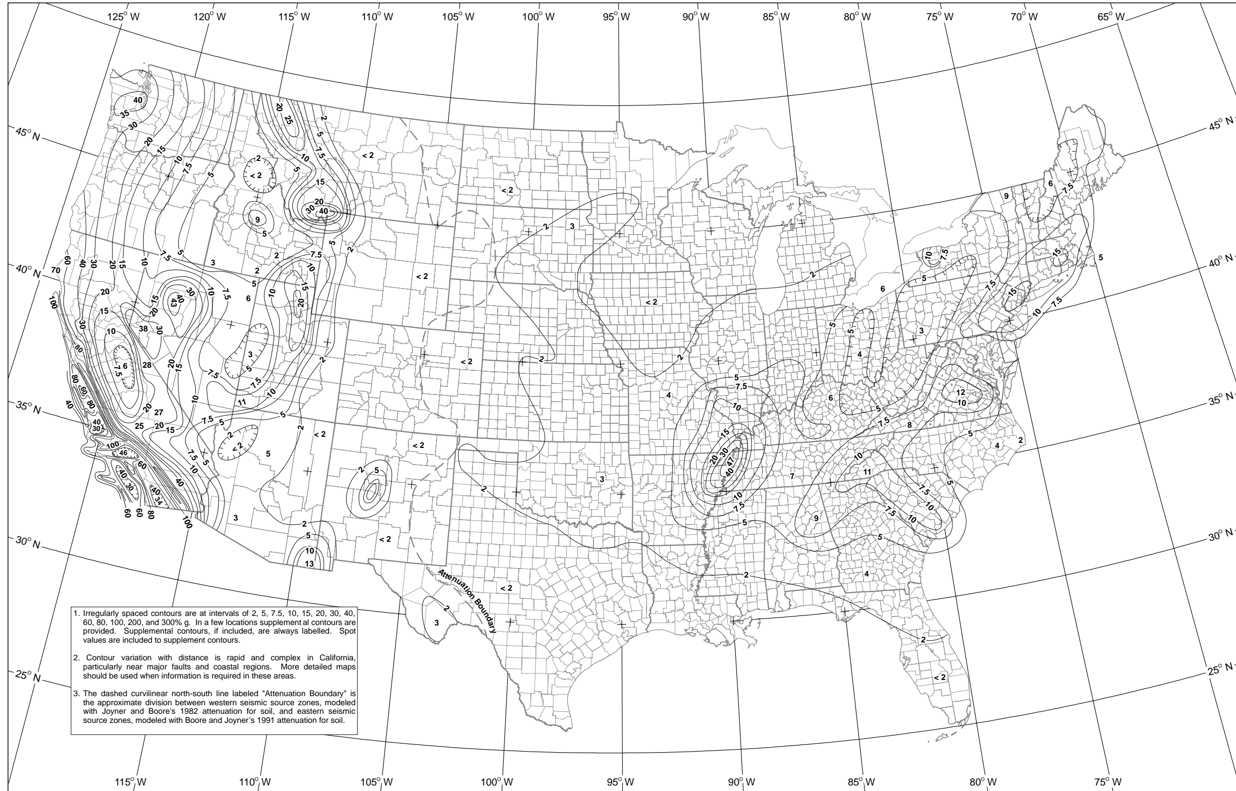
Figure B2. 1994 contour map of the 5 percent damped, 1.0 second pseudo-acceleration spectral response, expressed in percent of the acceleration of gravity, with a 10 percent probability of exceedance in 50 years. The map values include estimates of variability in the attenuation of spectral acceleration and in fault rupture length.
