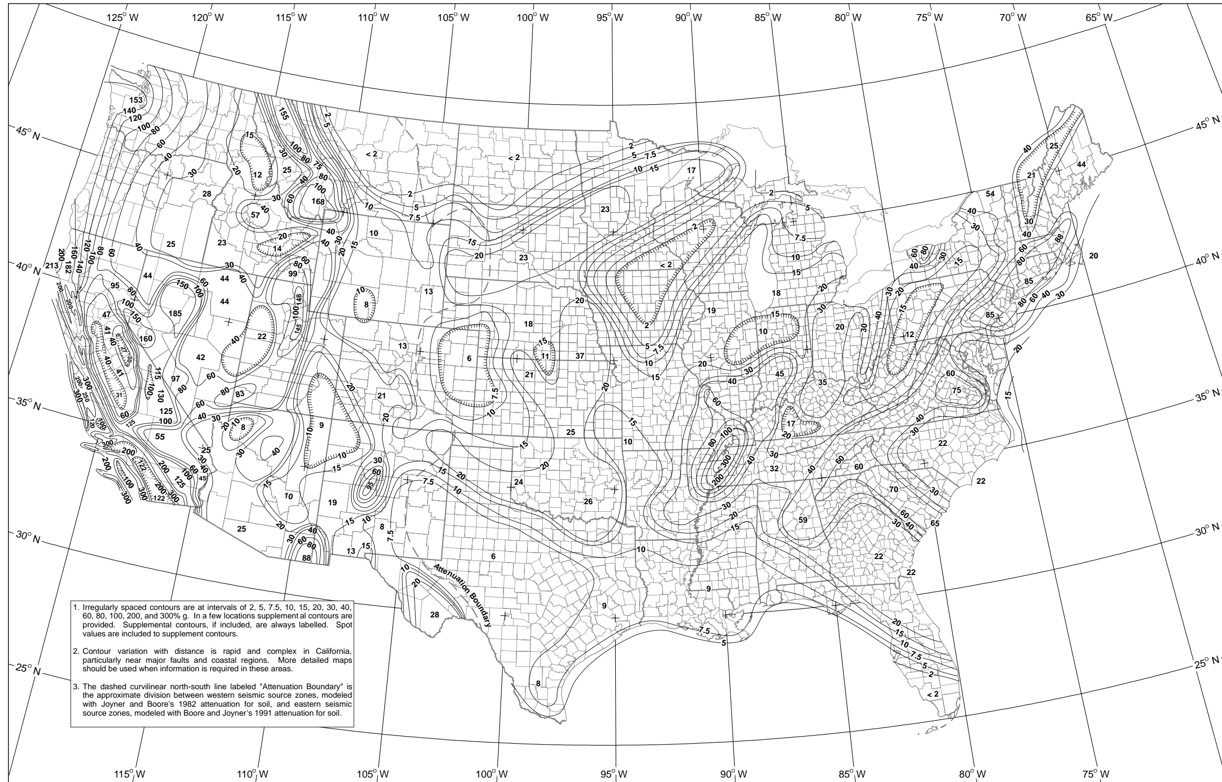
Figure B3. 1994 contour map of the 5 percent damped, 0.3 second pseudo-acceleration spectral response, expressed in percent of the acceleration of gravity, with a 10-percent probability of exceedance in 250 years. The map values include estimates of variability in the attenuation of spectral acceleration and in fault rupture length.
