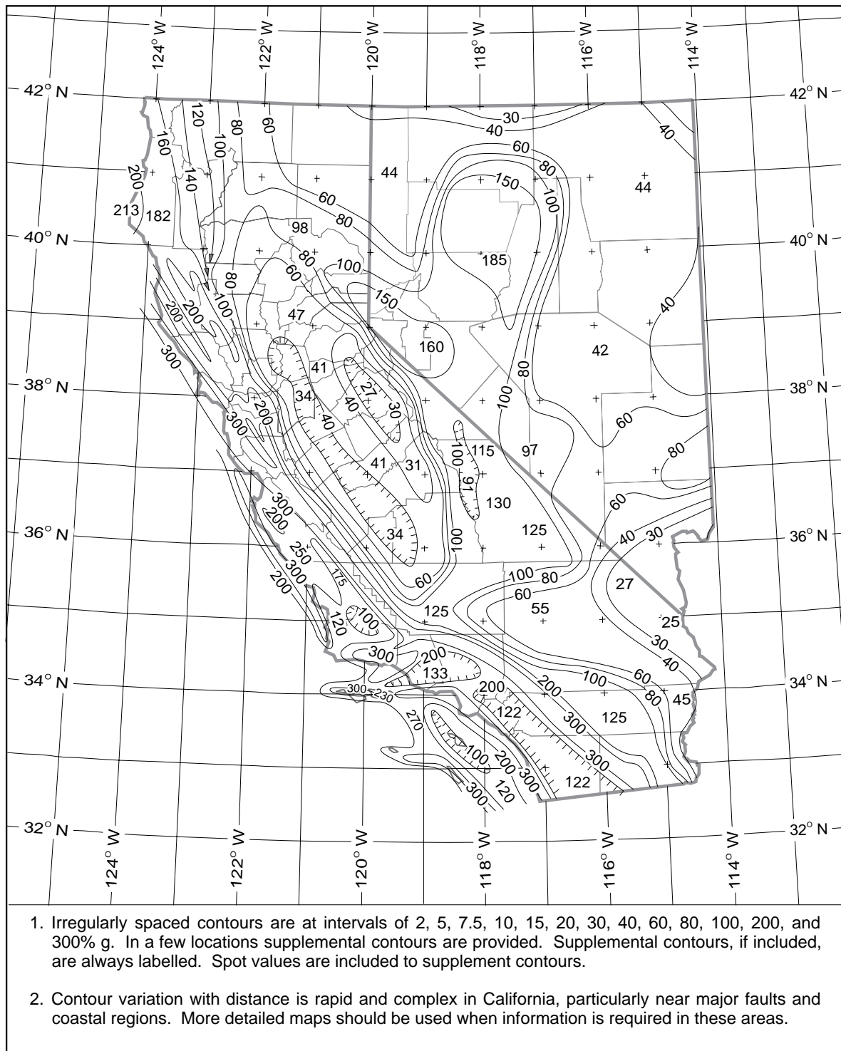
Figure B7. 1994 contour map of the 5 percent damped, 0.3 second pseudo-acceleration spectral response, expressed in percent of the acceleration of gravity, with a 10-percent probability of exceedance in 250 years. The map values include estimates of variability in the attenuation of spectral acceleration and in fault rupture length.
