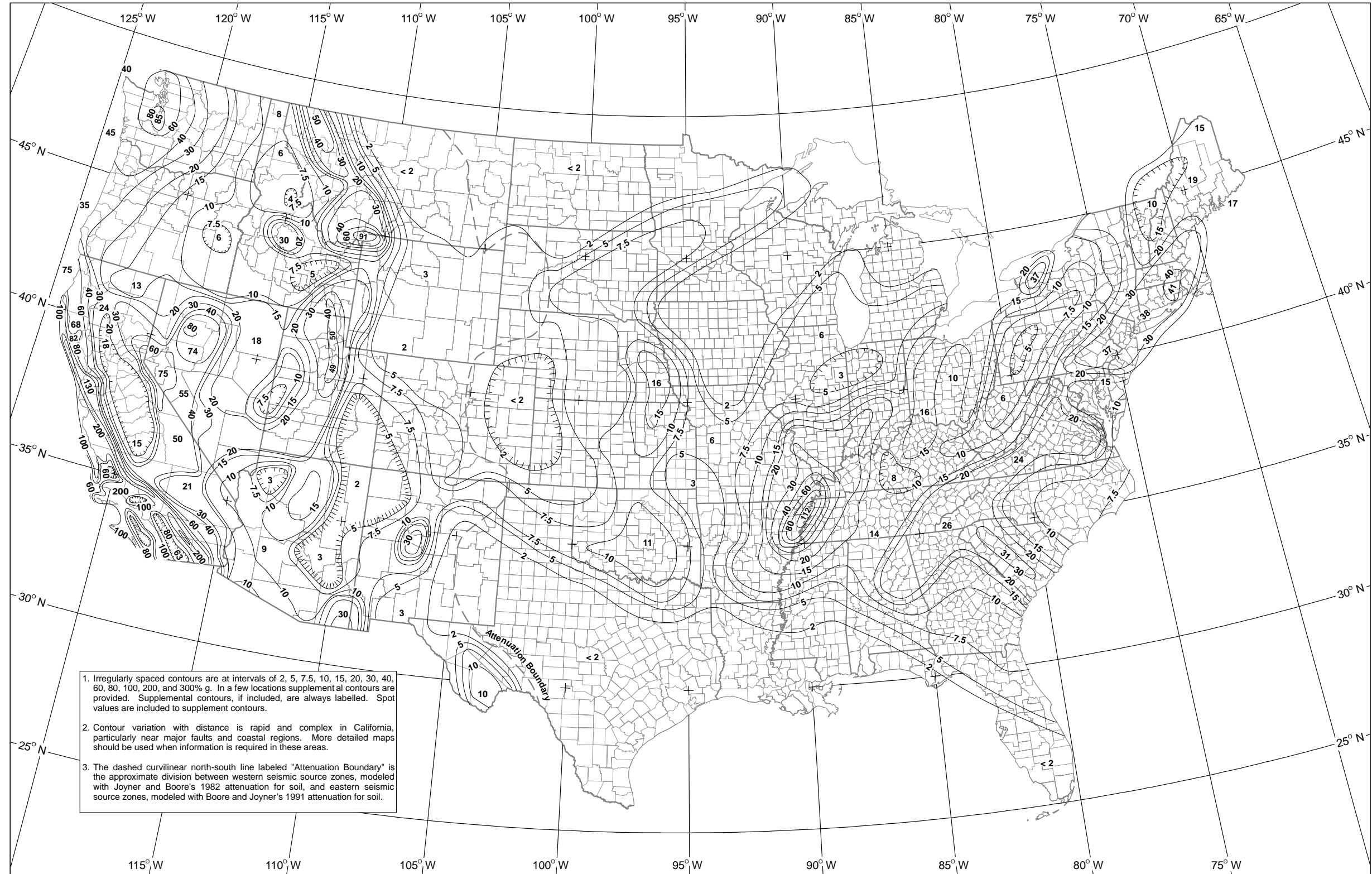
Figure C1. 1991 contour map of the 5 percent damped, 0.3 second pseudo-acceleration spectral response, expressed in percent of the acceleration of gravity, with a 10-percent probability of exceedance in 50 years. The map values include estimates of variability in the attenuation of spectral acceleration and in fault rupture length.
