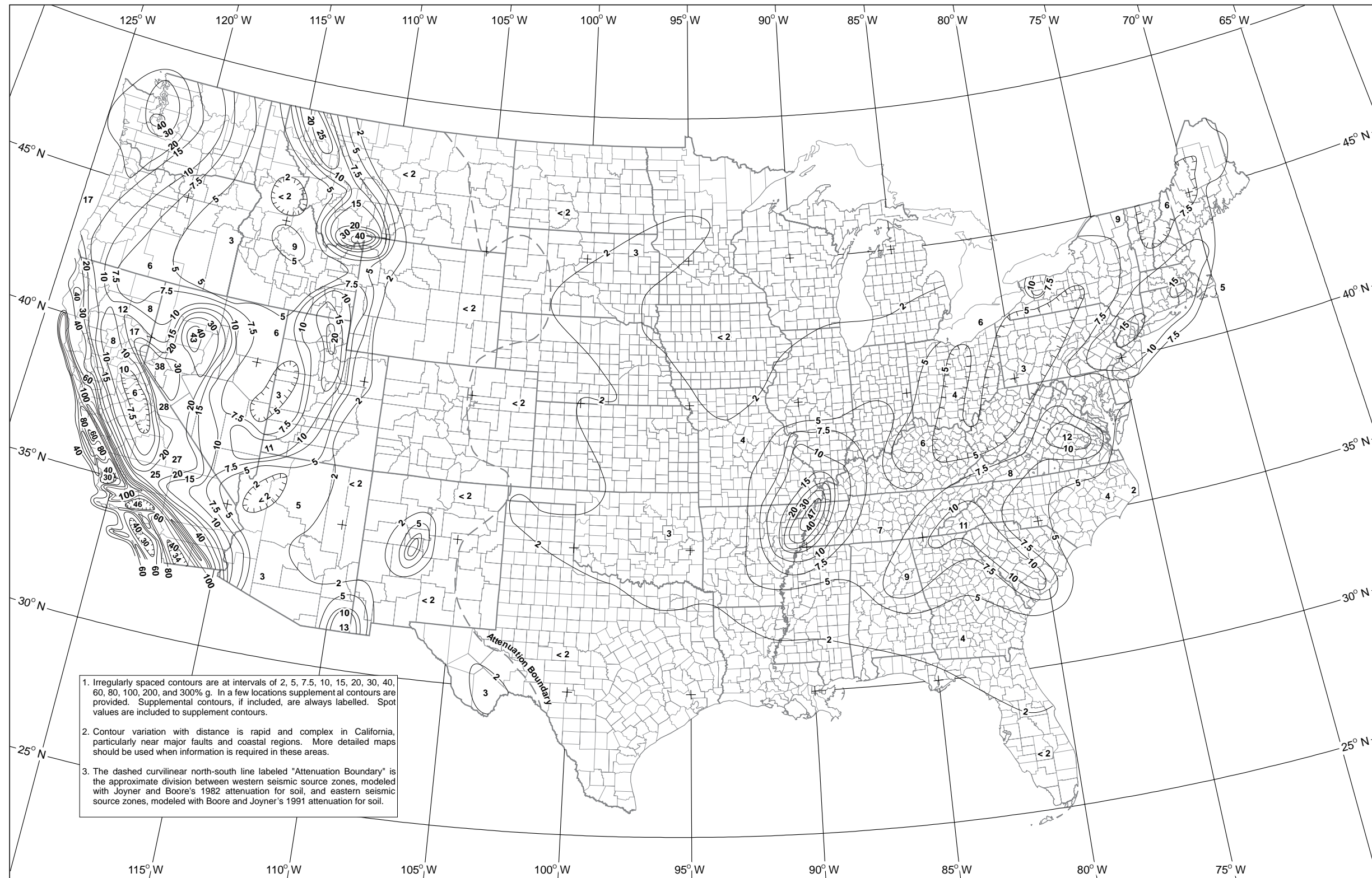
Figure C2. 1991 contour map of the 5 percent damped, 1.0 second pseudo-acceleration spectral response, expressed in percent of the acceleration of gravity, with a 10 percent probability of exceedance in 50 years. The map values include estimates of variability in the attenuation of spectral acceleration and in fault rupture length.
