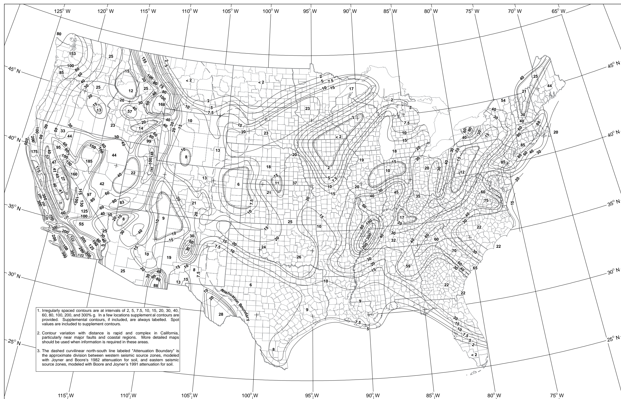
Figure C3. 1991 contour map of the 5 percent damped, 0.3 second pseudo-acceleration spectral response, expressed in percent of the acceleration of gravity, with a 10-percent probability of exceedance in 250 years. The map values include estimates of variability in the attenuation of spectral acceleration and in fault rupture length.
