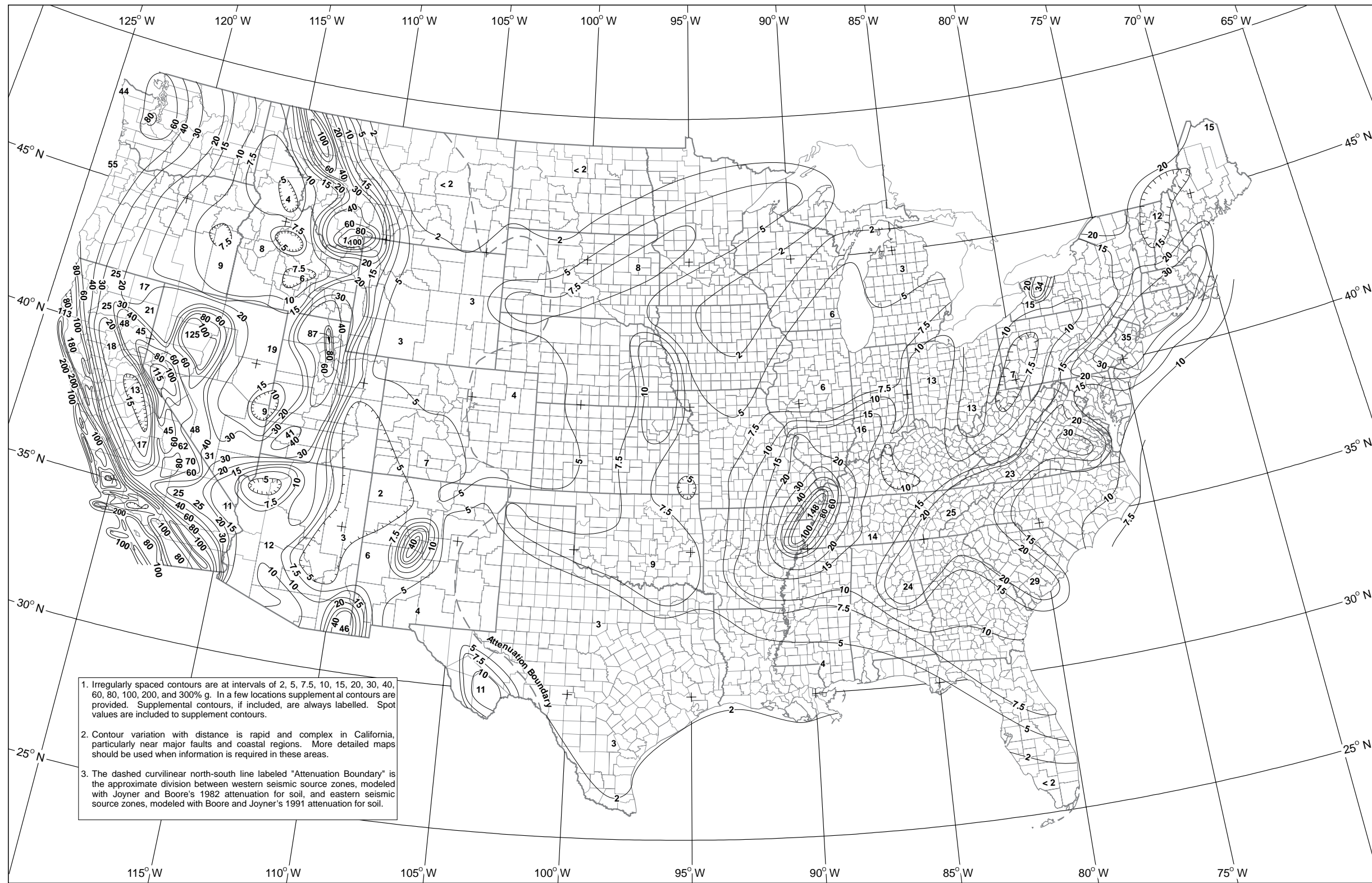
Figure C4. 1991 contour map of the 5 percent damped, 1.0 second pseudo-acceleration spectral response, expressed in percent of the acceleration of gravity, with a 10 percent probability of exceedance in 250 years. The map values include estimates of variability in the attenuation of spectral acceleration and in fault rupture length.
