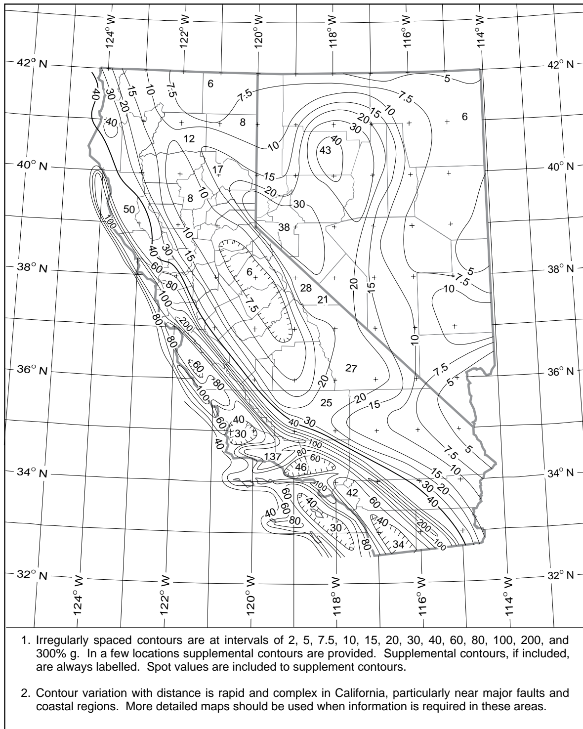
Figure C6. 1991 USGS map of the 5 percent damped, 1.0 second pseudo-acceleration spectral response, expressed in percent of the acceleration of gravity, with a 10-percent probability of exceedance in 50 years. The map values include estimates of variability in the attenuation of spectral acceleration and in fault rupture length.
