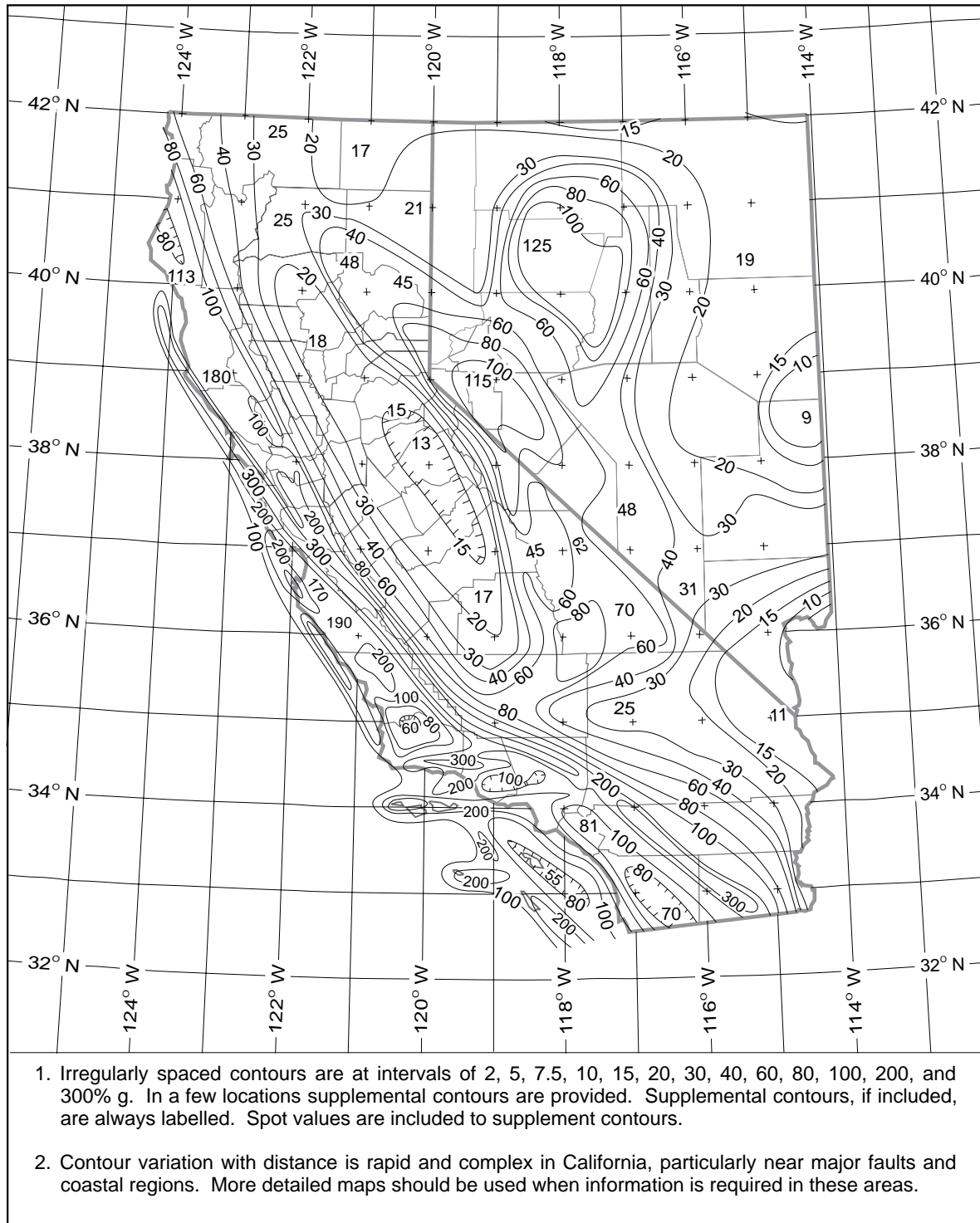
Figure C8. 1991 contour map of the 5 percent damped, 1.0 second pseudo-acceleration spectral response, expressed in percent of the acceleration of gravity, with a 10-percent probability of exceedance in 250 years. The map values include estimates of variability in the attenuation of spectral acceleration and in fault rupture length.
