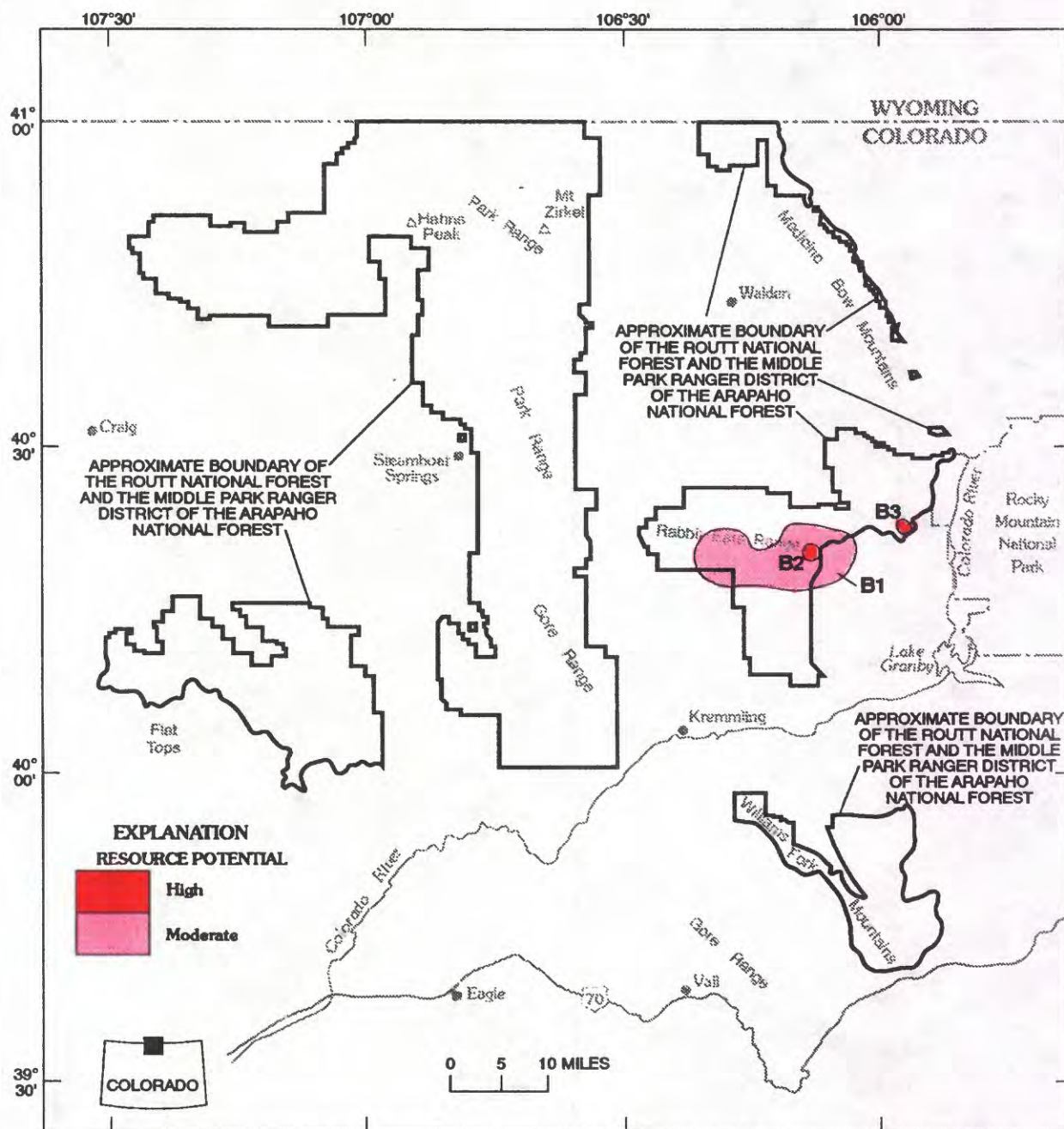
Figure 15. Mineral resource map for stockwork copper-molybdenum deposits (B) in the Routt National Forest and Middle Park Ranger District of the Arapaho National Forest, Colorado
