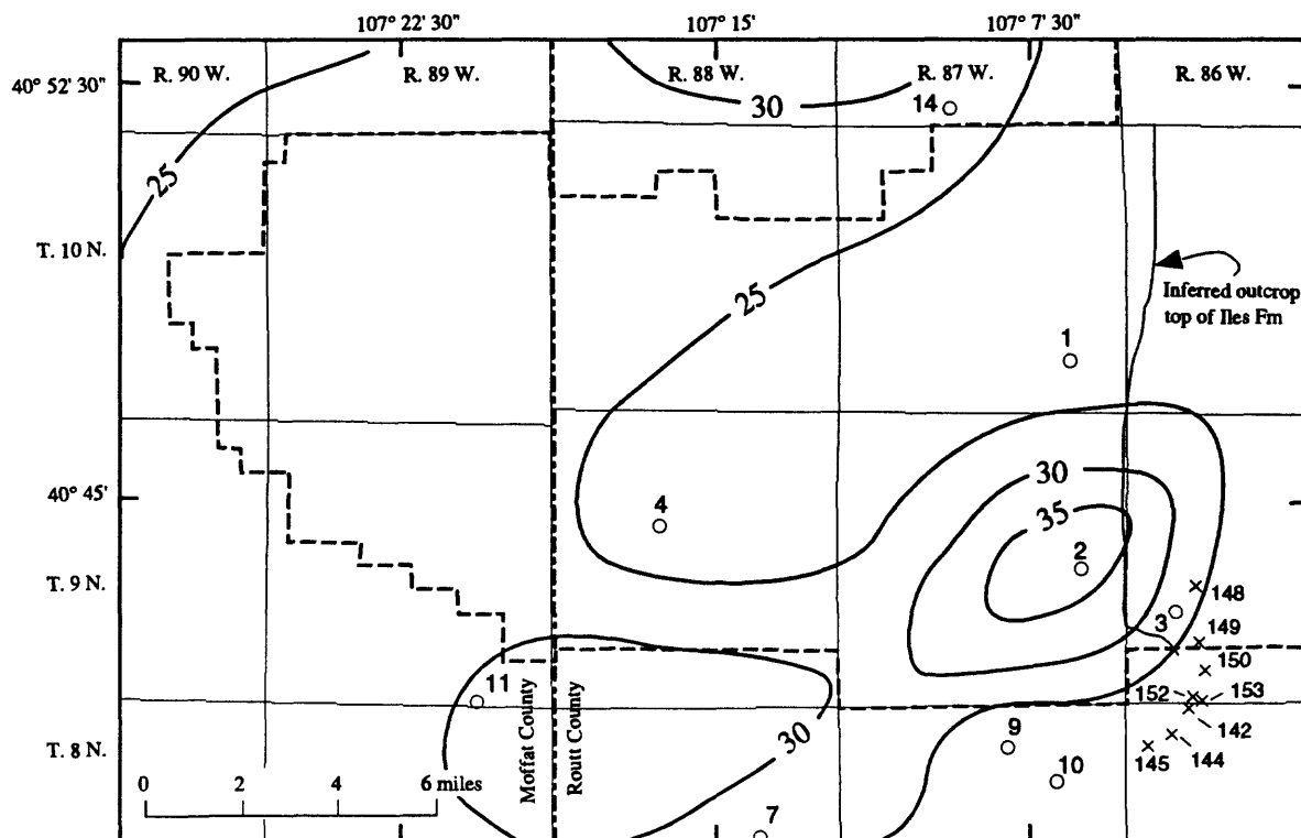
Figure 30a. Isopach map of cumulative coal in the Iles Formation in and near Area 1, including coals of the lower coal group (terminology of Bass and others, 1955). Thickness values are in feet.
