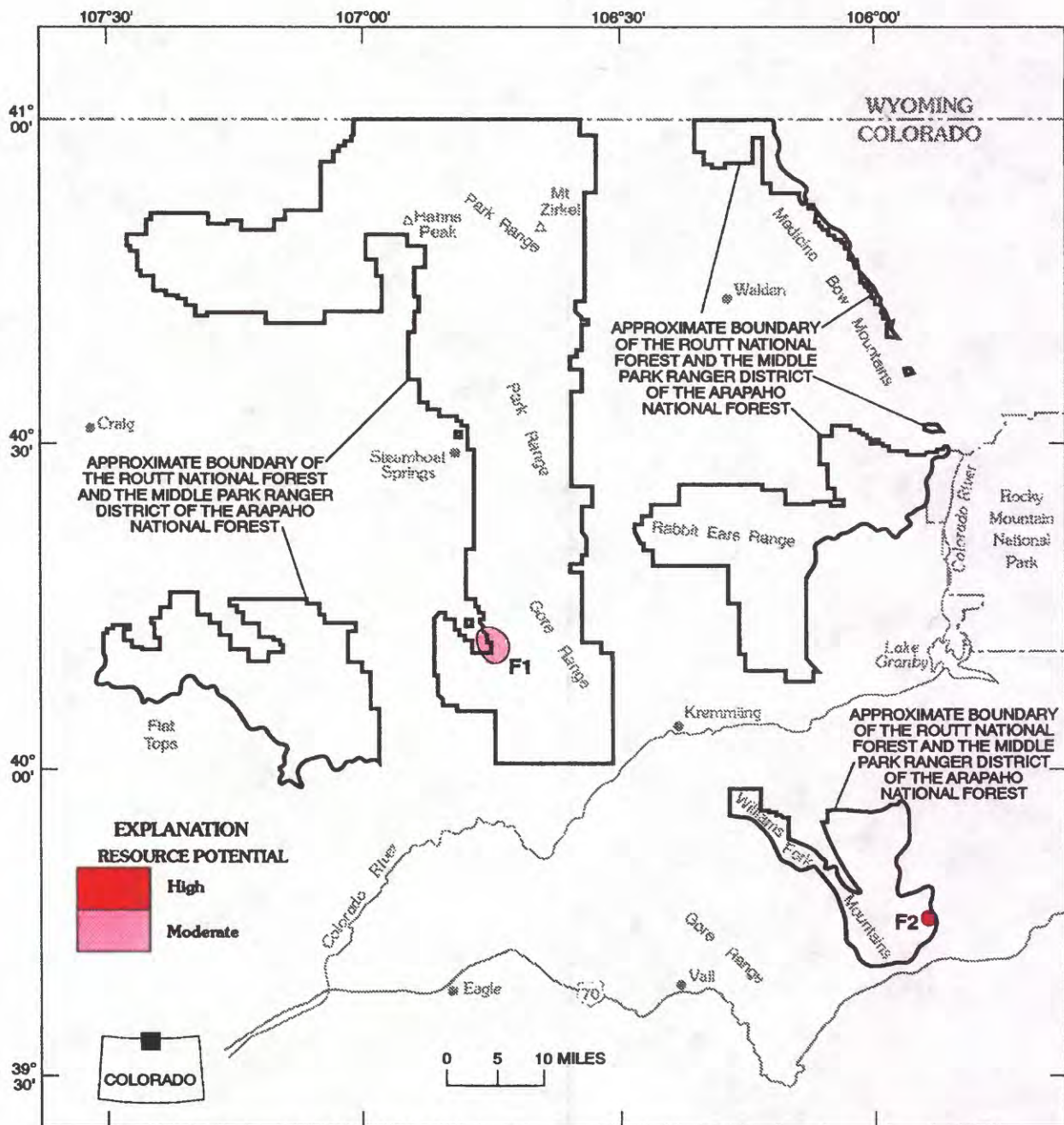
Figure 19. Mineral resource map for vein uranium (F) in the Routt National Forest and Middle Park Ranger District of the Arapaho National Forest, Colorado
