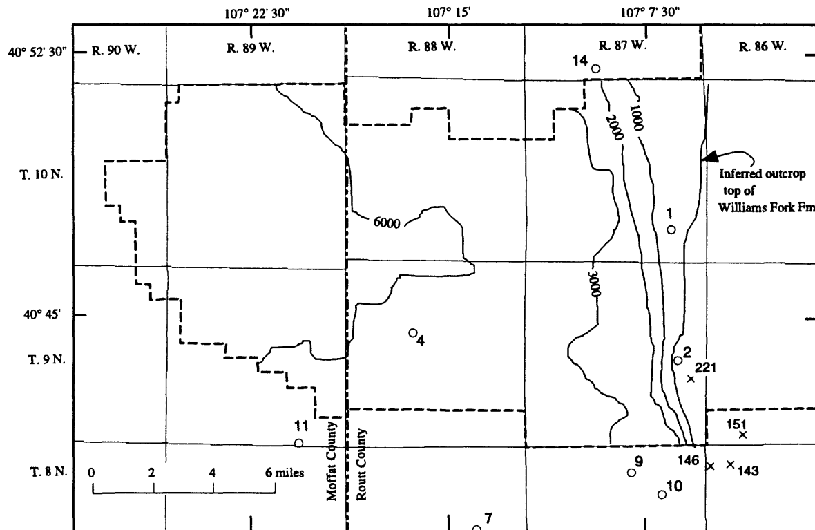
Figure 31b. Isopach map of overburden; datum is top of Williams Fork Formation in the Area 1. Thickness values are in feet. Drill holes represented by (o) and number, measured outcrop sections by (x) and number. See table 2 for location and source data for drill holes; see table 3 for the location, thickness and source data for measured sections.
