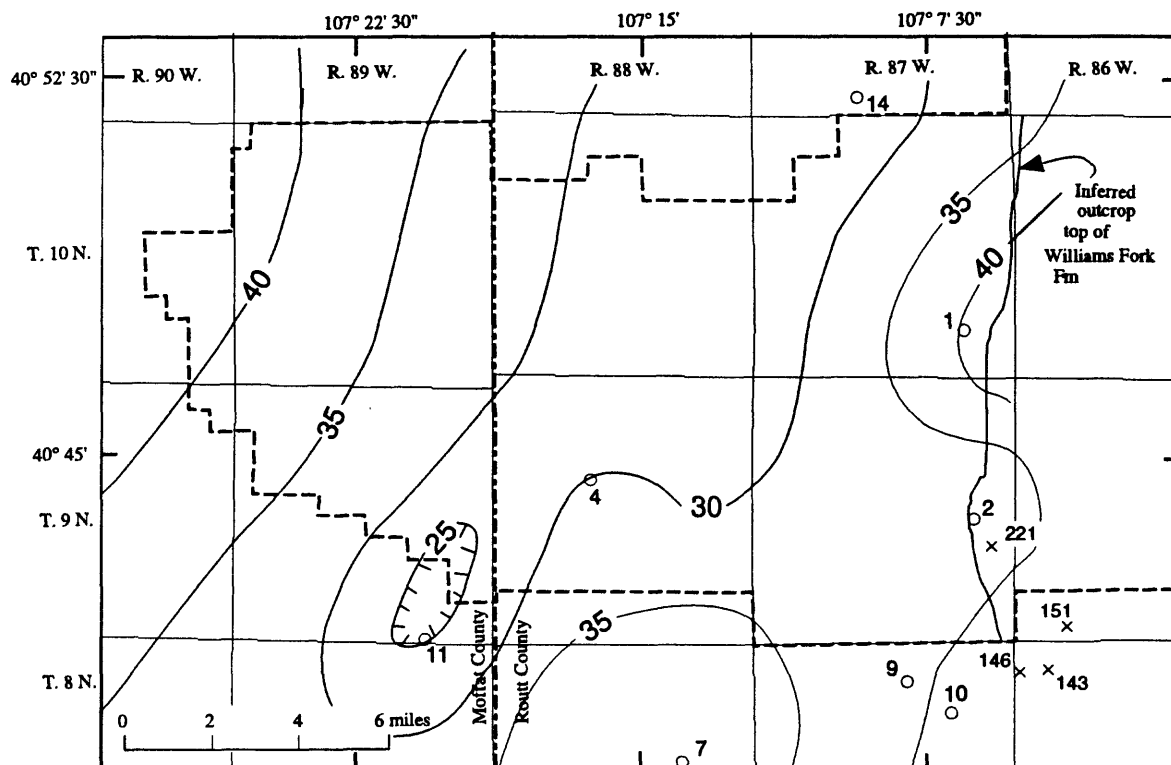
Figure 31a. Isopach map of overburden; datum is top of Williams Fork Formation in and near Area 1, including coals of the middle coal group and of the upper coal group (terminology of Bass and others, 1955). Thickness values are in feet. Hachures indicate area of local thinning.
