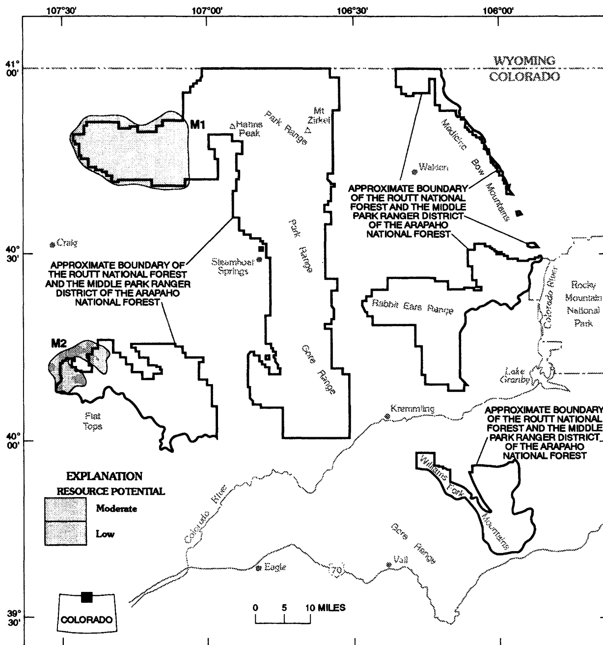
Figure 37. Energy resource map for coalbed methane gas accumulations (M) in the Routt National Forest and Middle Park Ranger District of the Arapaho National Forest, Colorado.
