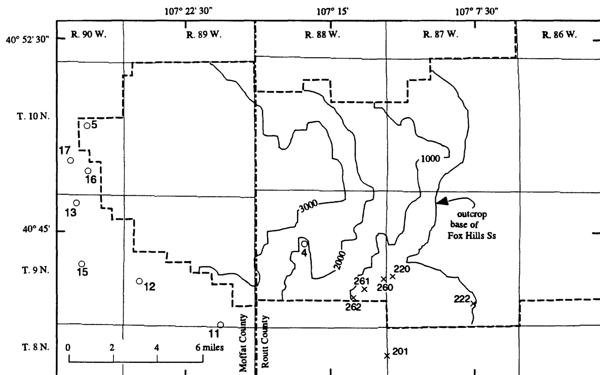
Figure 32b. Isopach map of overburden; datum is base of Lance Formation (top of Fox Hills Sandstone) in Area 1. Thickness values are in feet. Drill holes represented by (o) and number, measured outcrop sections by (x) and number. See table 2 for the location and source data for the drill holes; see table 3 for the location, thickness, and source data for measured sections.
