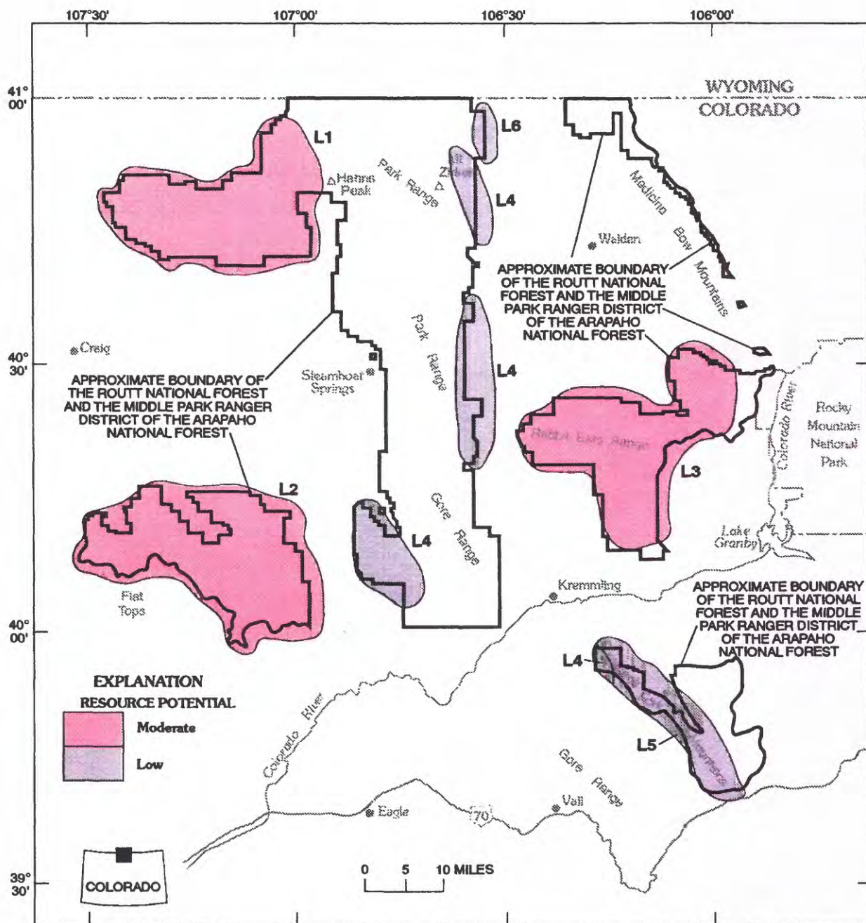
Figure 36. Energy resource map for conventional and subthrust oil gas accumulations (L) in the Routt National Forest and Middle Park Ranger District of the Arapaho National Forest, Colorado.
