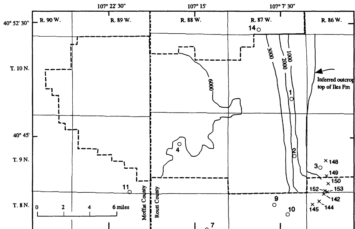
Figure 30b. Isopach map of overburden; datum is top of Iles Formation in Area 1. Thickness values are in feet.
