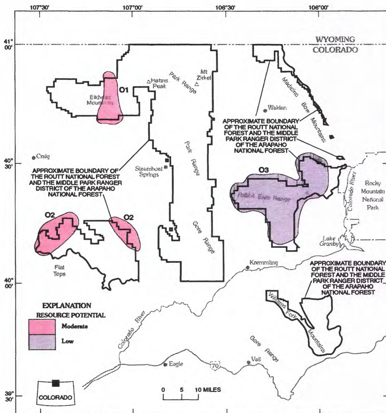
Figure 39. Energy resource map for fractured shale oil accumulations (O) in the Routt National Forest and Middle Park Ranger District of the Arapaho National Forest, Colorado.
