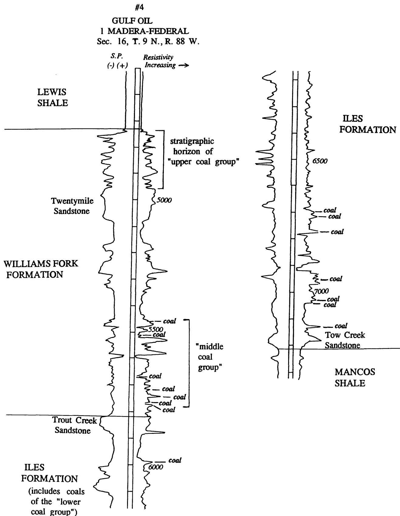
Figure 28. Spontaneous potential (S.P.) and resistivity log signatures of Upper Cretaceous stratigraphic units in Area 1, showing the "lower coal group" of the Iles Formation and the "middle coal group" and "upper coal group" of the Williams Fork Formation (terminology of Bass and others, 1955). In addition to these logs, gamma ray and sonic logs were used to identify coal beds. Log depths are in feet.
