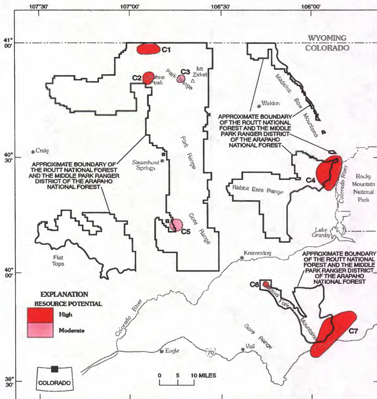
Figure 16. Mineral resource map for polymetallic vein deposits (C) in the Routt National Forest and Middle Park Ranger District of the Arapaho National Forest, Colorado
