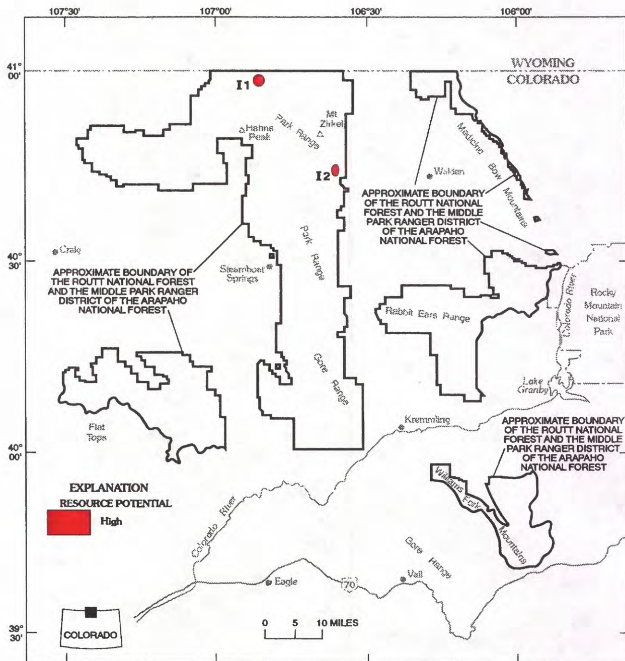
Figure 22. Mineral resource map for PGE in ultramafic rocks (I) in the Routt National Forest and Middle Park Ranger District of the Arapaho National Forest, Colorado
