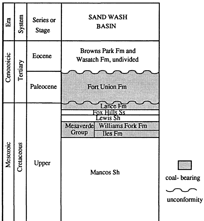
Figure 27. Stratigraphic units in and near Area 1, in the eastern part of the Sand Wash basin.
