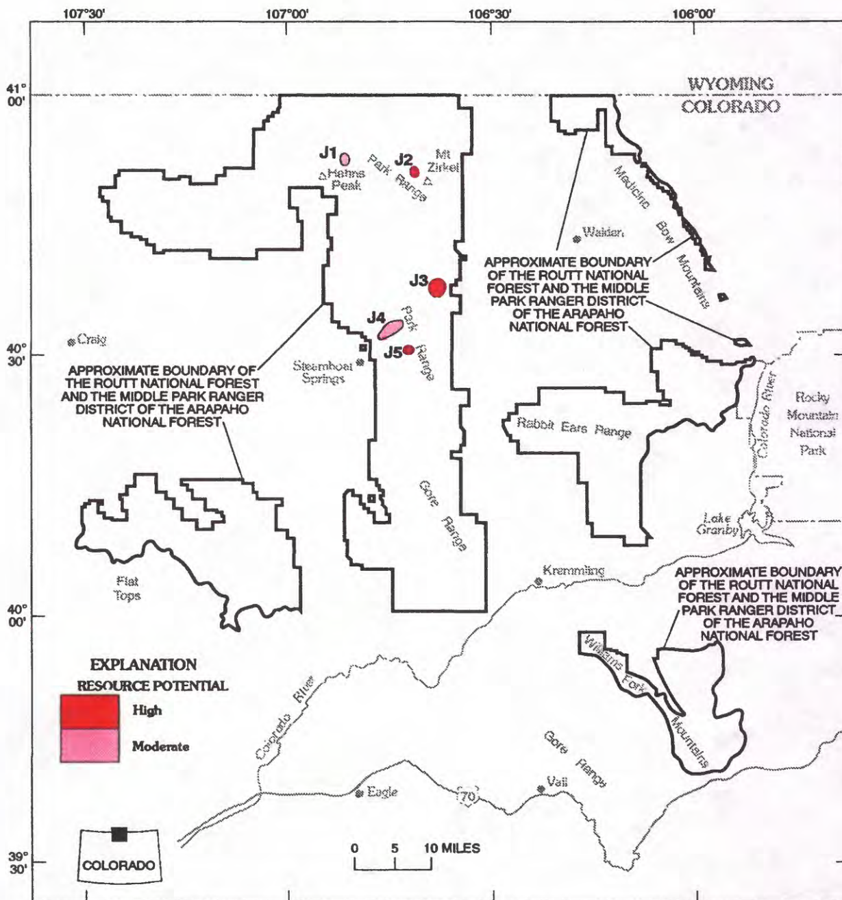
Figure 23. Mineral resource map for U-Th-REE (J) in the Routt National Forest and Middle Park Ranger District of the Arapaho National Forest, Colorado.
