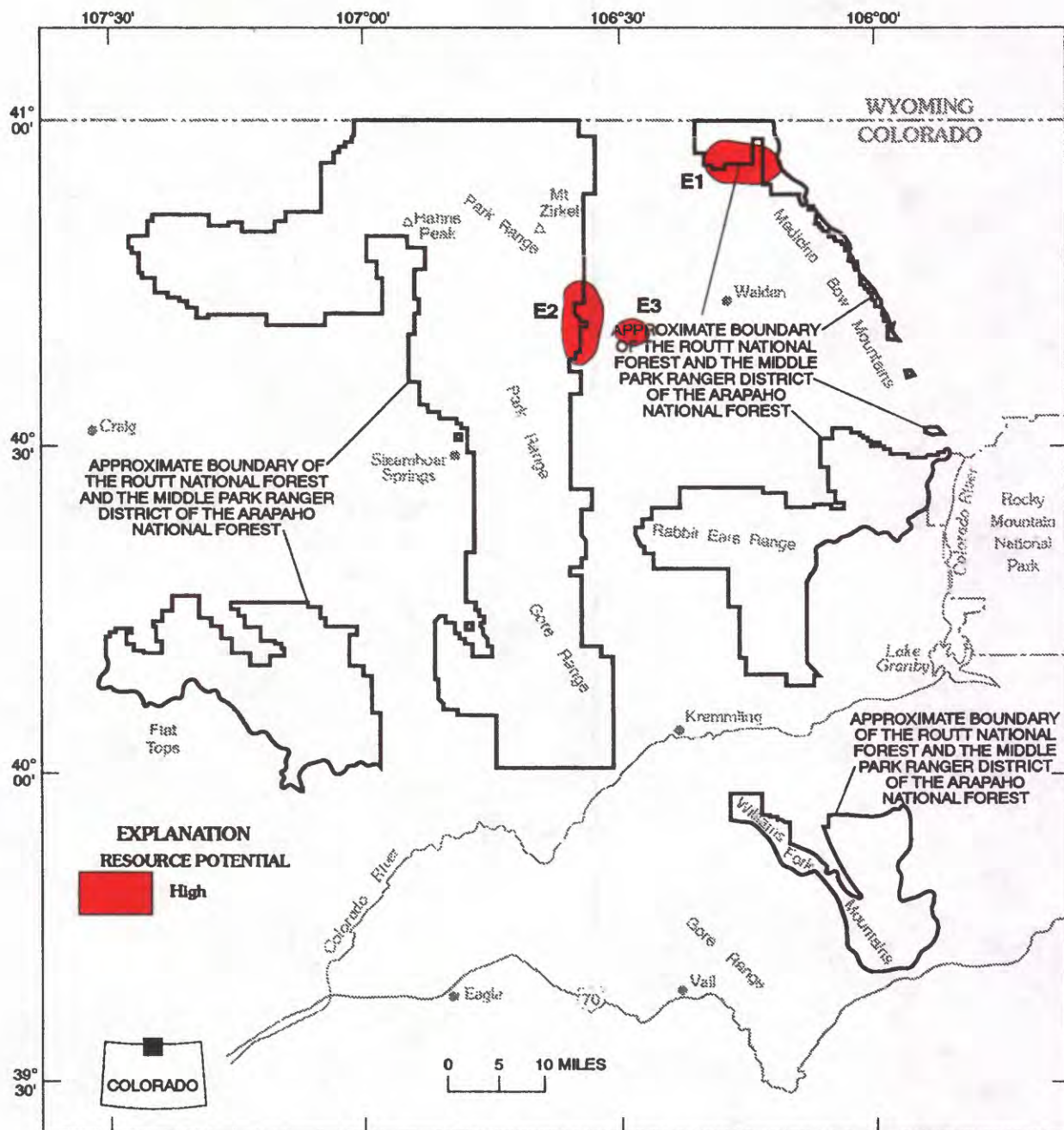
Figure 18. Mineral resource map for fluorsspar veins and dissemination deposits (E) in the Routt National Forest and Middle Park Ranger District of the Arapaho National Forest, Colorado
