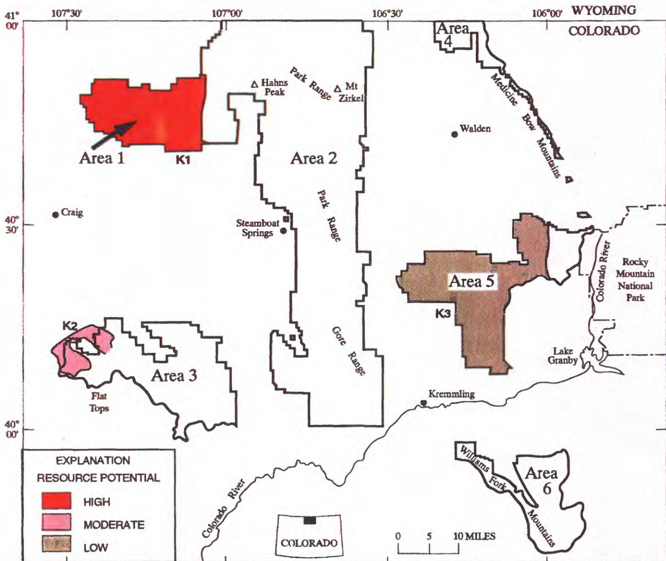
Figure 34. Map showing coal resource potential of areas underlain by coal-bearing Upper Cretaceous and Tertiary stratigraphic units, Routt National Forest. Forest areas shown by heavy outline.
