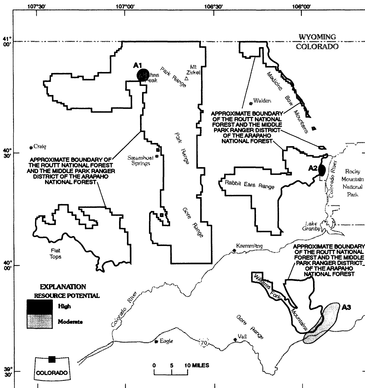
Figure 14. Mineral resource map for stockwork molybdenum deposits (A) in the Routt National Forest and Middle Park Ranger District of the Arapaho National Forest, Colorado
