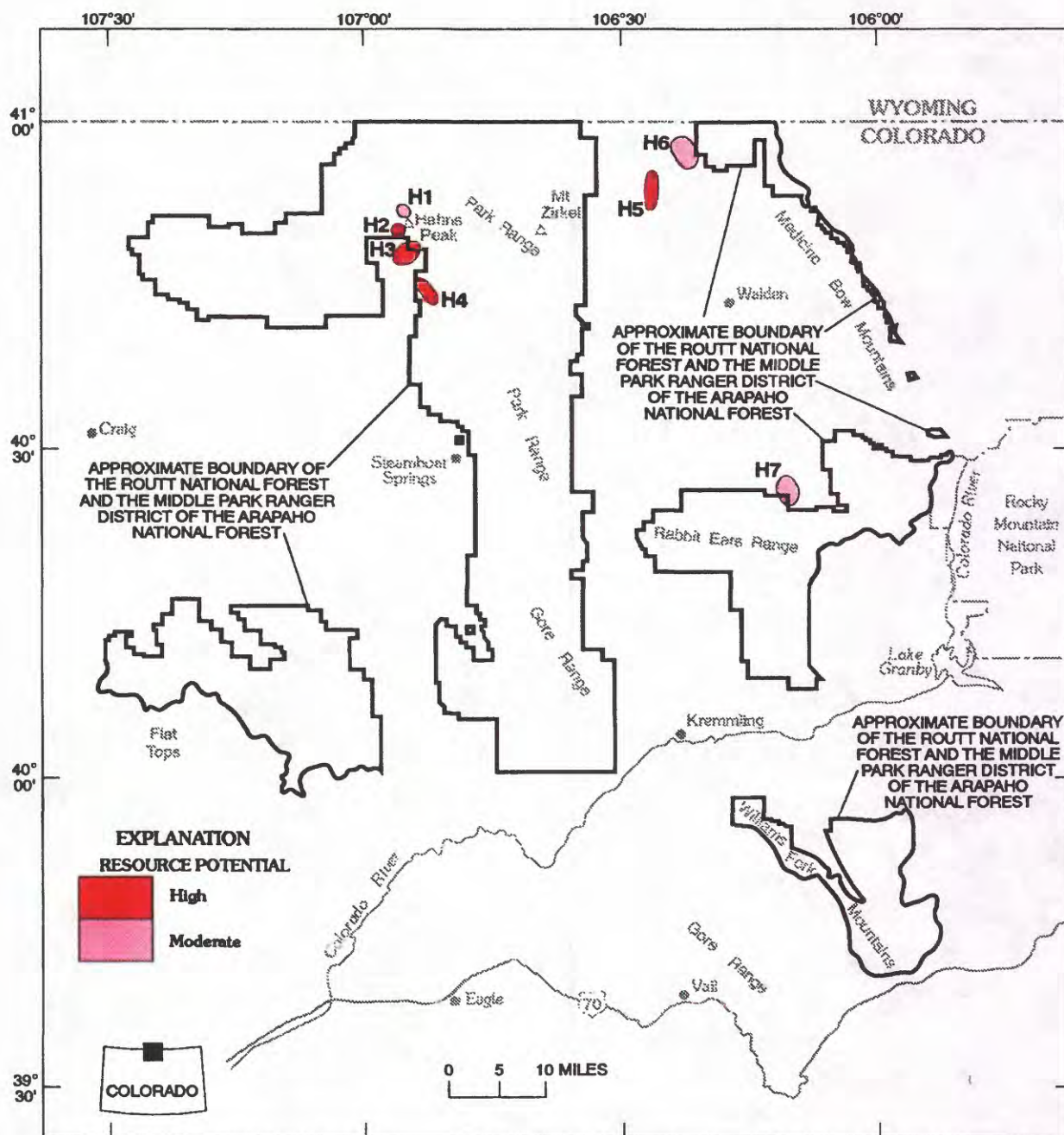
Figure 21. Mineral resource map for placer gold (H) in the Routt National Forest and Middle Park Ranger District of the Arapaho National Forest, Colorado.
