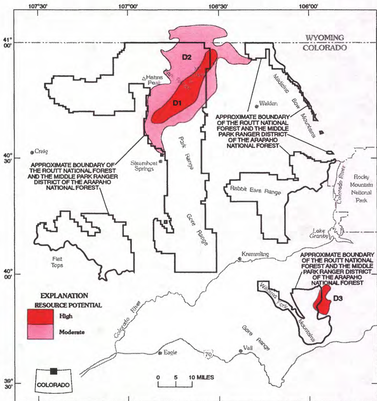
Figure 17. Mineral resource map for stratabound massive sulfide deposits (D) in the Routt National Forest and Middle Park Ranger District of the Arapaho National Forest, Colorado
