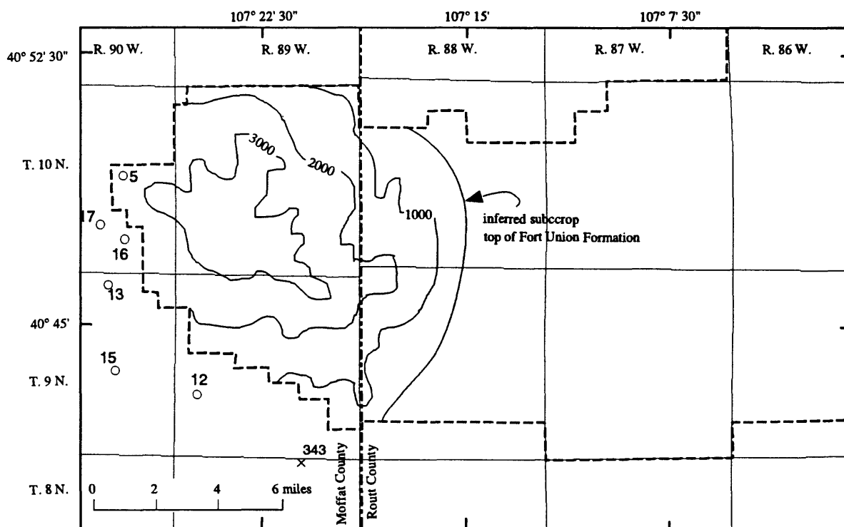
Figure 33b. Isopach map of overburden; datum is top of Fort Union Formation in Area 1. Thickness values are in feet. Drill holes represented by (o) and number, measured outcrop sections by (x) and number. See table 2 for the location and source data for drill holes; see table 3 for the location, thickness, and source data for measured sections.
