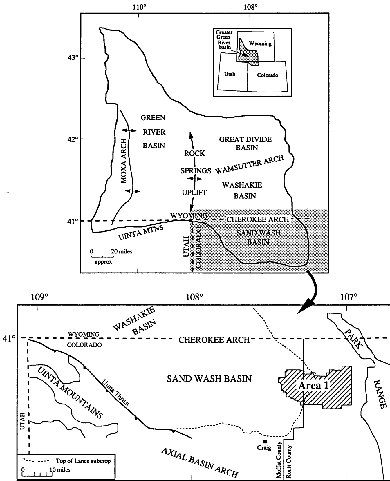
Figure 25. Structural setting of Area 1 in the southeastern part of the Sand Wash basin of the Greater Green River basin. Sawteeth on upper plate of thrust fault.
