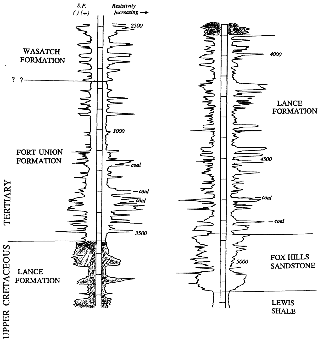
Figure 29. Spontaneous potential (S.P.) and resistivity log signatures of Upper Cretaceous and Tertiary stratigraphic units in Area 1, showing coal beds in the Lance Formation and in the Fort Union Formation. Shaded interval is the "unnamed Cretaceous-Tertiary sandstone unit" of Honey and Hettinger (1989). In addition to these logs, gamma ray and sonic logs were used to identify coal beds. Log depths are in feet.
