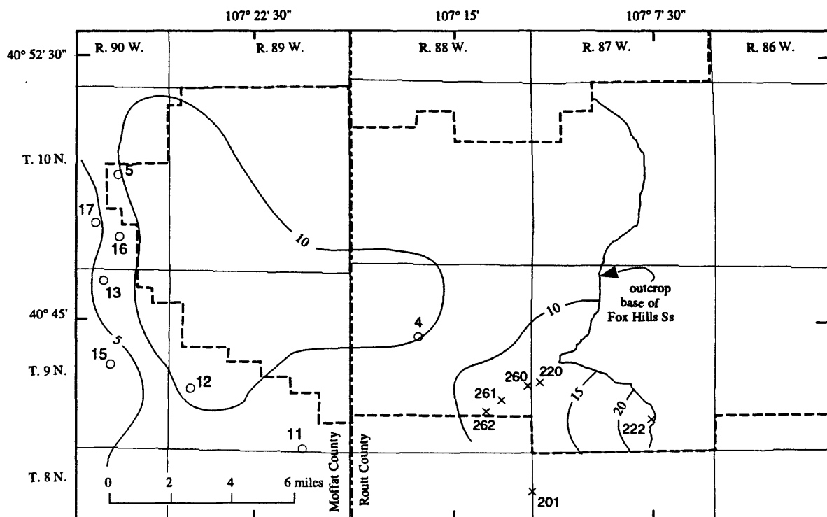
Figure 32a. Isopach map of cumulative coal in the Lance Formation, in and near Area 1. Thickness values are in feet.
