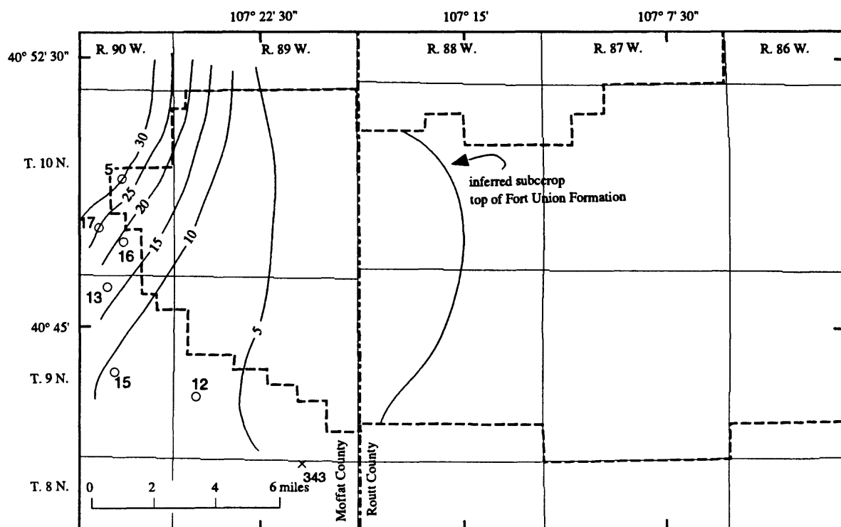
Figure 33a. Isopach map of cumulative coal in the Fort Union Formation, in and near Area 1. Thickness values are in feet.
