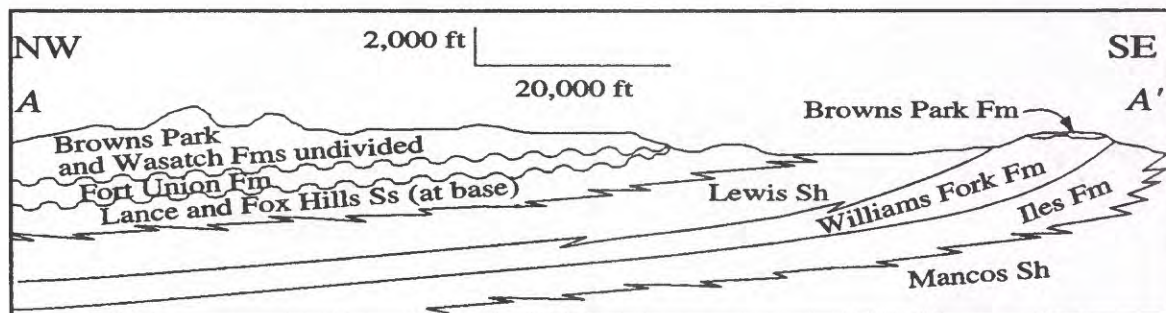
Figure 26. Generalized geologic map showing Late Cretaceous sedimentary rocks and Tertiary sedimentary, volcanic, and intrusive rocks in and near Area 1. (Modified from Tweto, 1976). Generalized cross section A-A' of Late Cretaceous through Tertiary sedimentary rocks in Area 1. An unconformity lies at the base of the Wasatch and Fort Union Formations. See figure 1 for location of Area 1.
