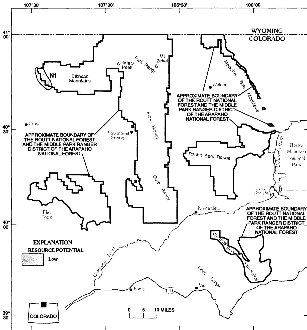
Figure 38. Energy resource map for basin centered gas accumulations (N) in the Routt National Forest and Middle Park Ranger District of the Arapaho National Forest, Colorado.
