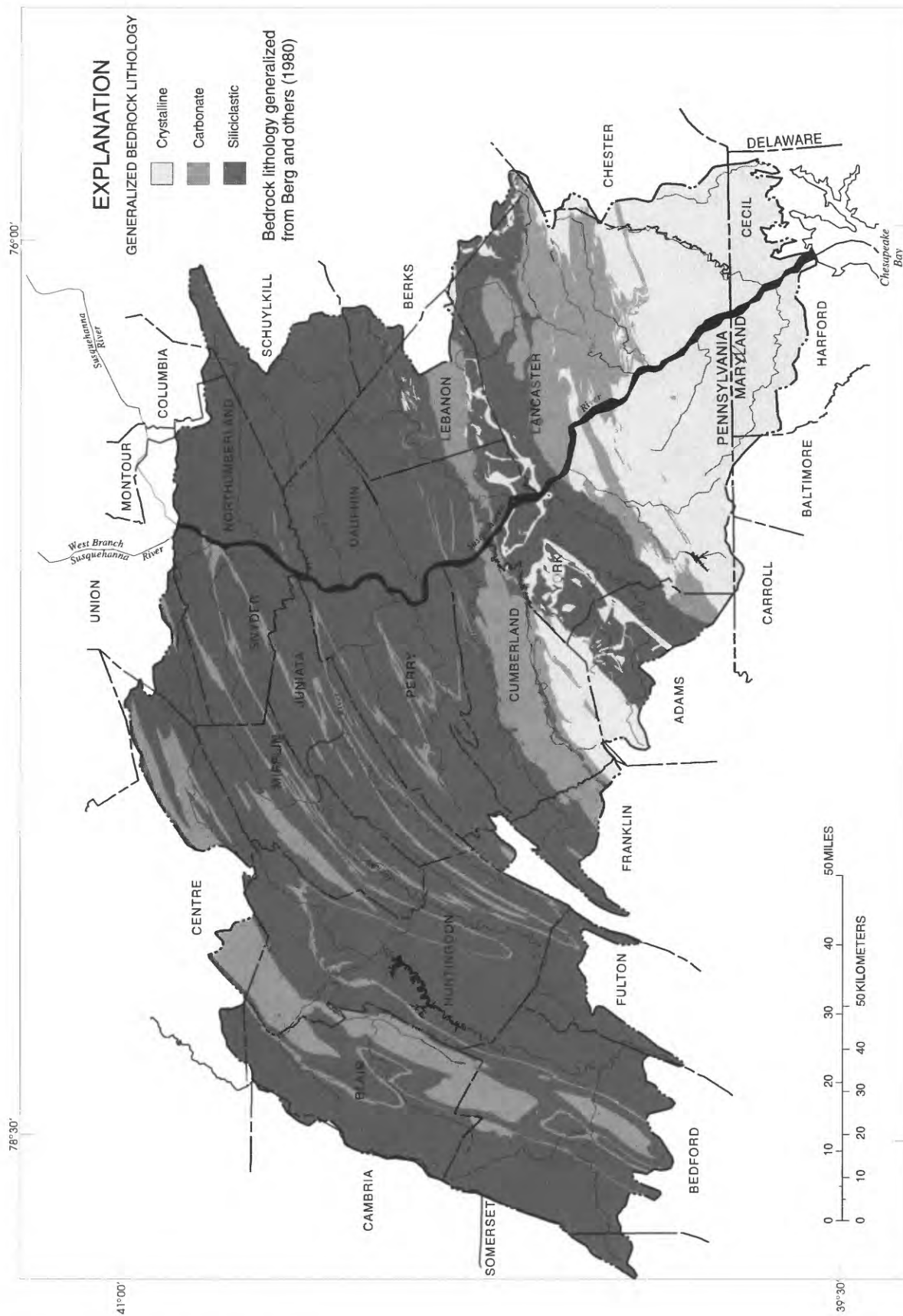
Figure 3. Generalized bedrock lithology in the Lower Susquehanna NAWQA study unit.
