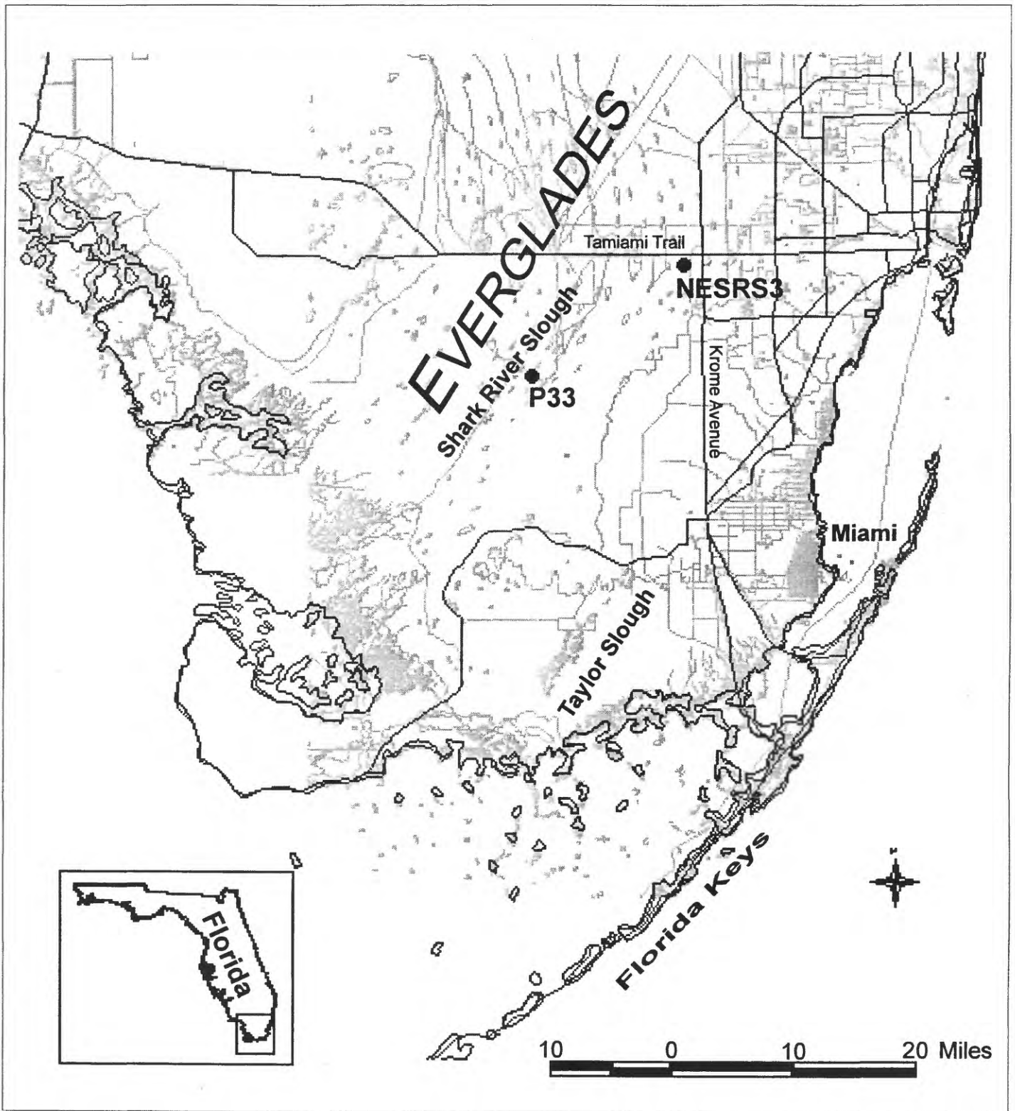
Figure 1. Site map showing the locations of sites P33 and NESRS3.
