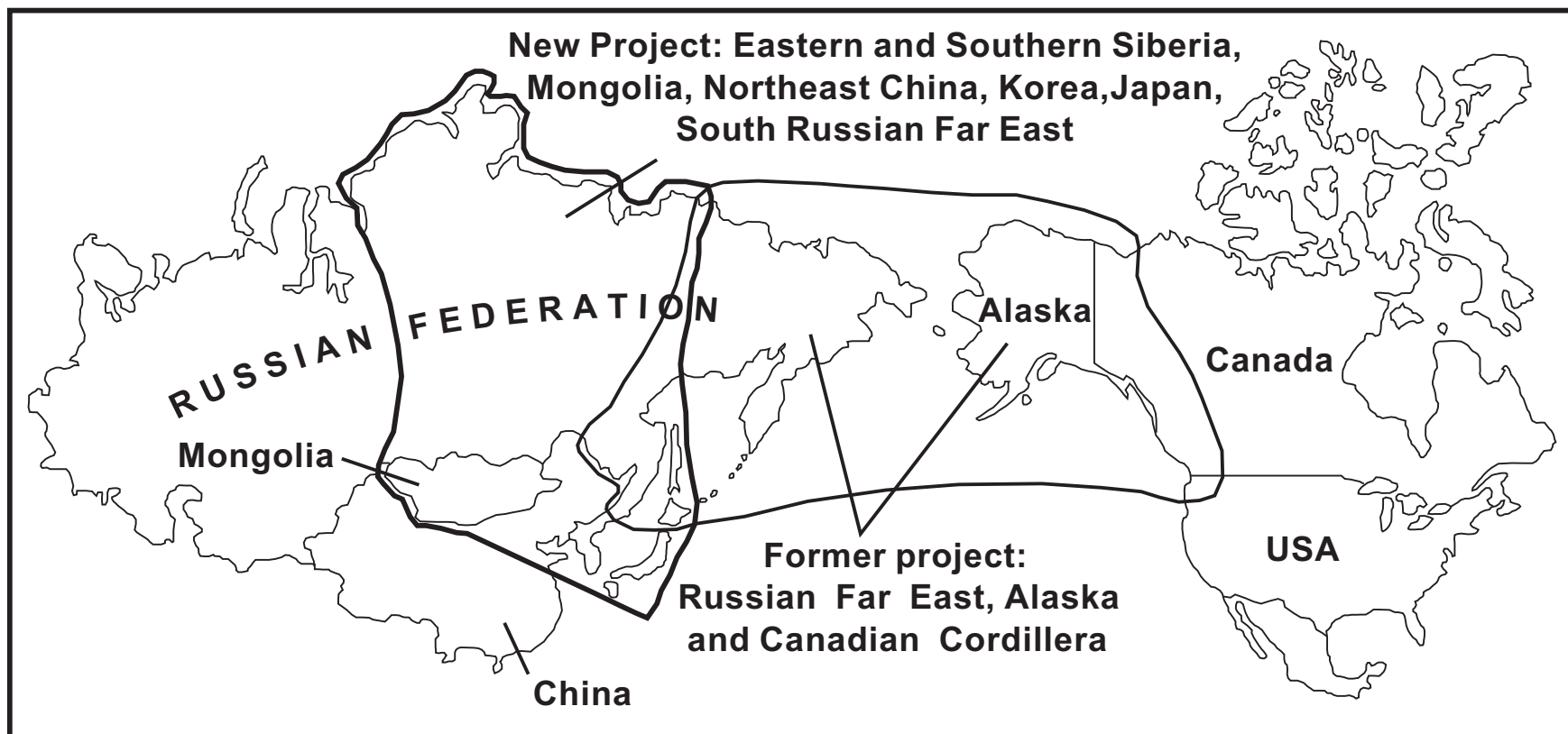
Figure 1. Areas covered by the previous project on metallogensis and tectonics of the Circum-North Pacific and the new project on metallogensis and tectonics of Northeast Asia.
