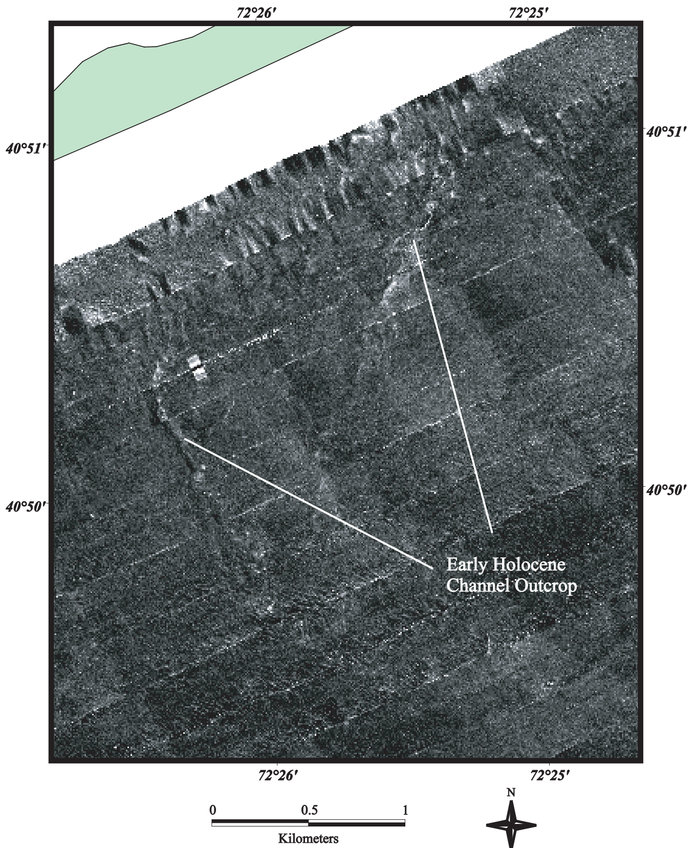
Figure 5. Sidescan-sonar image showing filled paleochannels exposed on the seafloor. These paleochannels are cut into the Pleistocene sedimentary deposit and filled with an early Holocene transgressional sequence. High backscatter is represented by light tones, low backscatter is represented by dark tones within the image. See Figure 2b for location.
