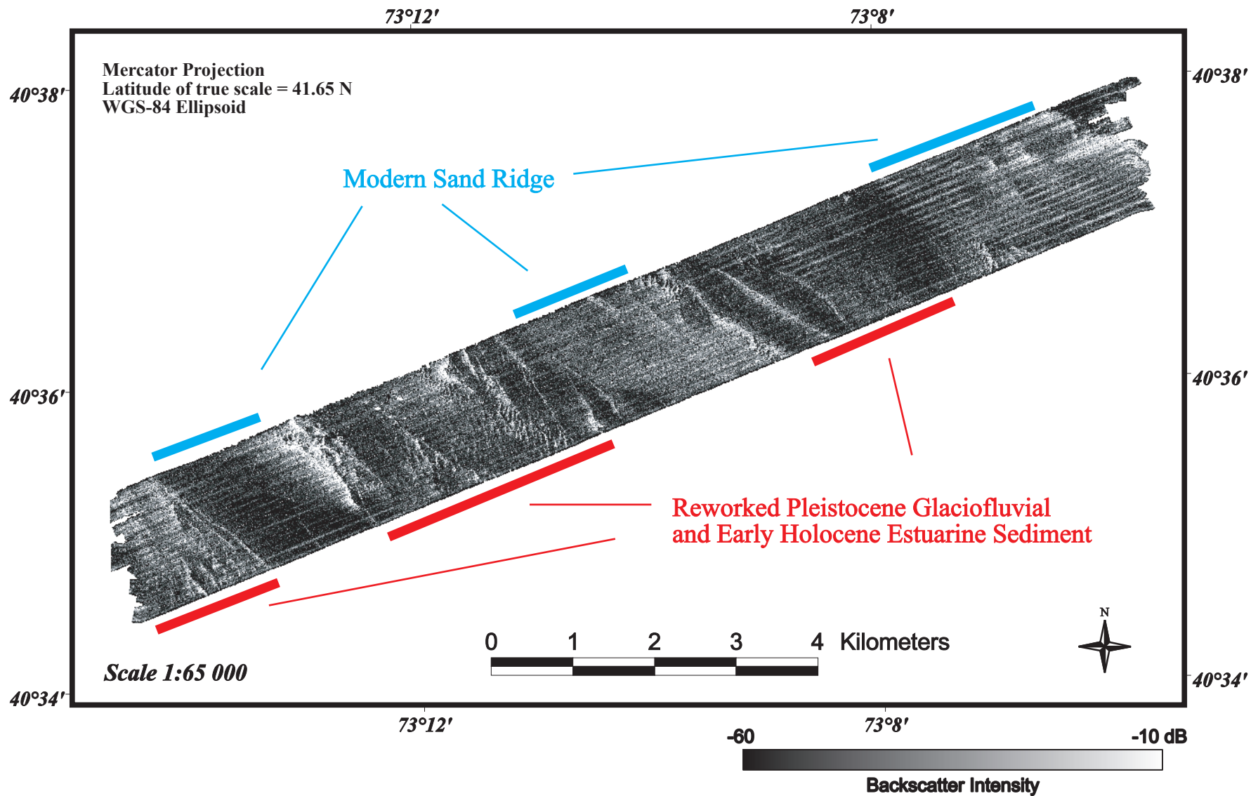
Figure 6a. Simrad EM 1000 Echo Sounder backscatter image of the shoreface-attached sand ridges west of Watch Hill. Light tones depict areas of high backscatter, dark tones areas of low backscatter within the image. See Figure 2b for location.
