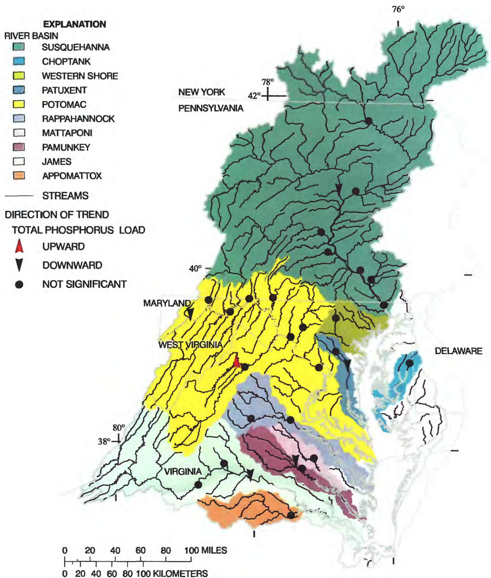
Figure 3B. Trends in load for total phosphorus.
