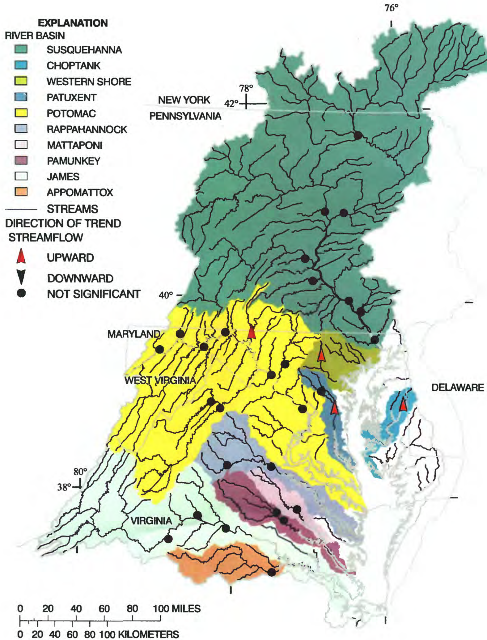
Figure 2. Trends in streamflow, 1985-99.
