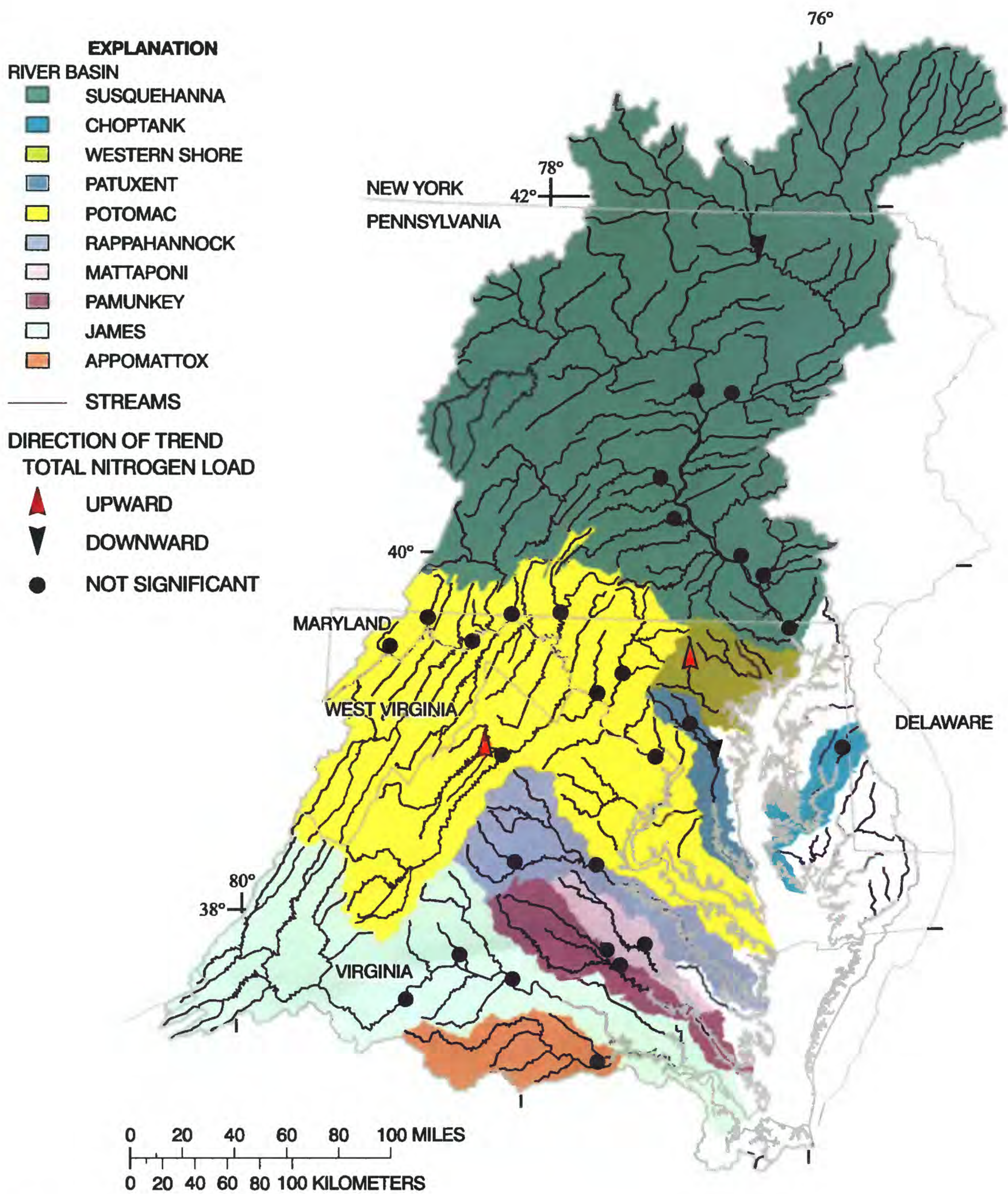
Figure 3A. Trends in load for total nitrogen.
