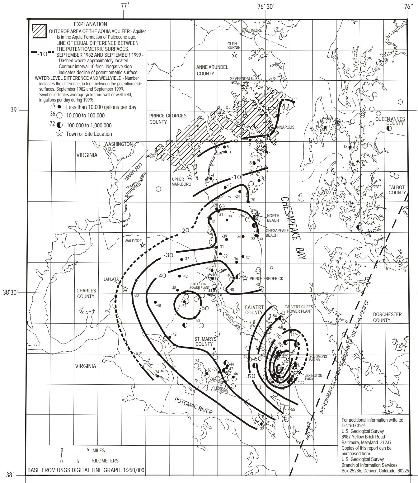
THE DIFFERENCE BETWEEN THE POTENTIOMETRIC SURFACES OF THE AQUIA AQUIFER, SEPTEMBER 1982 AND SEPTEMBER 1999 IN SOUTHERN MARYLAND
