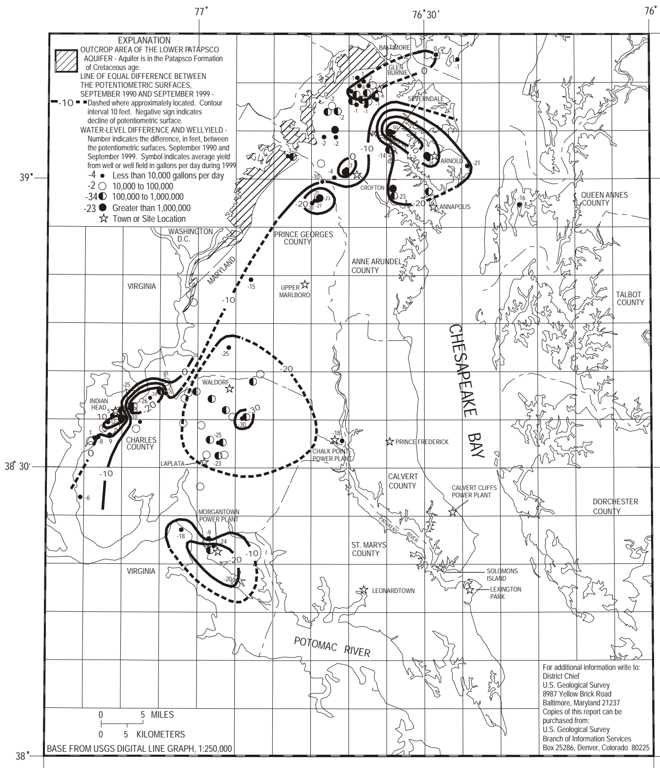
THE DIFFERENCE BETWEEN THE POTENTIOMETRIC SURFACES OF THE LOWER PATAPSCO AQUIFER, SEPTEMBER 1990 AND SEPTEMBER 1999 IN SOUTHERN MARYLAND
