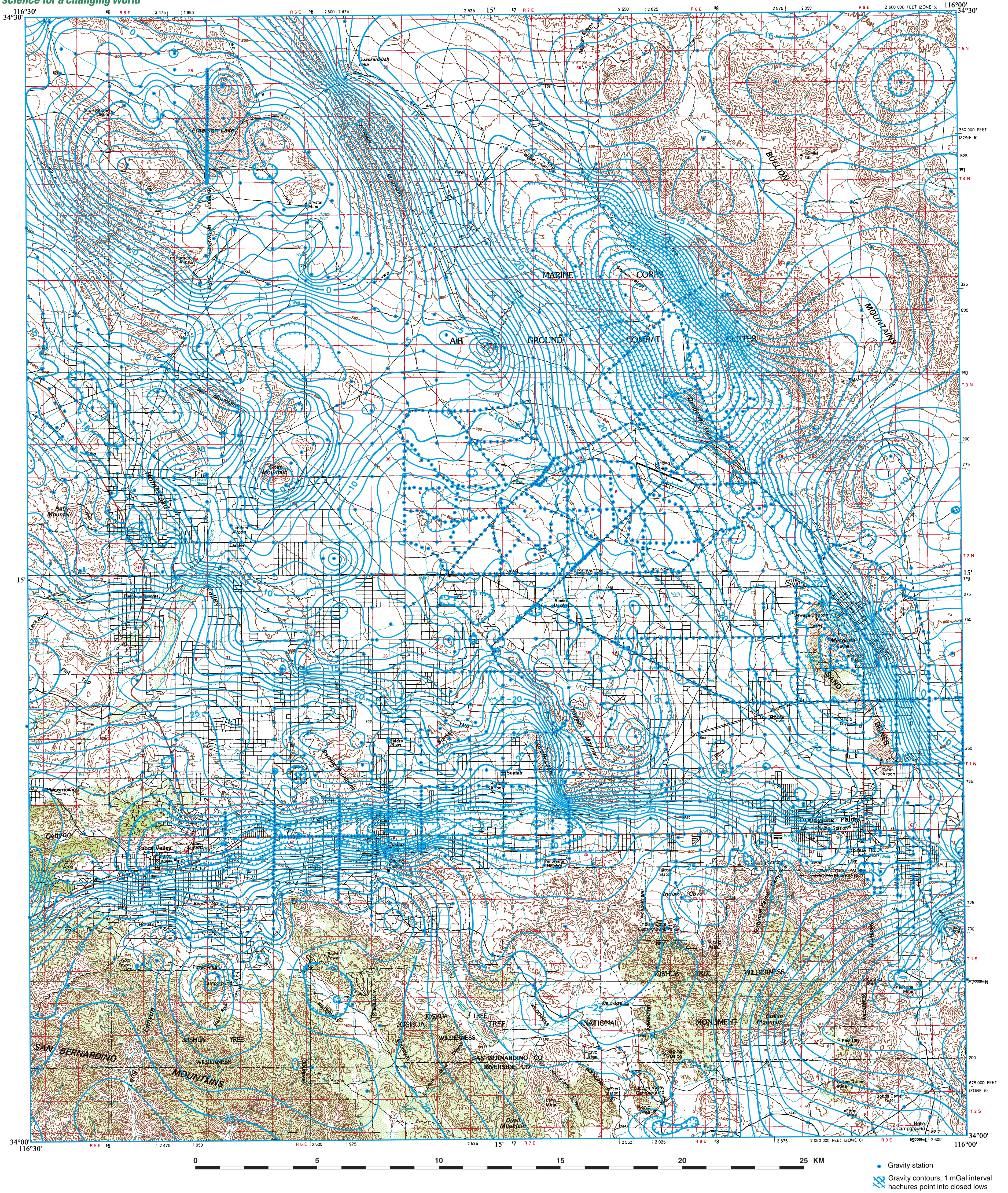
Isostatic residual gravity map of the eastern half of the Big Bear Lake 1:100,000 scale quadrangle.
