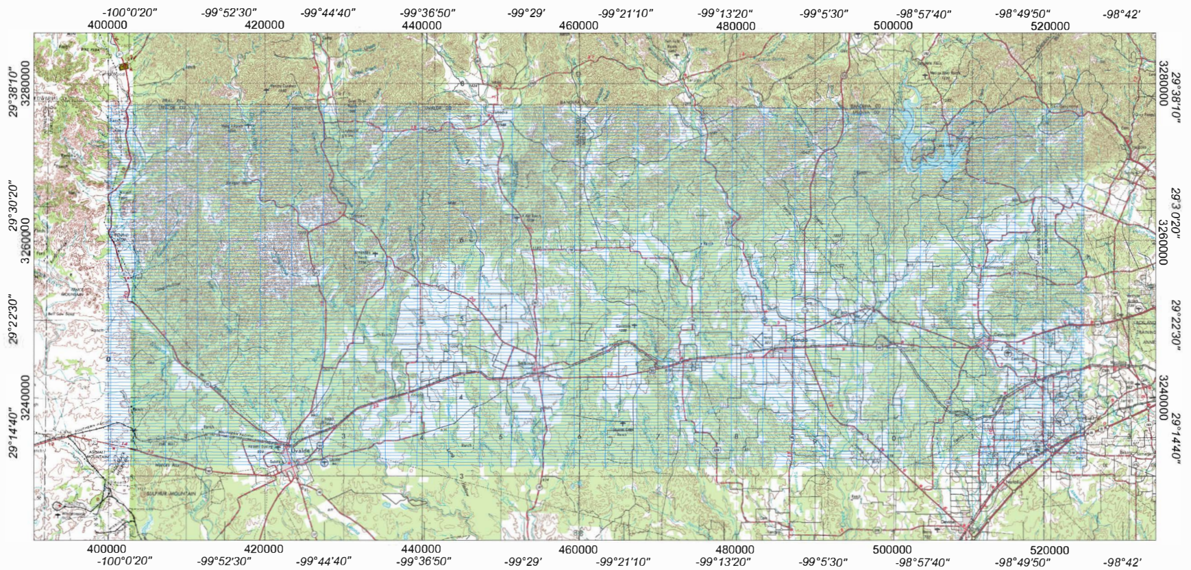
Aeromagnetic Survey Flight Lines
