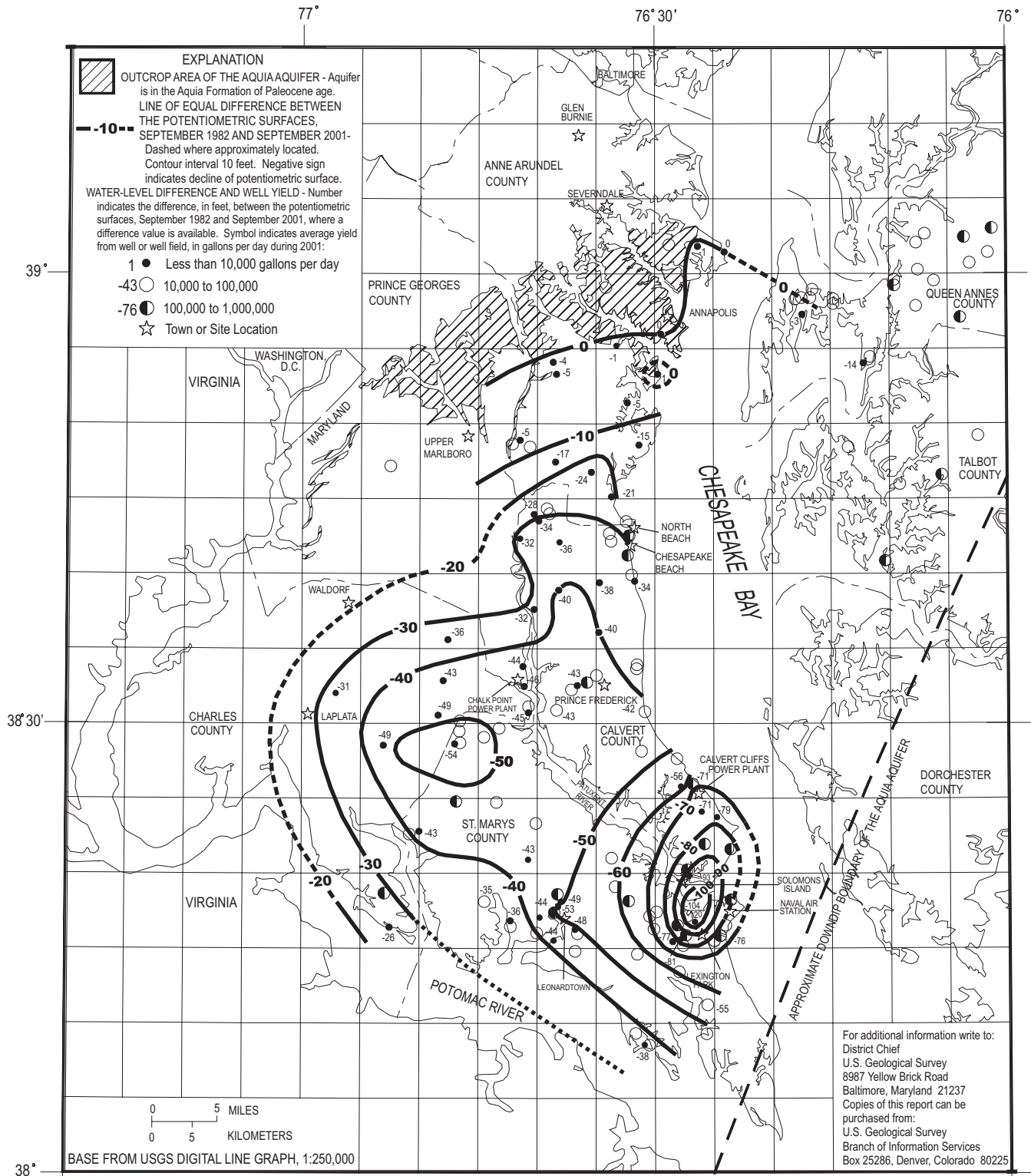
THE DIFFERENCE BETWEEN THE POTENTIOMETRIC SURFACES OF THE AQUIA AQUIFER, SEPTEMBER 1982 AND SEPTEMBER 2001 IN SOUTHERN MARYLAND
