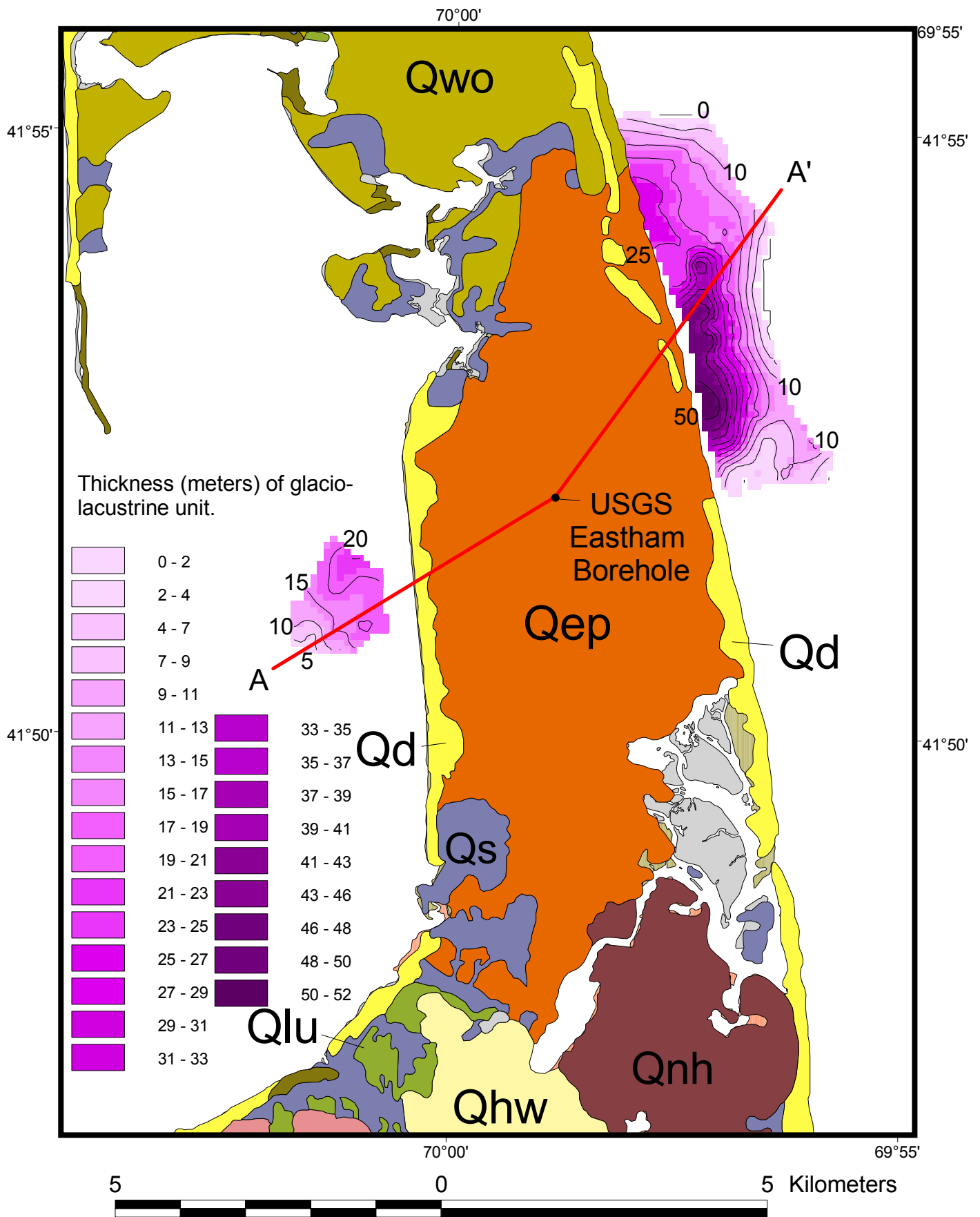
Figure 10. Map showing the thickness (meters) of glaciolacustrine (Qdl). Location of cross section A (Fig. 13) shown with red line. Surficial geologic units are described in figure 3.
