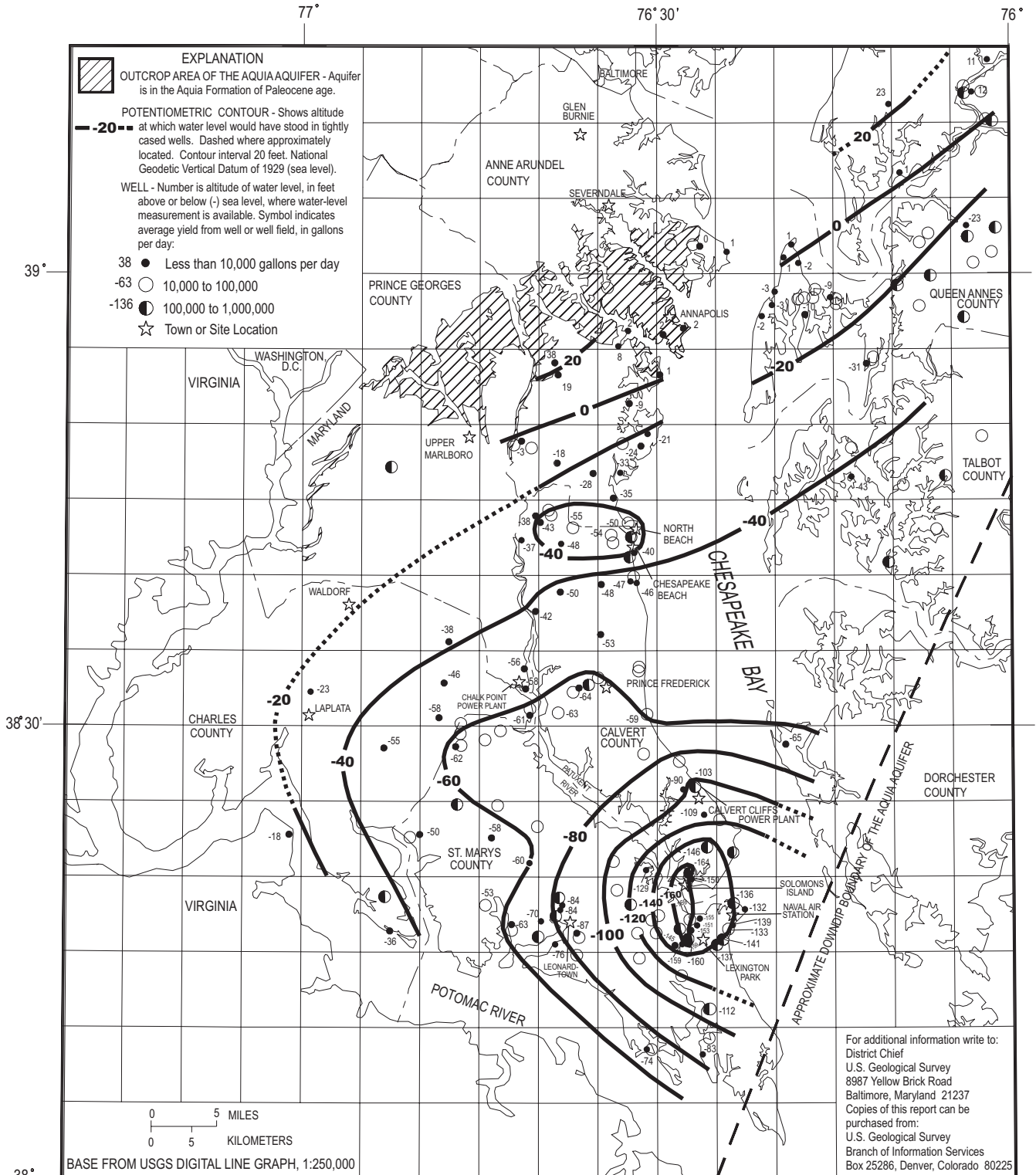
POTENTIOMETRIC SURFACE OF THE AQUIA AQUIFER IN SOUTHERN MARYLAND,
