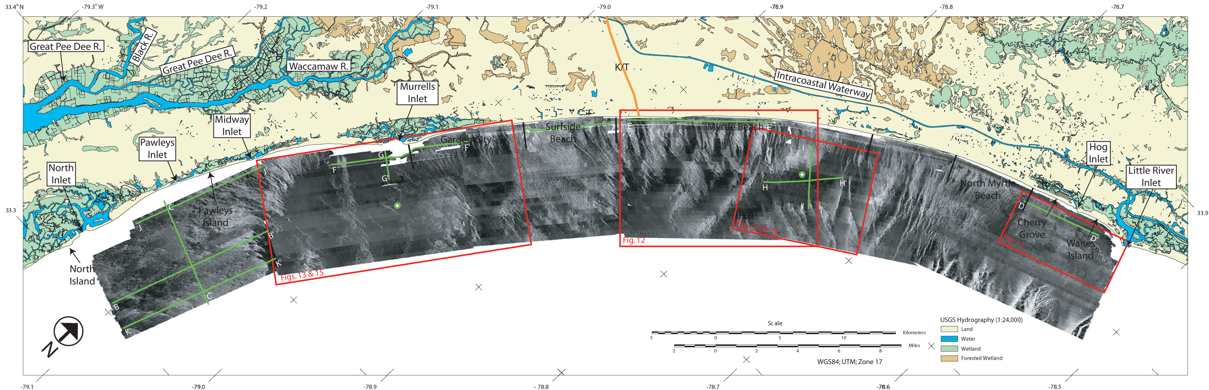
Figure 7. SIS-1000 100 kHz sidescan-sonar image of the study area. Light tones depict areas of high backscatter and dark tones indicate areas of low backscatter. Inset numbered boxes indicate the locations of figures within the text. Green lines indicate trackline coverage of sub-bottom profiles and green circled white crosses indicate groundtruth locations used for illustration.
