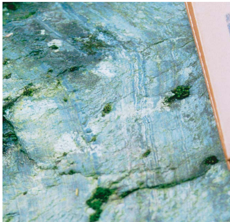
Fig. 9B Early laminations, parallel to edge of notebook, are vertical beds that strike north-south into the faults along the Little River. These rocks are located in the Wear Cove, Tenn., 7.5-minute quadrangle.
