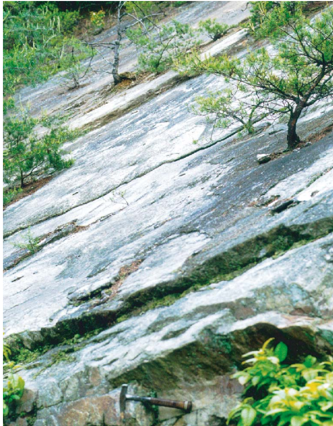
Fig. 32 Southeast-dipping beds of Hesse Quartzite (Ch) form the dip slope to the homoclinal ridge of Chilhowee Mountain, where the Foothills Parkway transects it. Pine trees thrive in cracks in the rocks that are well drained and acidic. Rock hammer in lower center of photo for scale.
