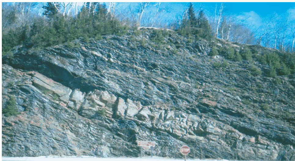
Fig. 19A Southeast-dipping beds at the intersection of Route 441 and the road to Clingmans Dome. Stop sign in lower center for scale.
