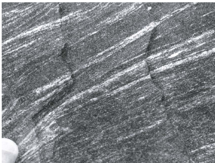
Fig. 3B Mafic rocks are foliated amphibolite (Ya) near Dellwood, in the Dellwood, N.C., 7.5-minute quadrangle. This photograph is of a small part of a body that is 900 ft wide and 2,000 ft long within hornblende-biotite gneiss. Fingertip for scale.
