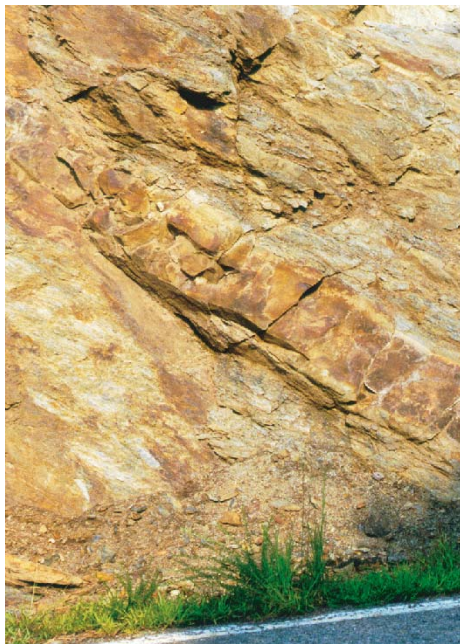
Fig. 26B Metasandstone and metaconglomerate beds within the schist dip to the lower right of the photo. Roadcut is about 10 ft high and is located in the Bryson City, Tenn.-N.C., 7.5-minute quadrangle.
