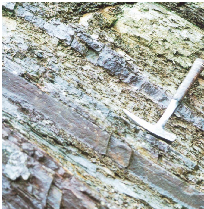
Fig. 31B Thin beds of sandstone occur within the shale, just as thin beds of shale also occur within the overlying quartzite units. Outcrop is at Chilogatee Gap in the Blockhouse, Tenn., 7.5-minute quadrangle.
