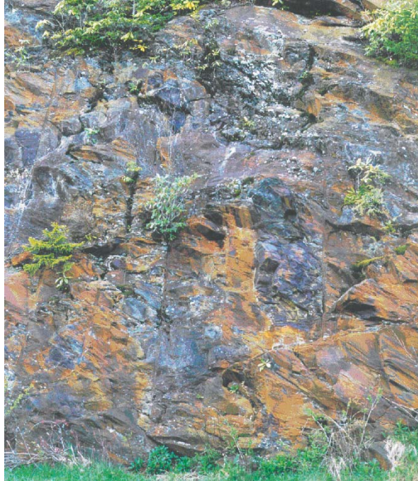
Fig. 18A Slate, sandy slate, and metasandstone exposed in a roadcut near Newfound Gap. Roadcut is about 10 ft high.
