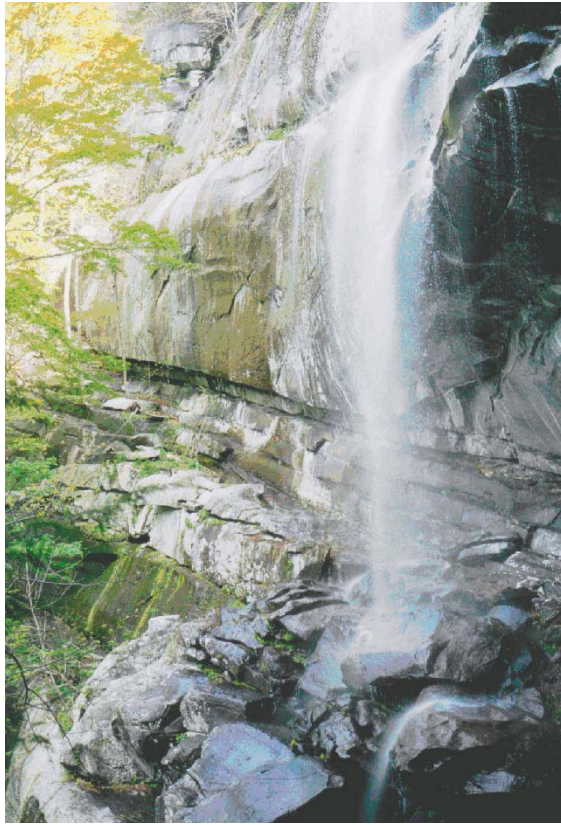
Fig. 12A Thick beds of massive Thunderhead Sandstone form cliffs hundreds of feet high in the north-central part of the park. These are unique habitats mostly due to sprays of water. Height of cliff is about 30 ft.
