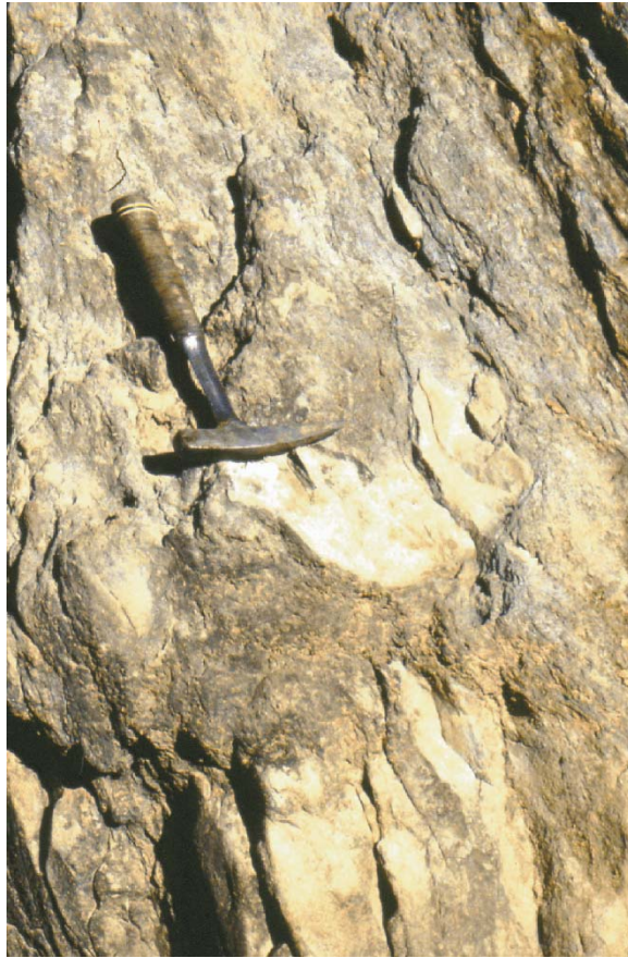
Fig. 35A Foliated greenstone with large body of epidote and quartz (epidosite). Rock hammer for scale.
