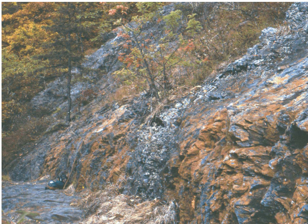
Fig. 14 Dark rusty weathered, sulfidic metasiltstones (Zts) similar to rocks of the Anakeesta Formation are within the Thunderhead Sandstone. Some are thick enough to be portrayed on the map, like these rocks along the Appalachian Trail at Shuckstack, in the Fontana Dam, N.C., 7.5-minute quadrangle.
