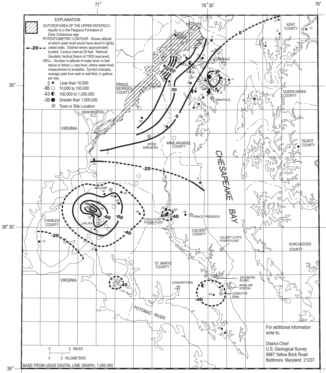
POTENTIOMETRIC SURFACE OF THE UPPER PATAPSCO AQUIFER IN SOUTHERN MARYLAND, SEPTEMBER 2003
