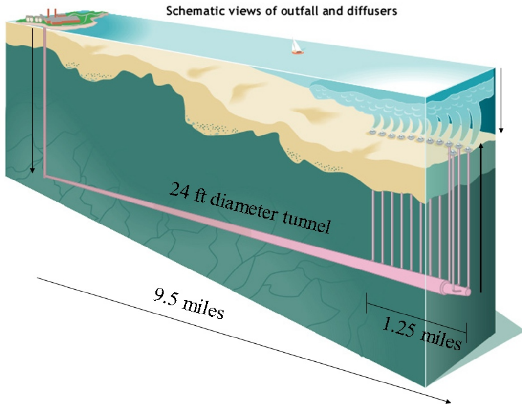
Figure 1.3. The Massachusetts Bay outfall consists of 55 diffuser heads connecting to a tunnel that transports an average of 350 million gallons per day of secondary treated sewage effluent from the Deer Island Treatment plant.
