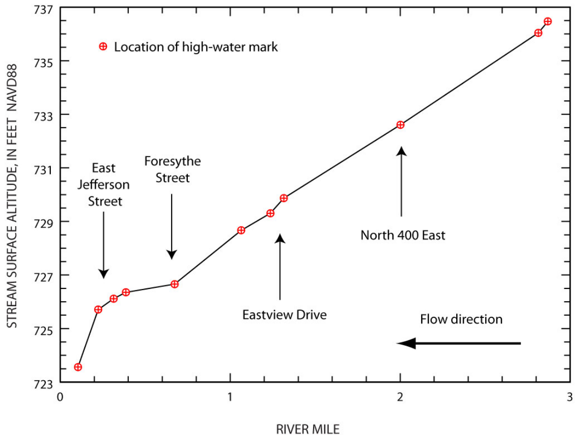
Flood-peak elevation profile, flood of June 7–9, 2008, for Hurricane Creek at Franklin, Indiana.
