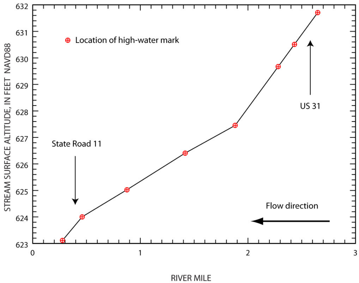
Flood-peak elevation profile, flood of June 7–9, 2008, for Flatrock River at Columbus, Indiana.
