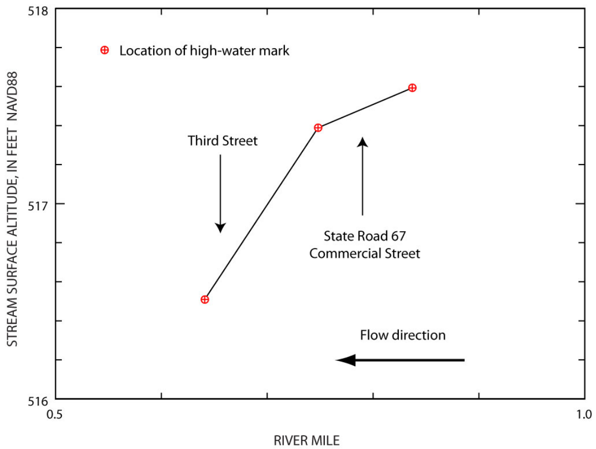
Flood-peak elevation profile, flood of June 7–9, 2008, for Eel River at Worthington, Indiana.
