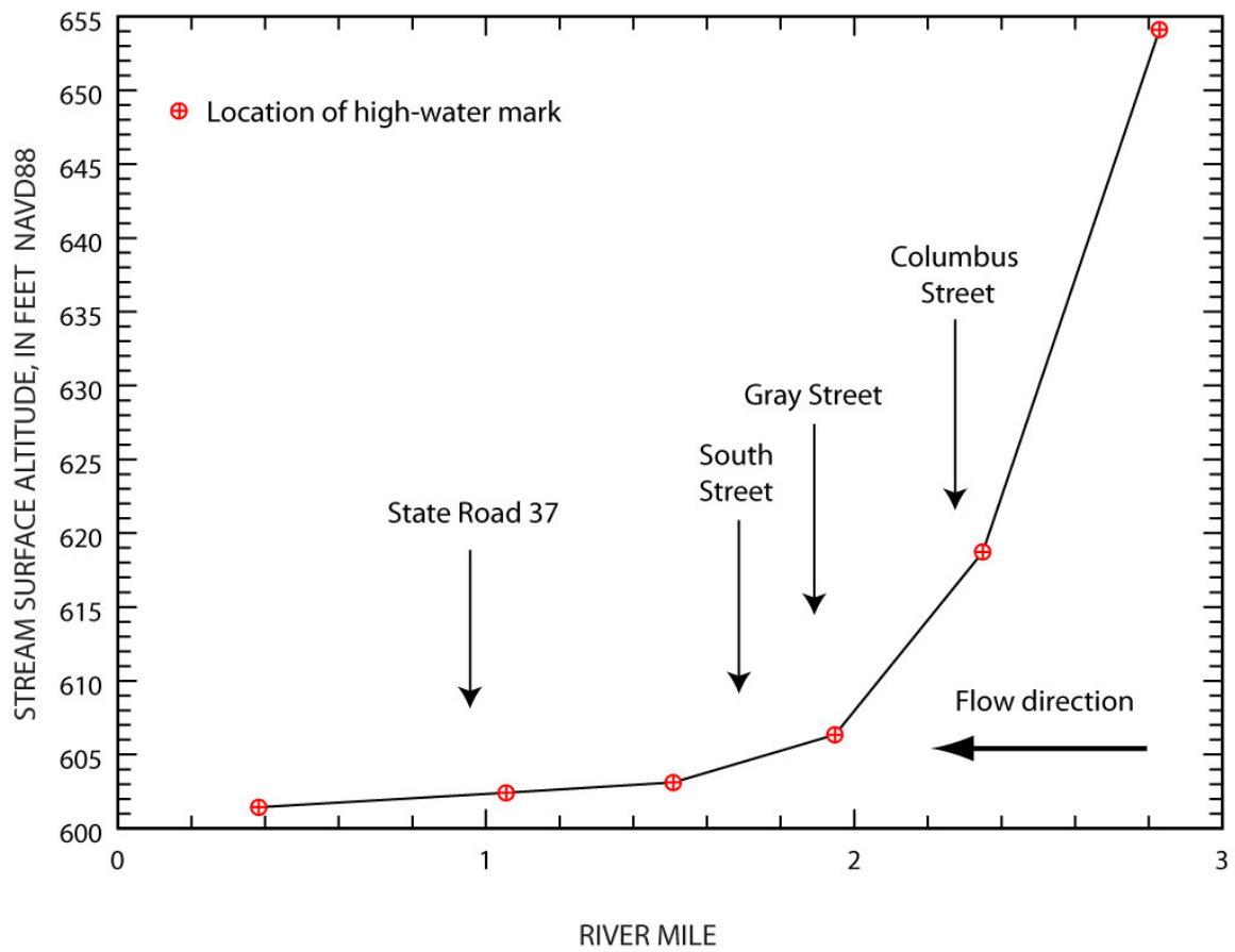
Flood-peak elevation profile, flood of June 7–9, 2008, for Sartor Ditch, Martinsville, Indiana.
