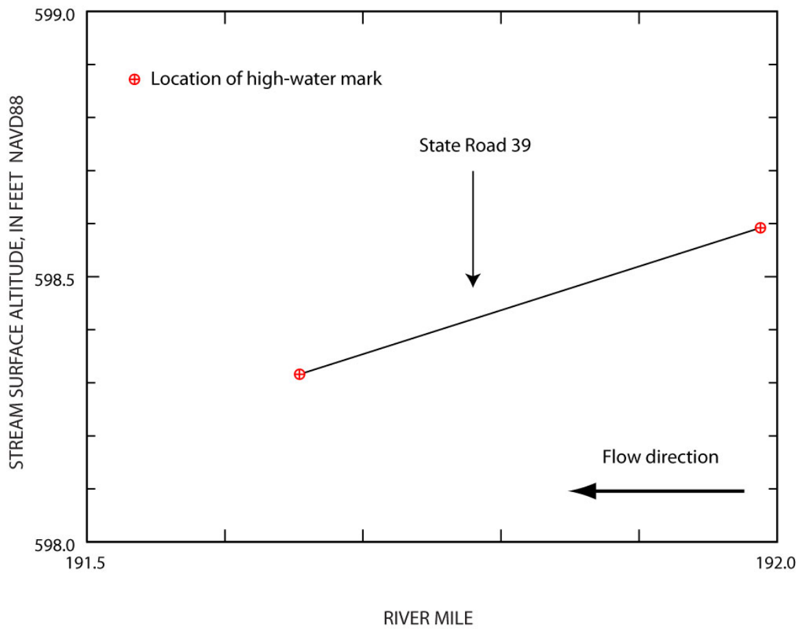
Flood-peak elevation profile, flood of June 7–9, 2008, for White River at Martinsville, Indiana.
