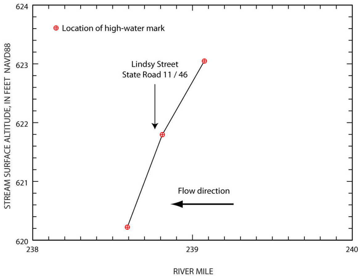
Flood-peak elevation profile, flood of June 7–9, 2008, for East Fork White River at Columbus, Indiana.
