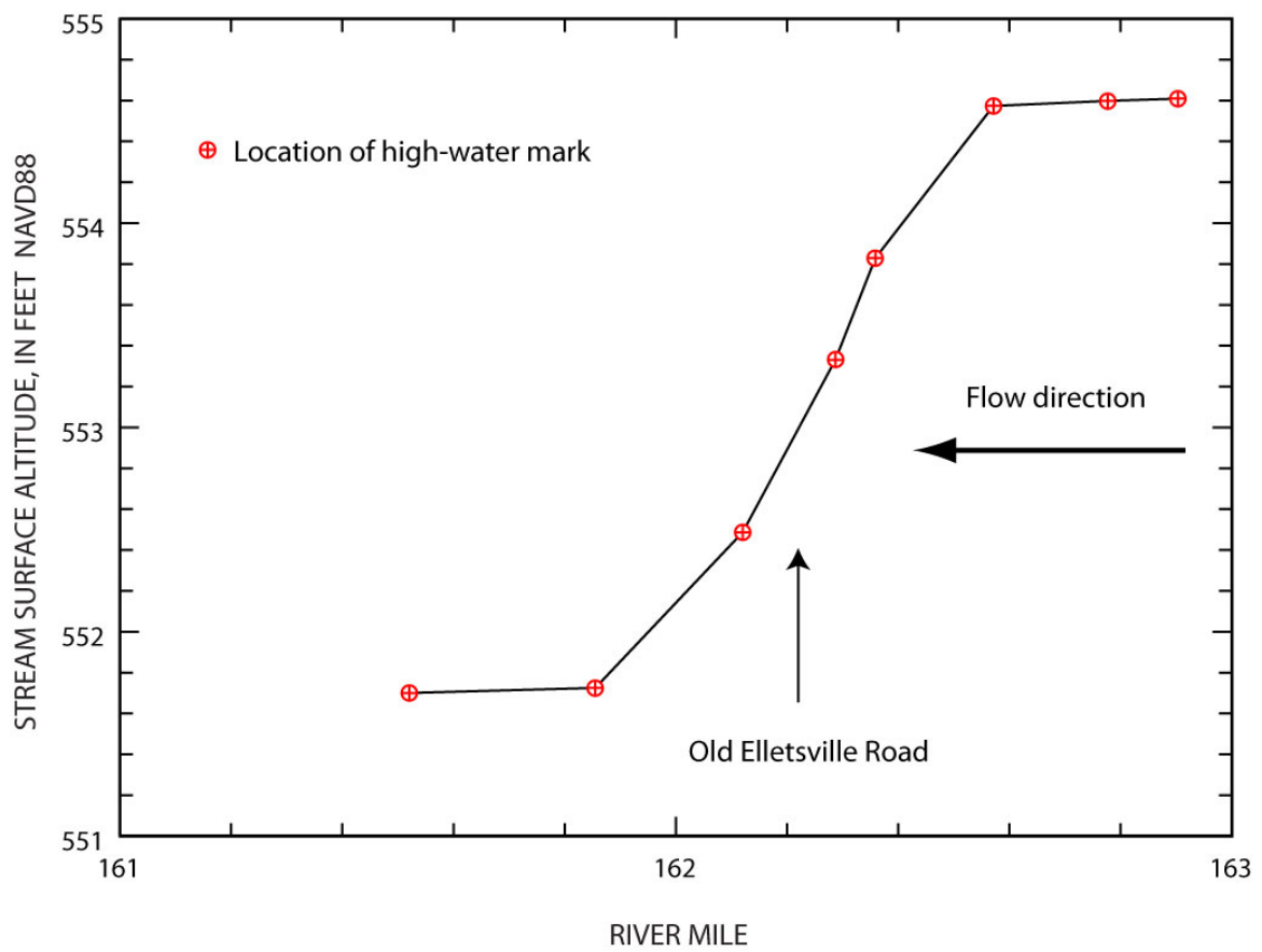
Flood-peak elevation profile, flood of June 7–9, 2008, for White River at Spencer, Indiana.
