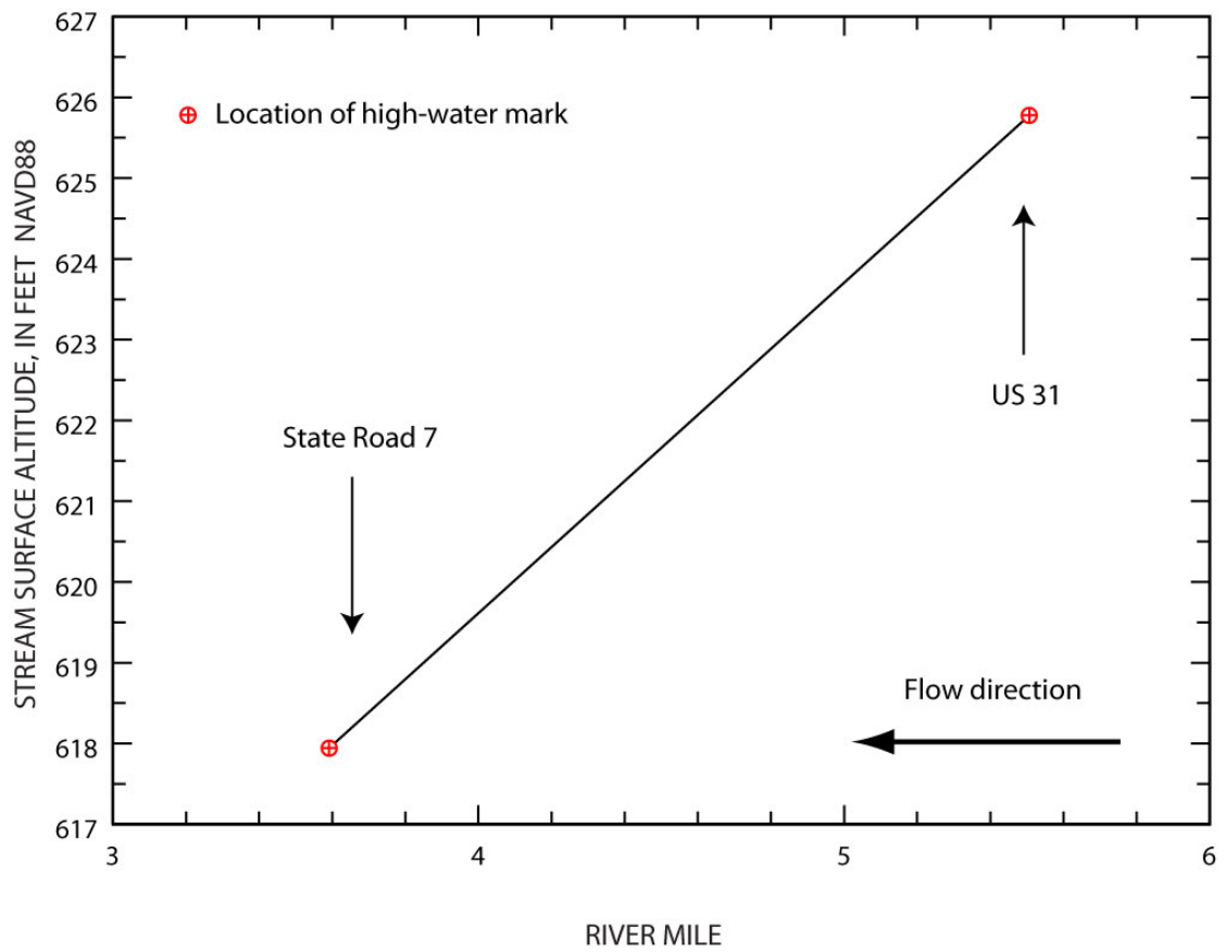
Flood-peak elevation profile, flood of June 7–9, 2008, for Clifty Creek at Columbus, Indiana.
