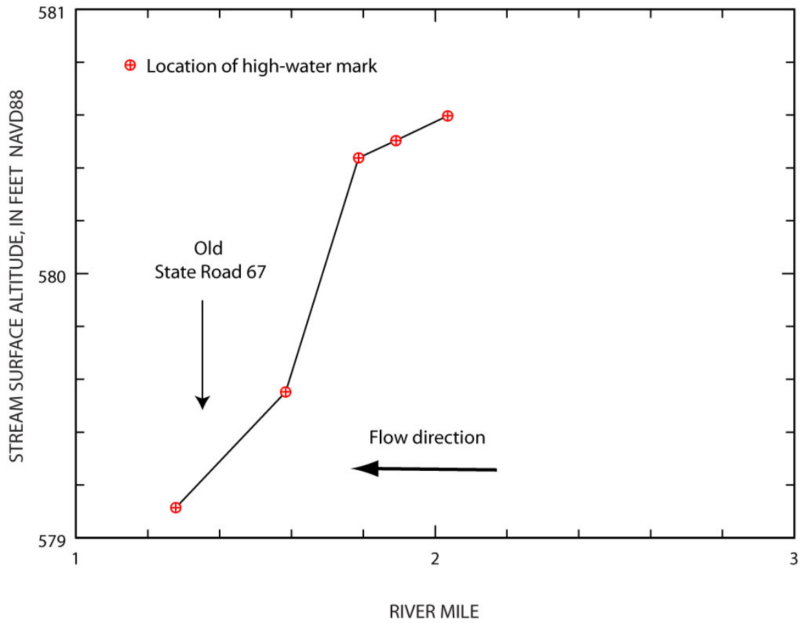
Flood-peak elevation profile, flood of June 7–9, 2008, for an unnamed tributary of Fall Creek at Paragon, Indiana.
