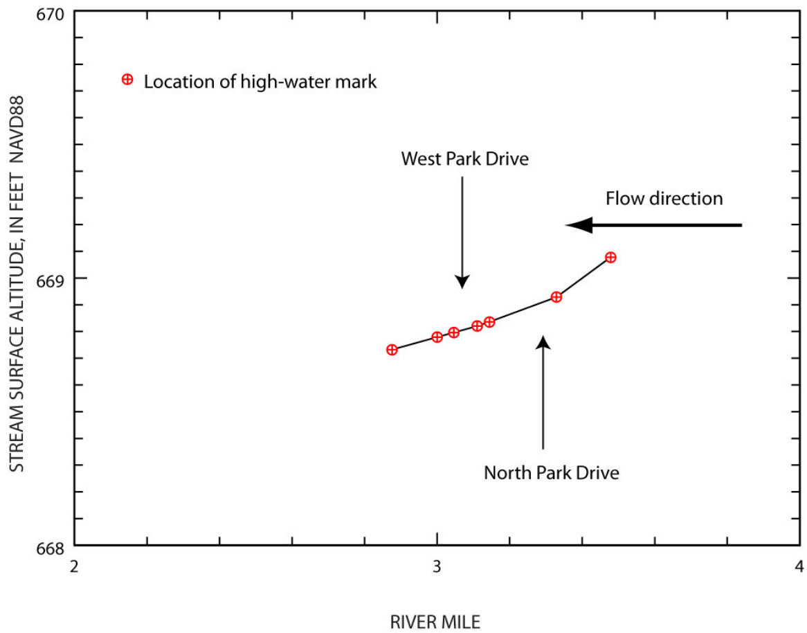
Flood-peak elevation profile, flood of June 7–9, 2008, for East Side Swale at Edinburgh, Indiana.
