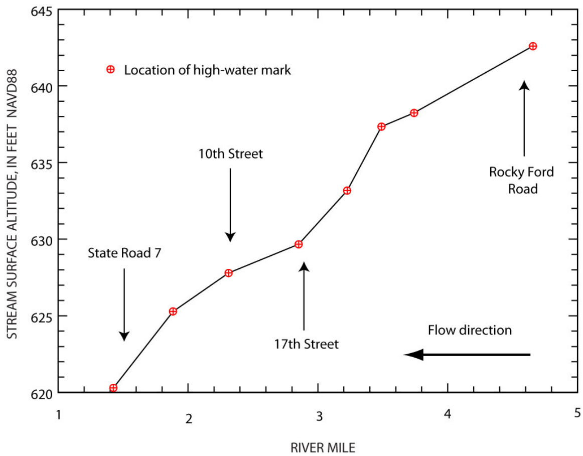
Flood-peak elevation profile, flood of June 7–9, 2008, for Haw Creek at Columbus, Indiana.
