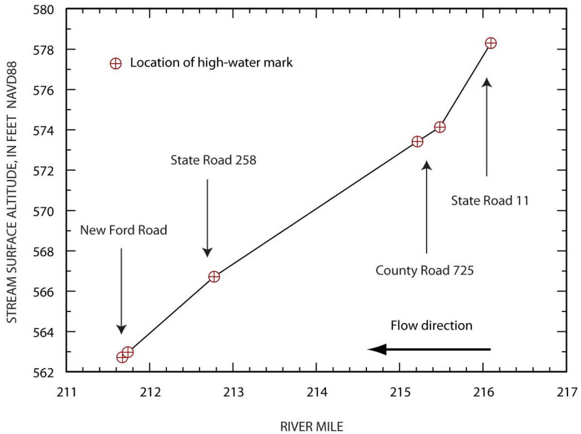
Flood-peak elevation profile, flood of June 7–9, 2008, for East Fork White River at Seymour, Indiana.
