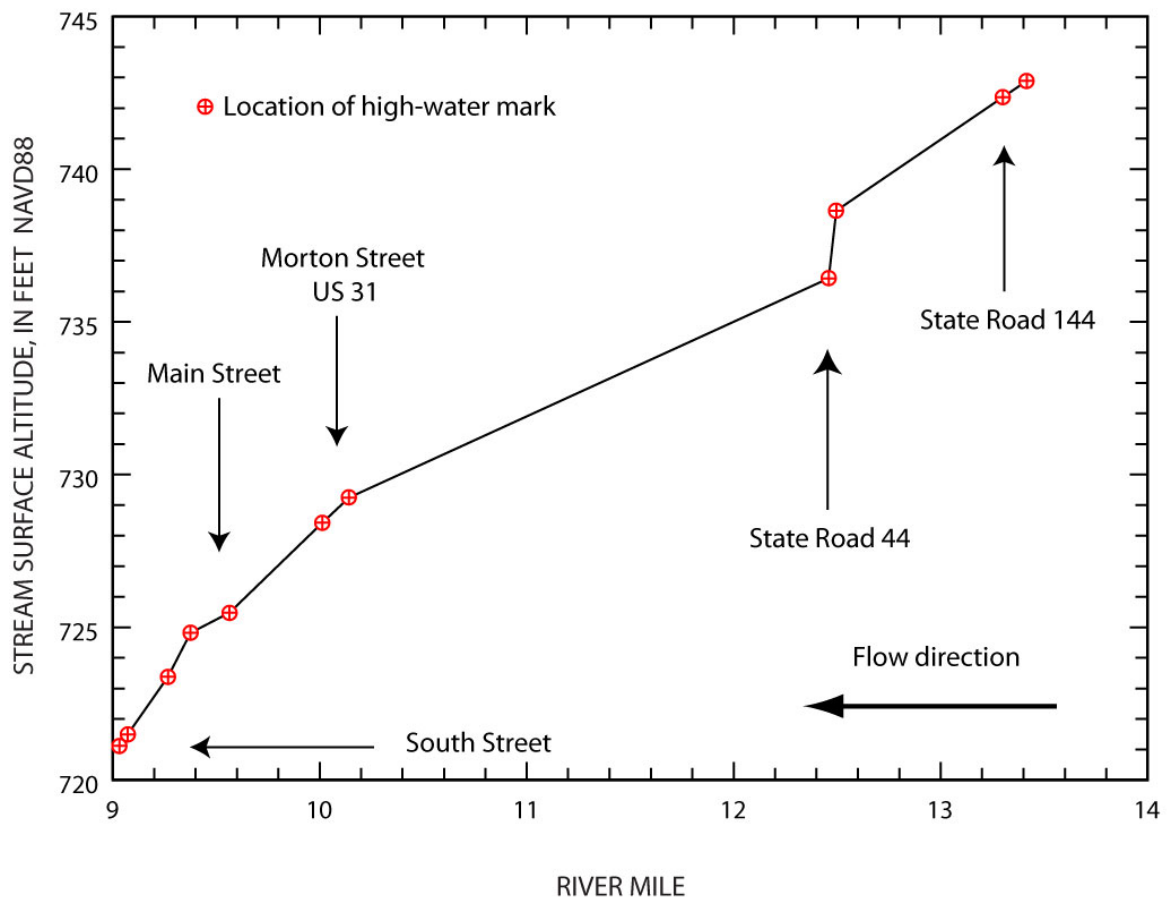
Flood-peak elevation profile, flood of June 7–9, 2008, for Youngs Creek at Franklin, Indiana
