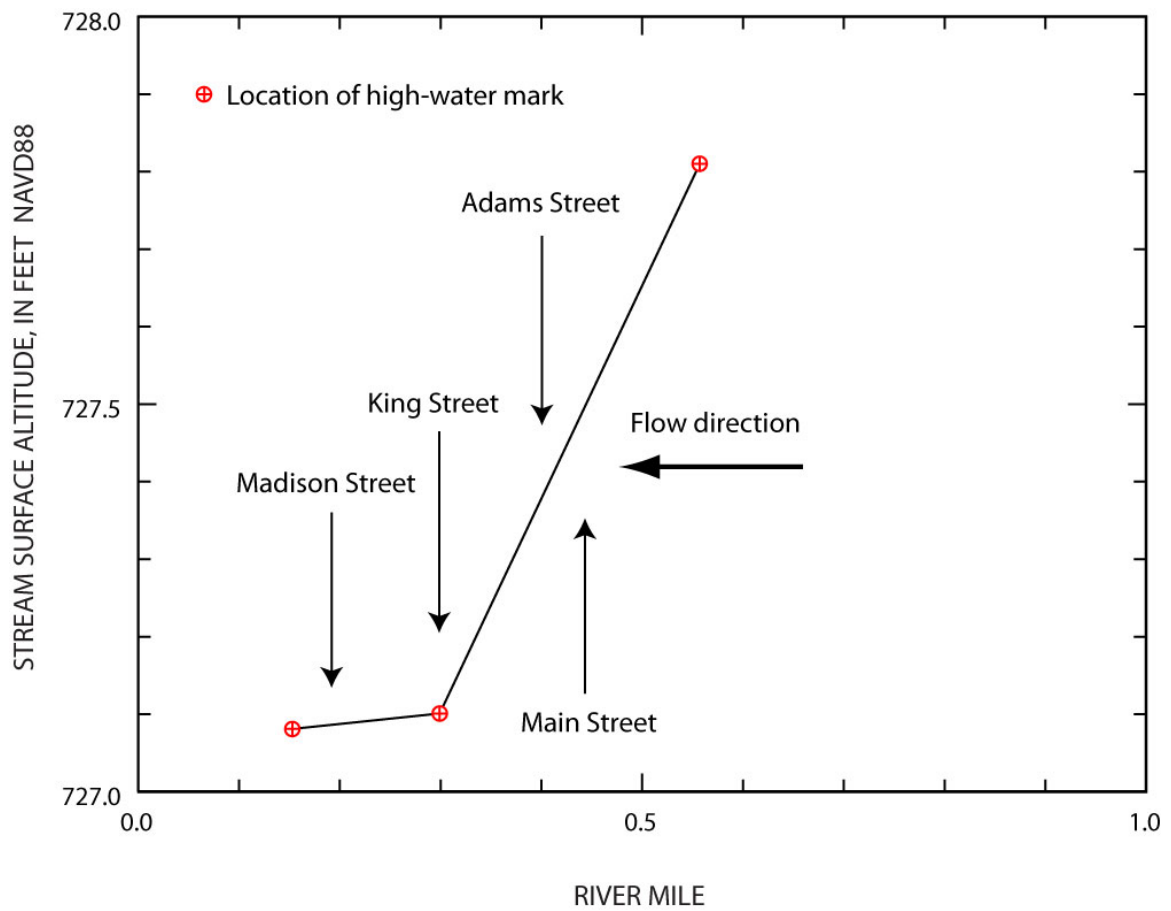
Flood-peak elevation profile, flood of June 7–9, 2008, for an unnamed tributary of Youngs Creek at Franklin, Indiana.
