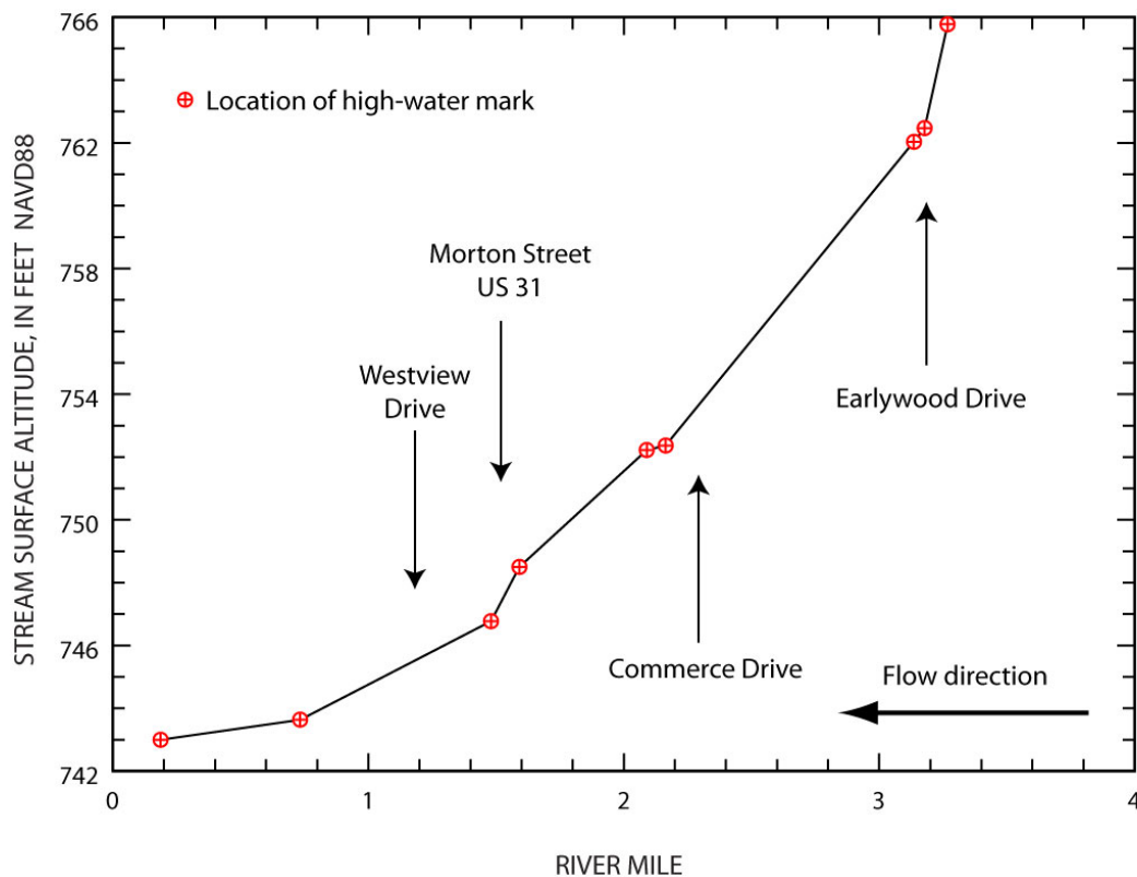
Flood-peak elevation profile, flood of June 7–9, 2008, for Canary Ditch at Franklin, Indiana.
