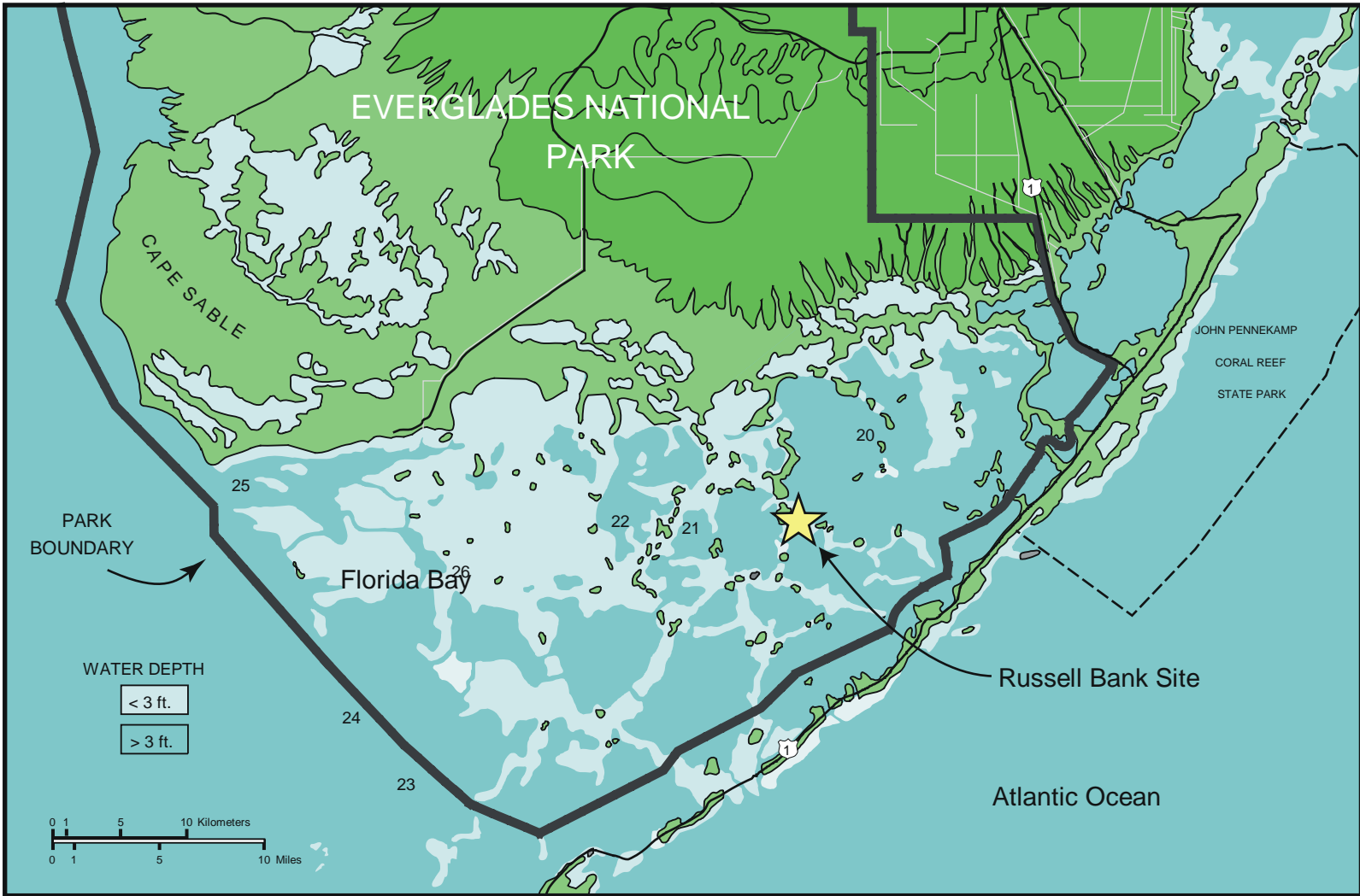
Figure 1. Location of Russell Bank (N25 03.831', W80 37.486'), cores 19A, 19B, and 19C.
