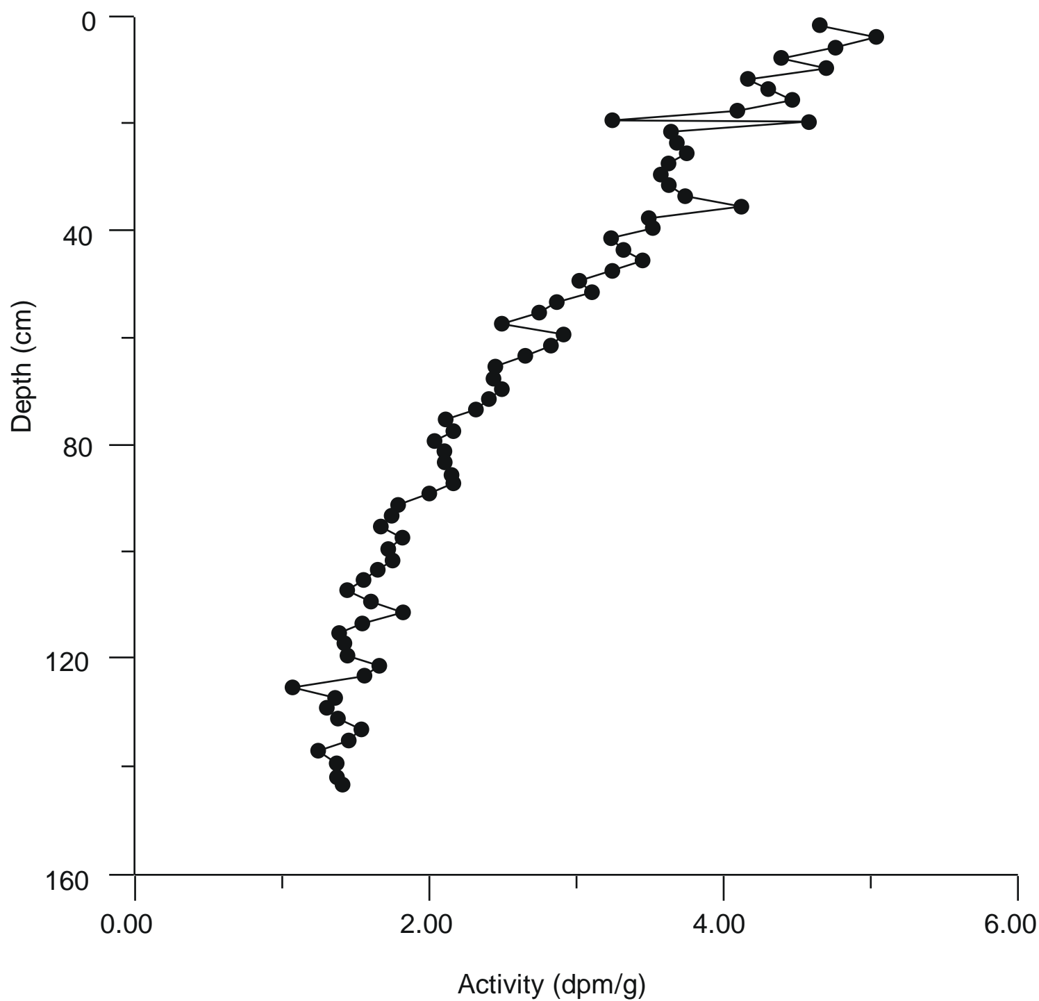
Figure 9: \text{Pb}^{210} activity in dpm/g for core 19B
