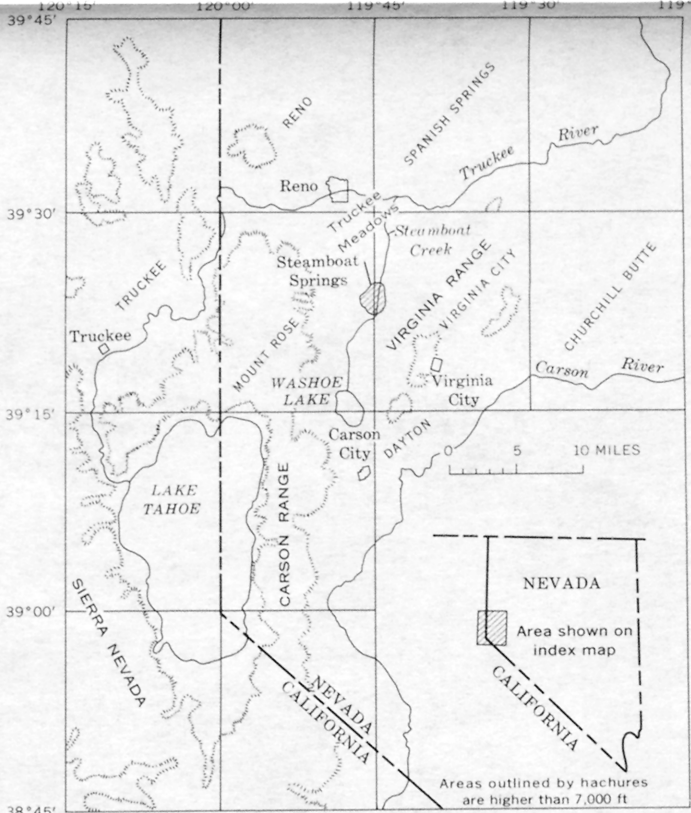
LOCATION OF STEAMBOAT SPRINGS THERMAL AREA, WASHOE COUNTY, NEVADA
