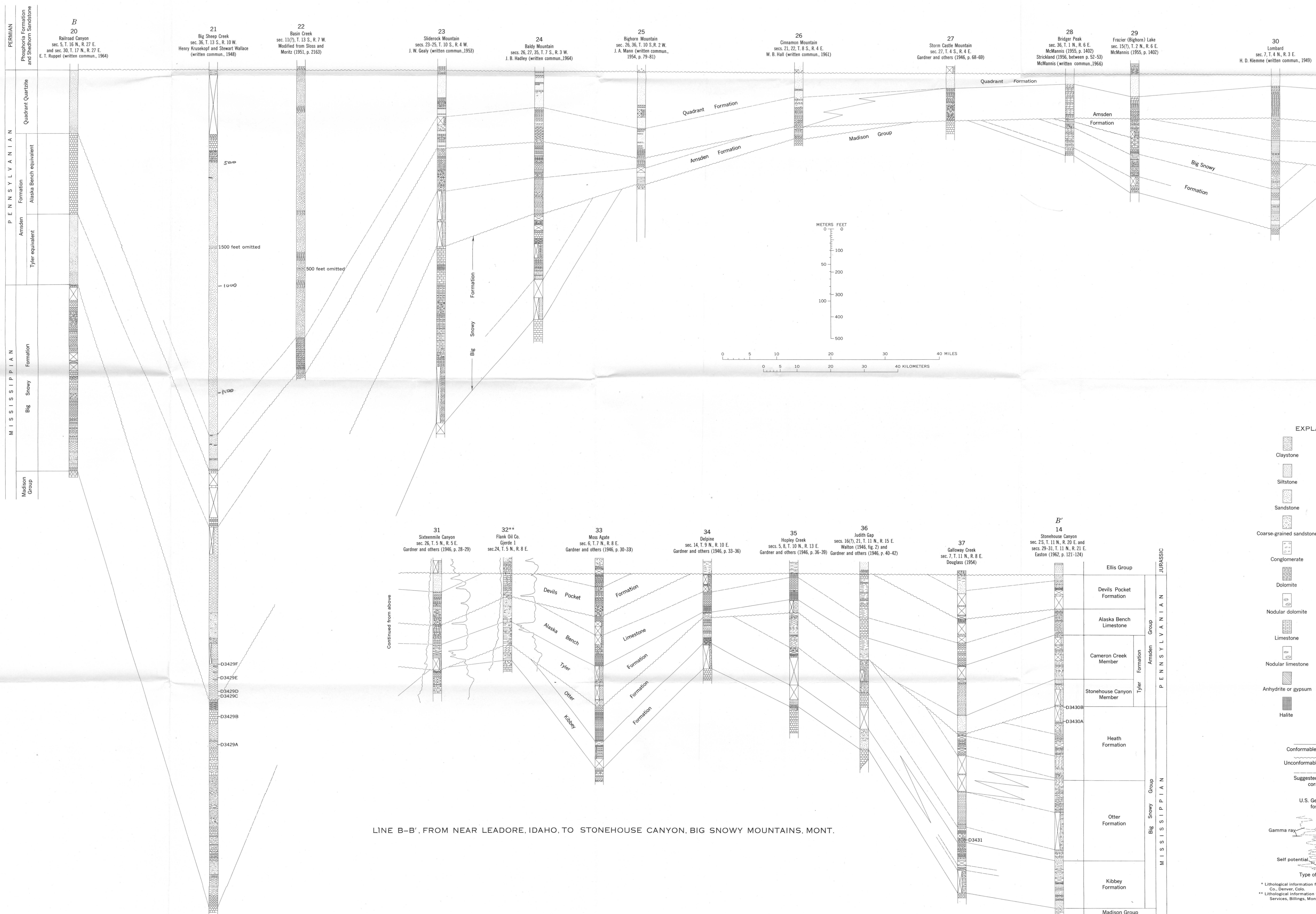
COLUMNAR SECTIONS SHOWING CORRELATION OF BIG SNOWY AND AMSDEN GROUPS IN CENTRAL AND SOUTHERN MONTANA
