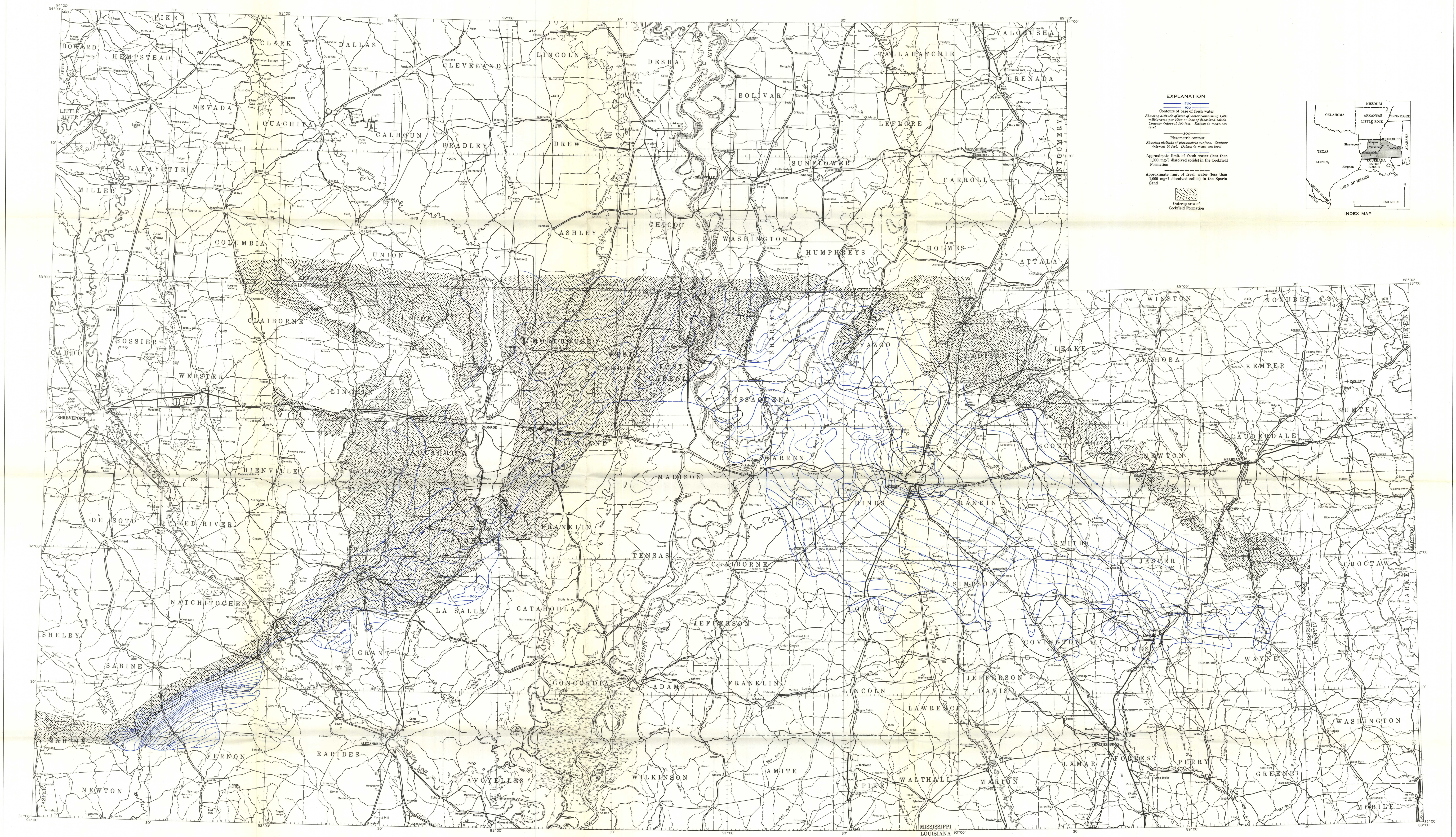
MAP SHOWING THE PIEZOMETRIC SURFACE AND THE ALTITUDE OF THE BASE OF FRESH GROUND WATER IN THE COCKFIELD FORMATION IN LOUISIANA AND MISSISSIPPI
