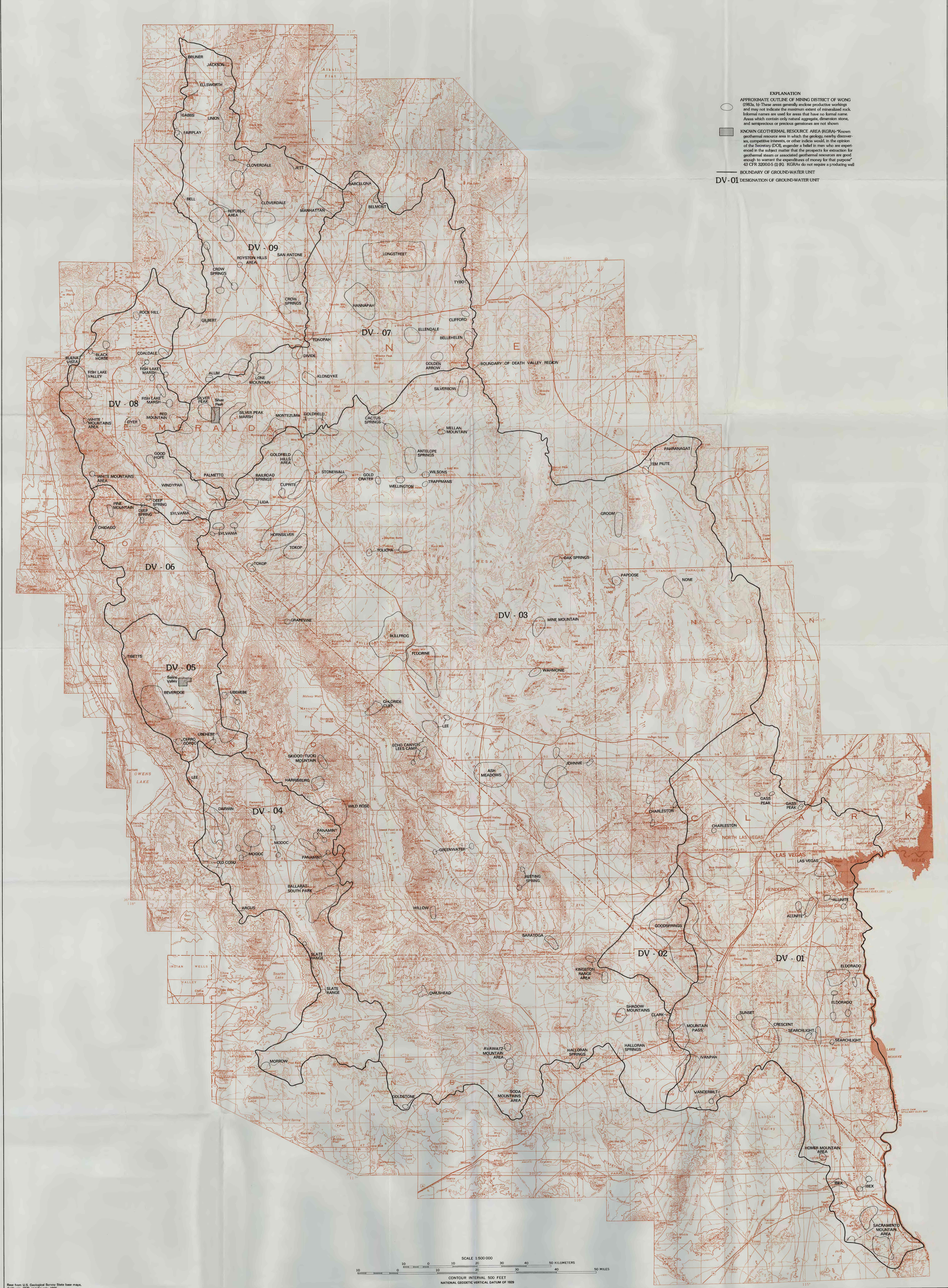
MAP SHOWING PRINCIPAL MINING DISTRICTS, DEATH VALLEY REGION, NEVADA AND CALIFORNIA
