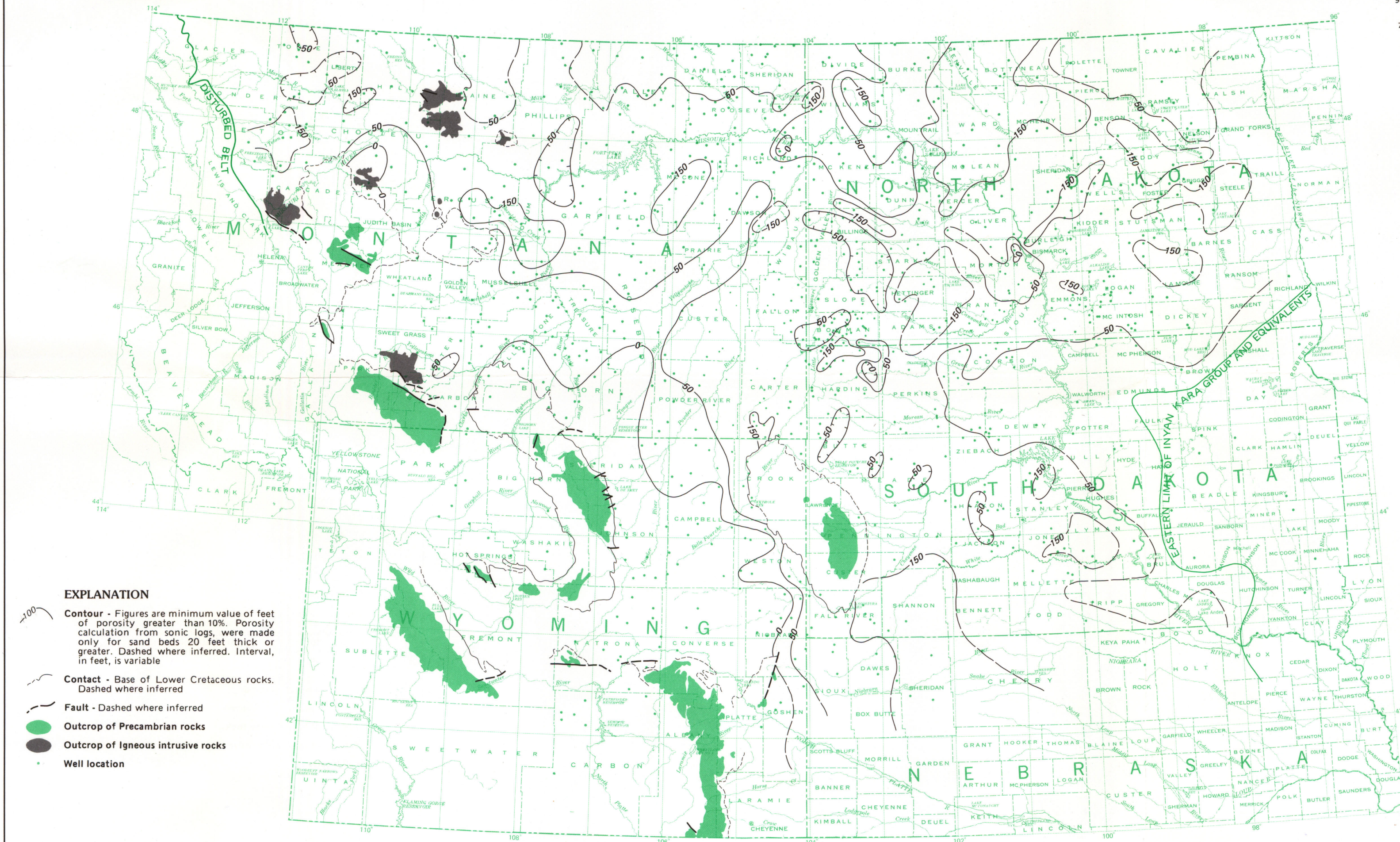
C. MINIMAL FEET OF POROSITY OF INYAN KARA GROUP AND EQUIVALENTS, LOWER CRETACEOUS.
