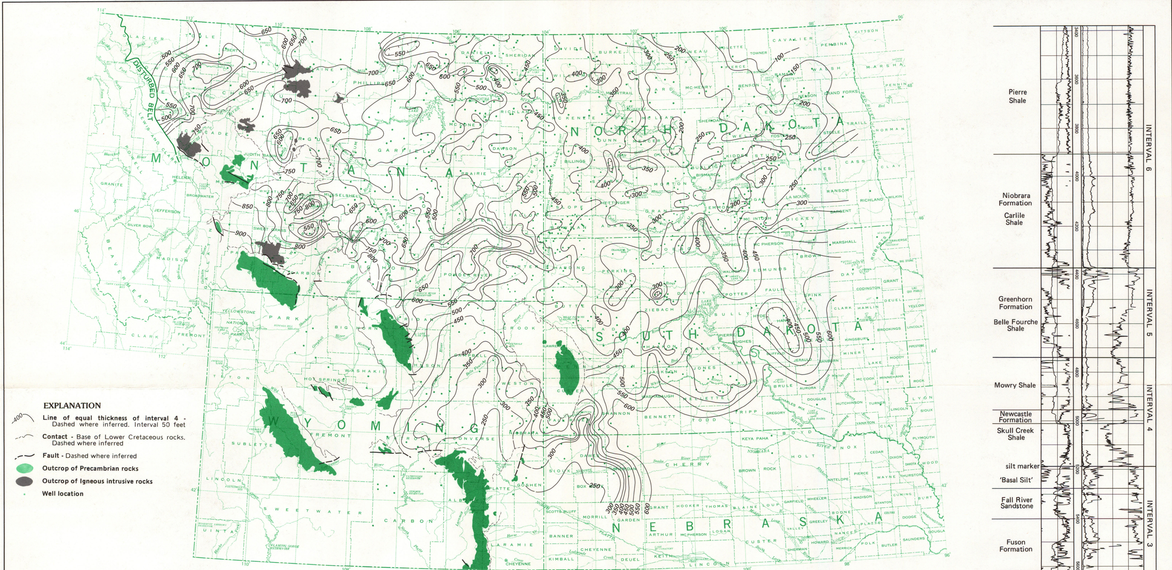
A. ISOPACH OF INTERVAL 4, SILT MARKER BED AND UPPER PART OF THE SKULL CREEK SHALE, NEWCASTLE SANDSTONE, MOWRY SHALE AND EQUIVALENT ROCKS, LOWER CRETACEOUS.
