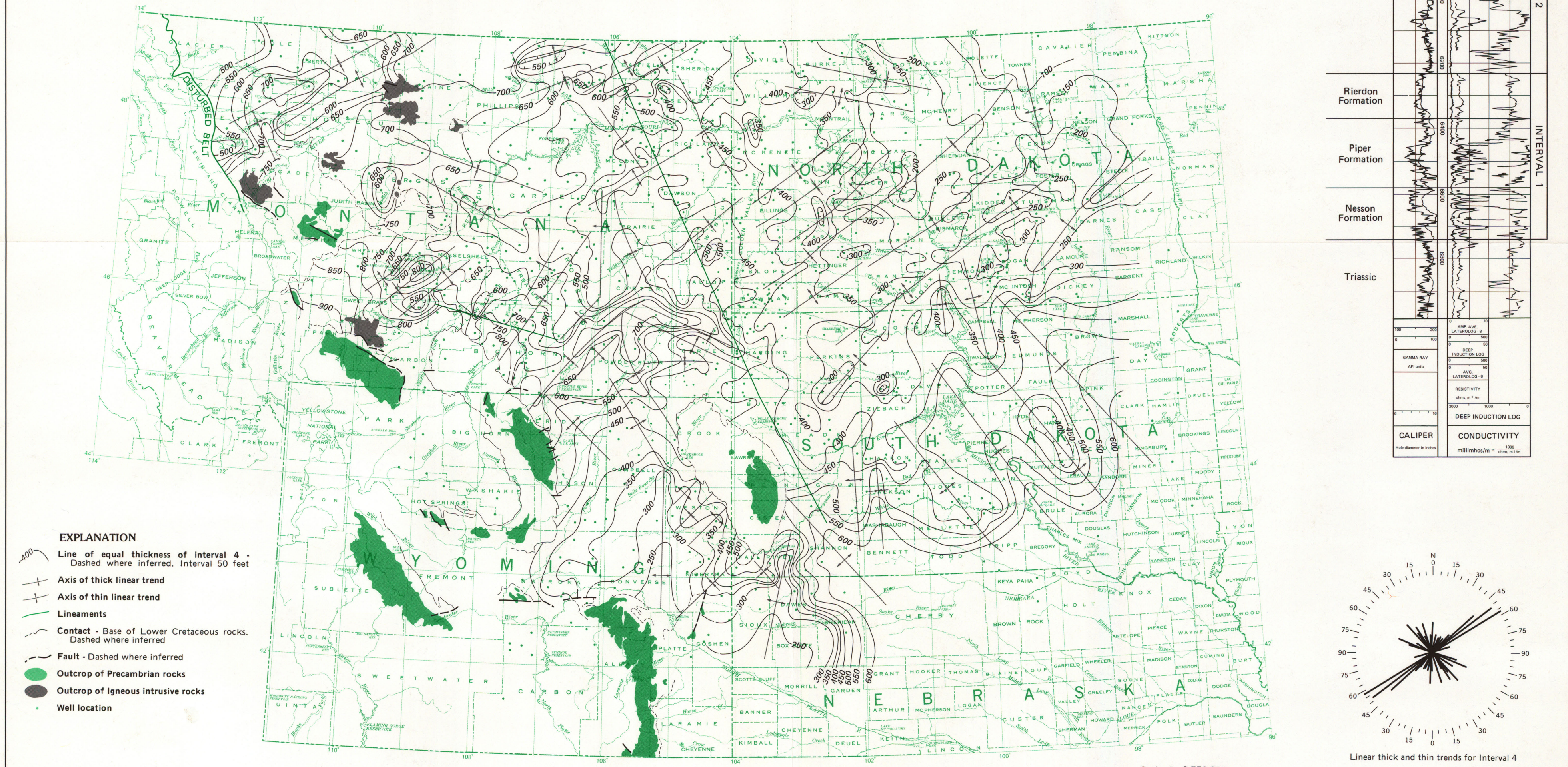
B. ISOPACH AND LINEAR TREND OF INTERVAL 4.
